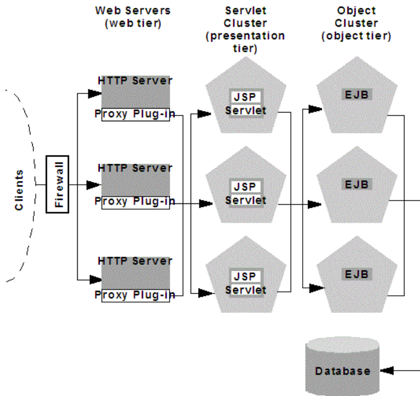
Figure 9-5 Multitier Proxy Architecture
