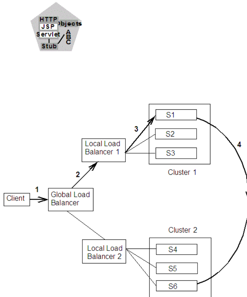
Figure 6-6 MAN Replication
