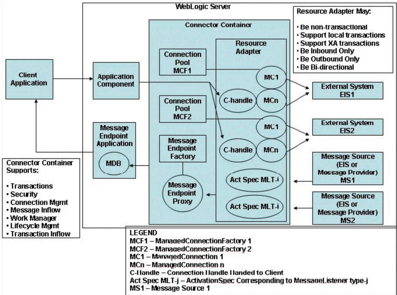
Figure 2-1 Connector Architecture Overview
