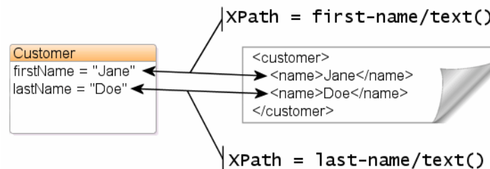
Figure 4-2 XML Direct Mapping to Individual Text Nodes
