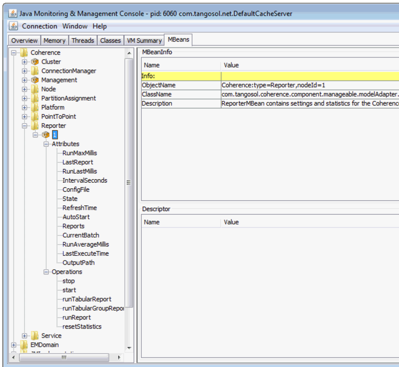
Figure 4-1 ReporterMBean MBean in JConsole
