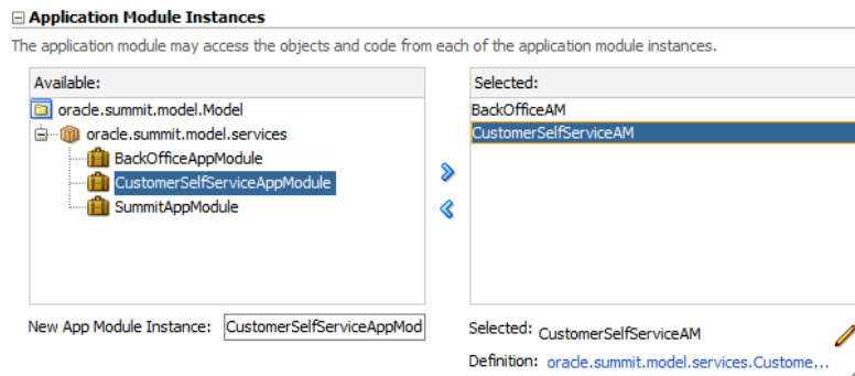
Figure 13-14 Data Model Displays Added Application Module Instances
