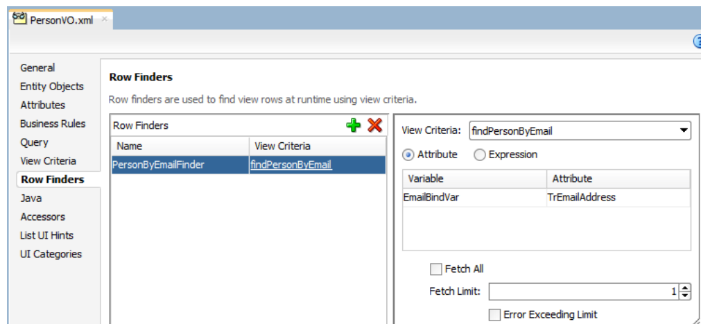
Figure 6-10 View Object Overview Editor with Row Finder
