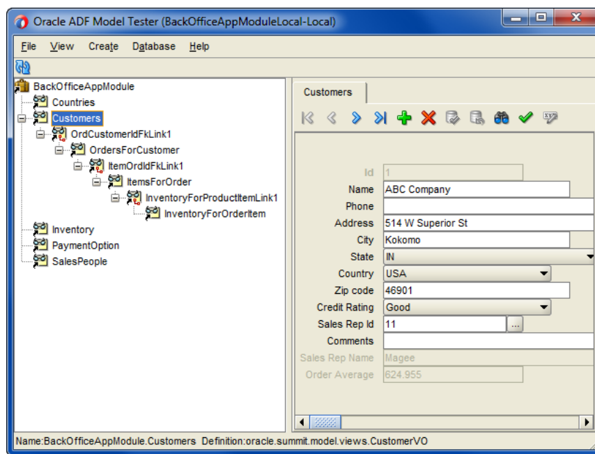
Figure 8-6 Testing the Data Model in the Oracle ADF Model Tester
