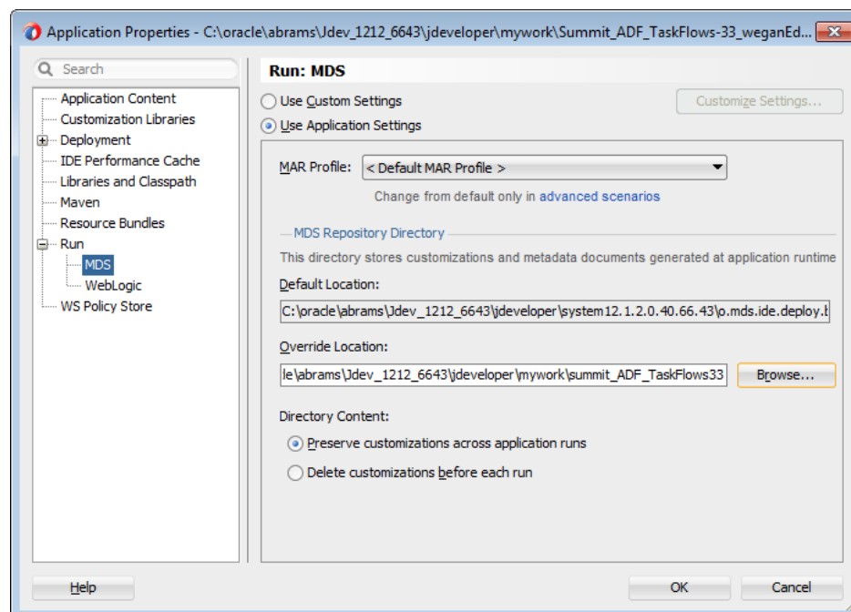
Figure 55-2 Setting the Run MDS Options
