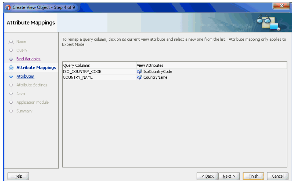
Figure 5-26 Create View Object Wizard, Attribute Mappings Page
