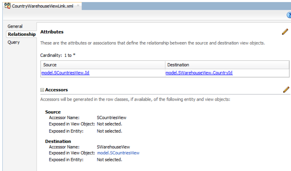
Figure 43-27 Sample View Link Between Country and Warehouse
