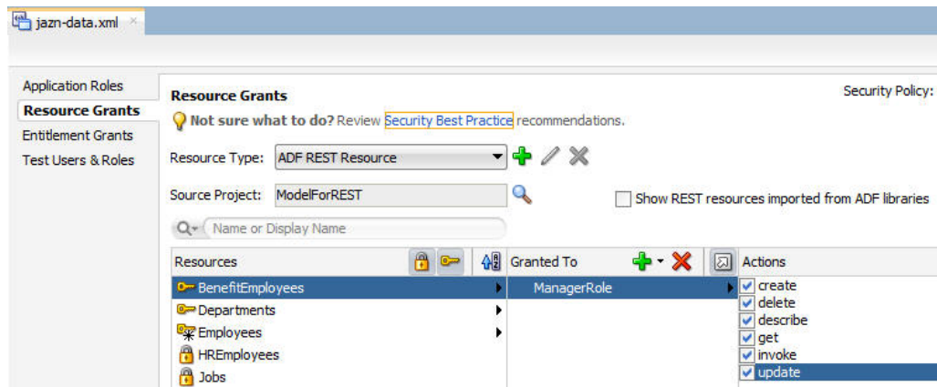
Figure 16-21 Creating a Grant for an ADF REST Resource
