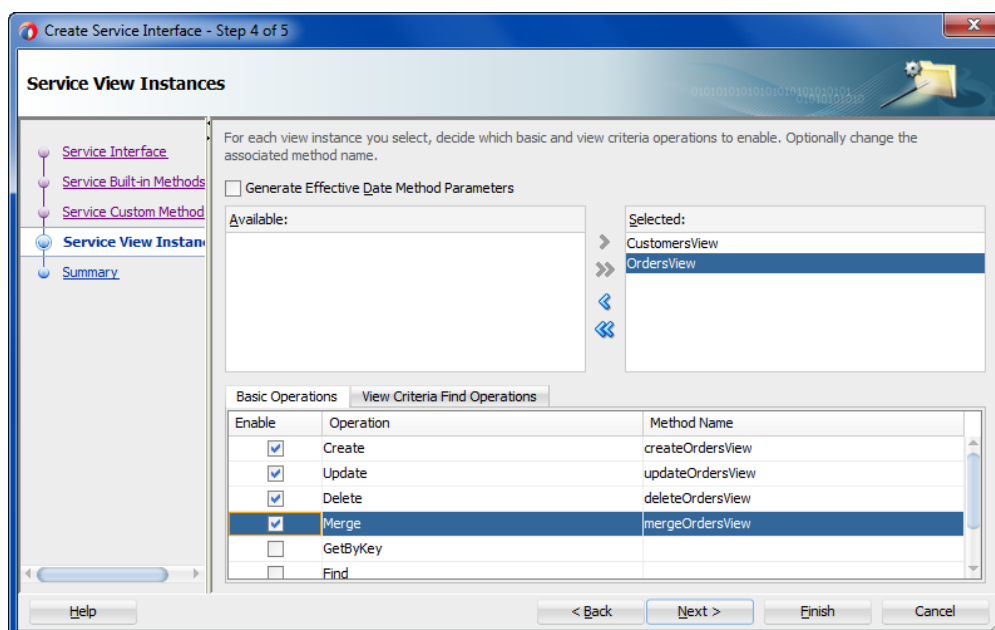
Figure 15-1 View Instances and CRUD Operation Selection
