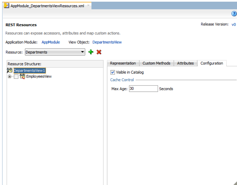
Figure 16-19 Cache Maximum in Seconds Set on the Root of the REST Resource
