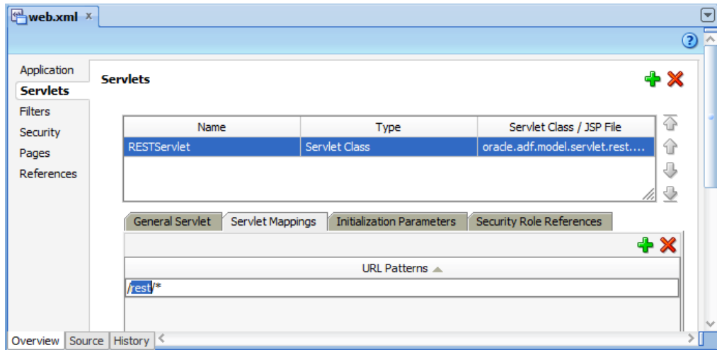
Figure 16-26 Editing the URL Pattern for the REST Servlet Mapping
