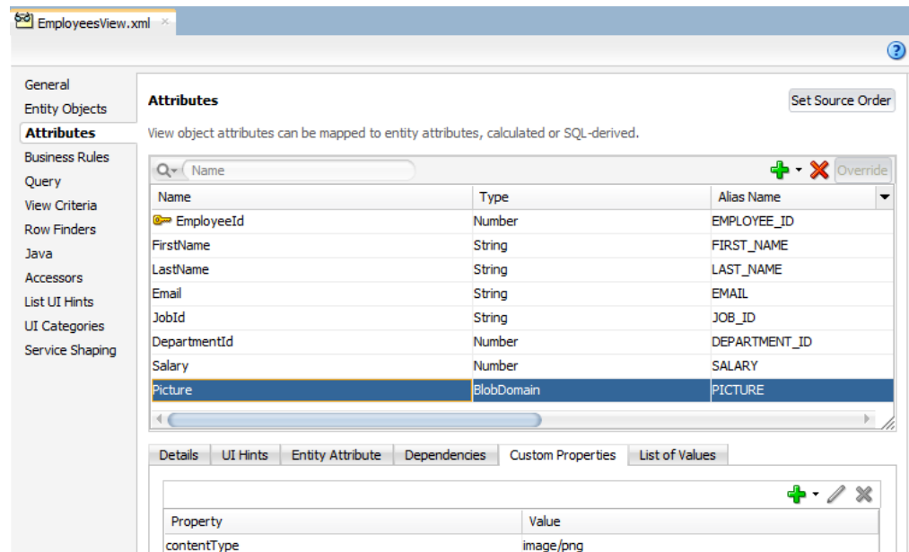
Figure 16-12 Custom Content Type Configured for LOB Attributes
