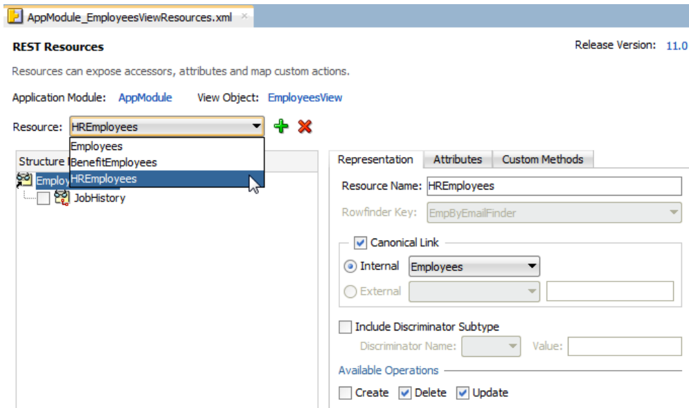
Figure 16-7 Resource List Supports Multiple Resource in the REST Resource Definition
