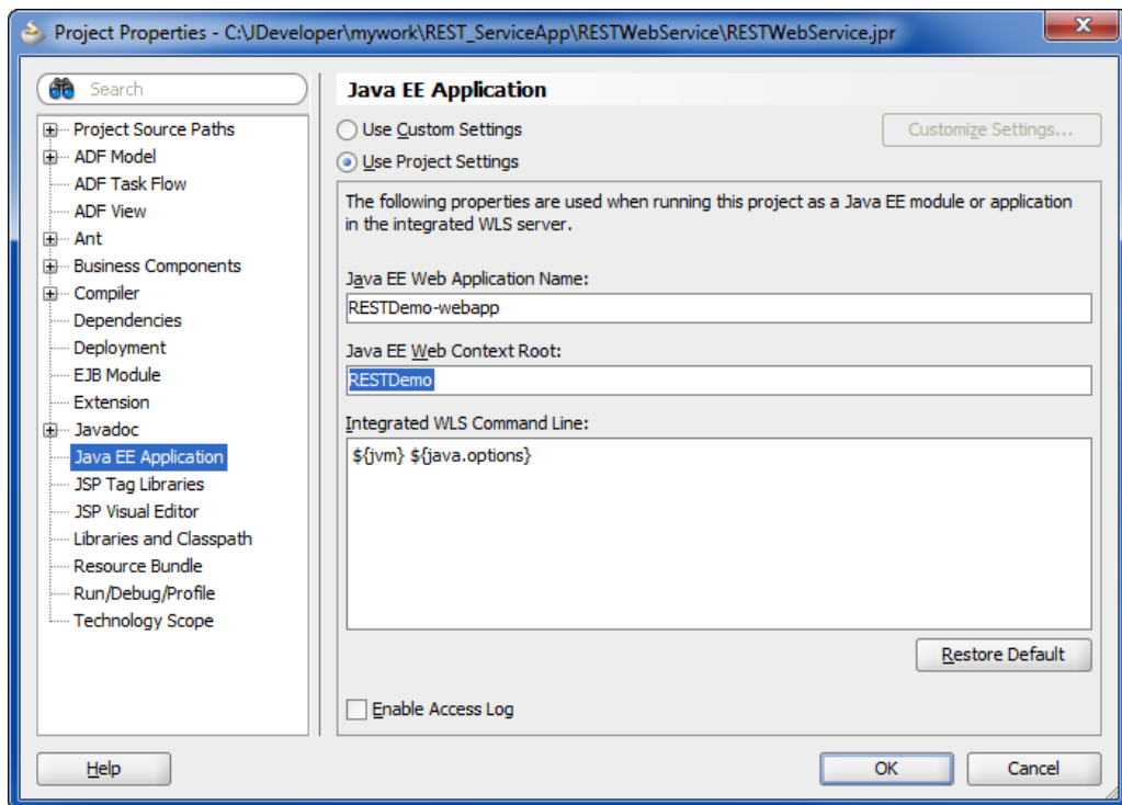
Figure 16-27 Editing the Default Context Root on the RESTWebService Project
