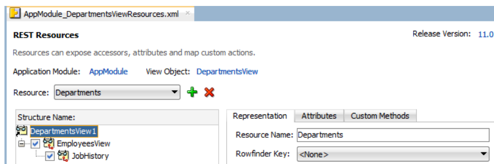
Figure 16-11 REST Resource Editor Displays Version
