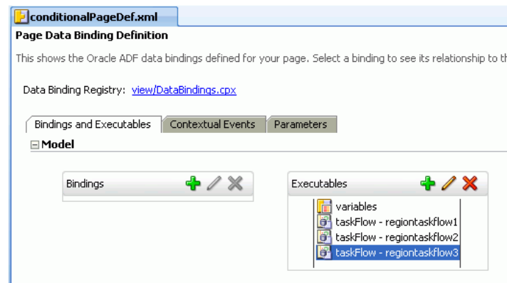
Figure 26-8 Task Flow Bindings for ADF Region Configured for Activation
