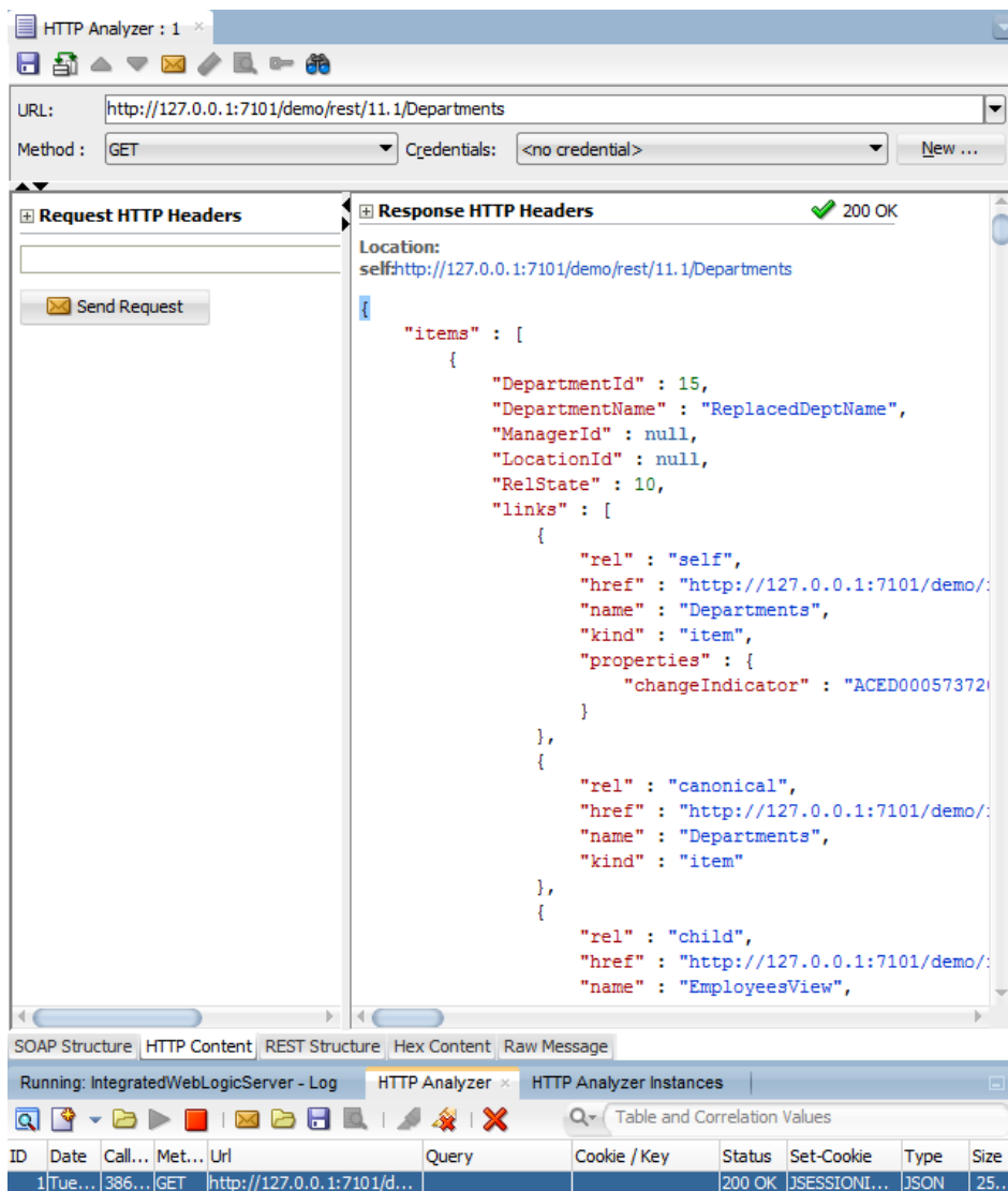
Figure 16-28 Using the HTTP Analyzer to Make a GET REST Request
