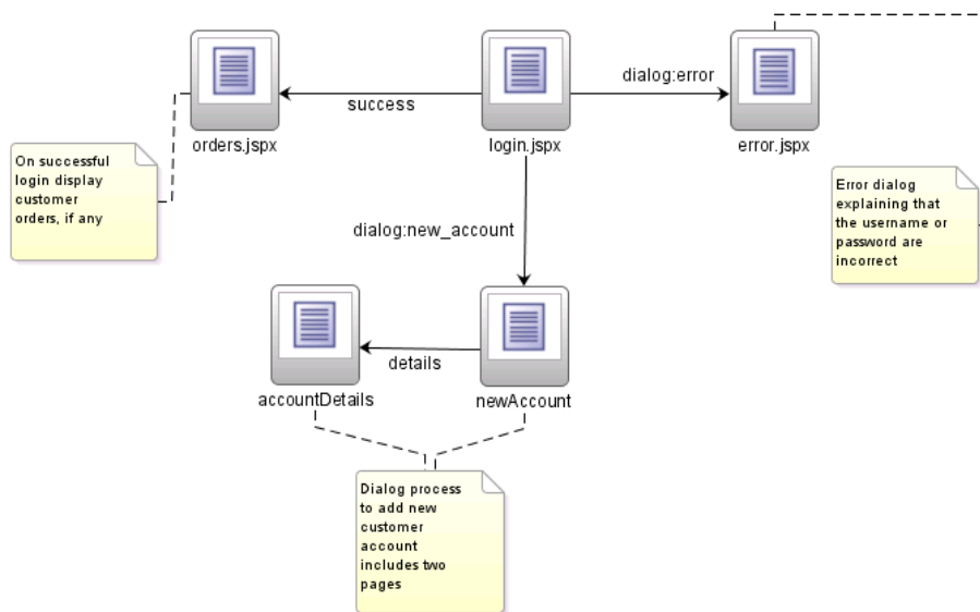
Figure 28-2 Page Flow of an External Dialog Sample Application
