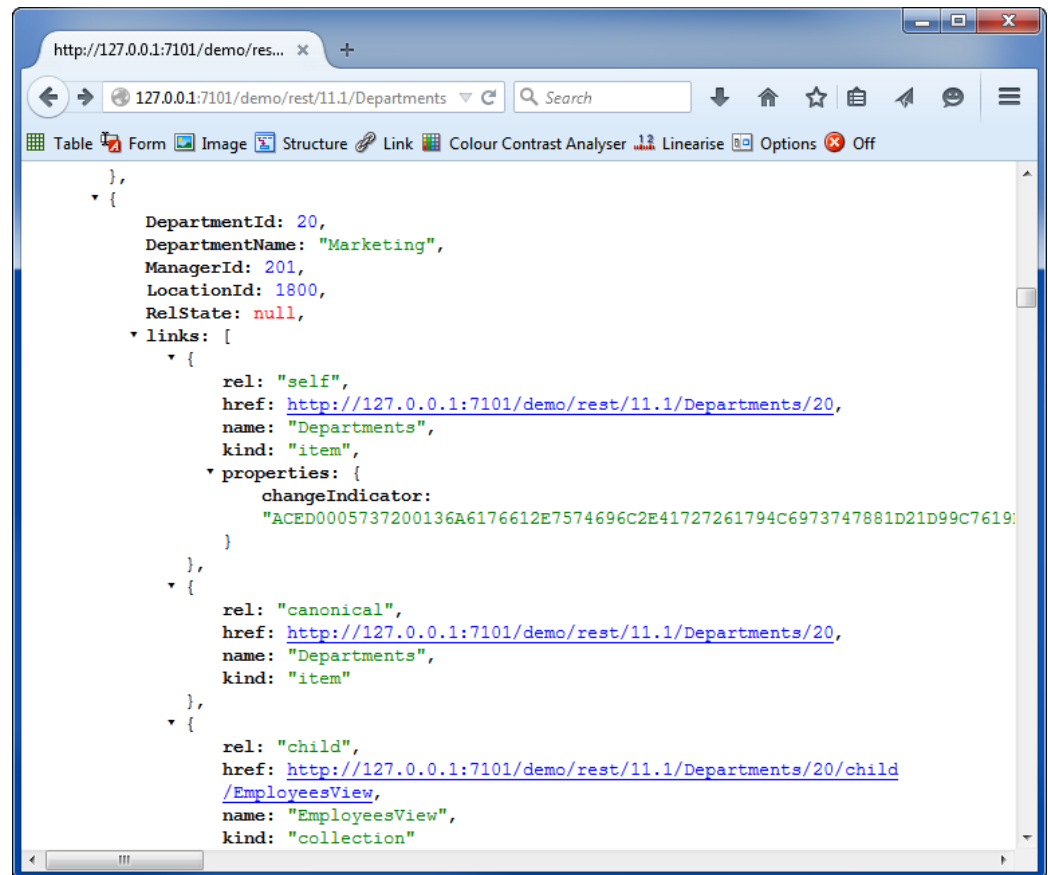
Figure 16-24 Using the Browser to Make a GET REST Request
