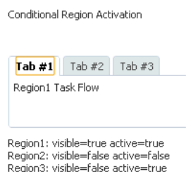
Figure 26-11 Conditional Activation of ADF Regions
