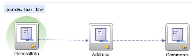
Figure 27-9 Task Flow Configured to Render as a Train
