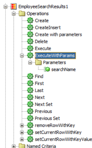
Figure 43-20 ExecuteWithParams Operation for Hierarchy Viewer Search Example
