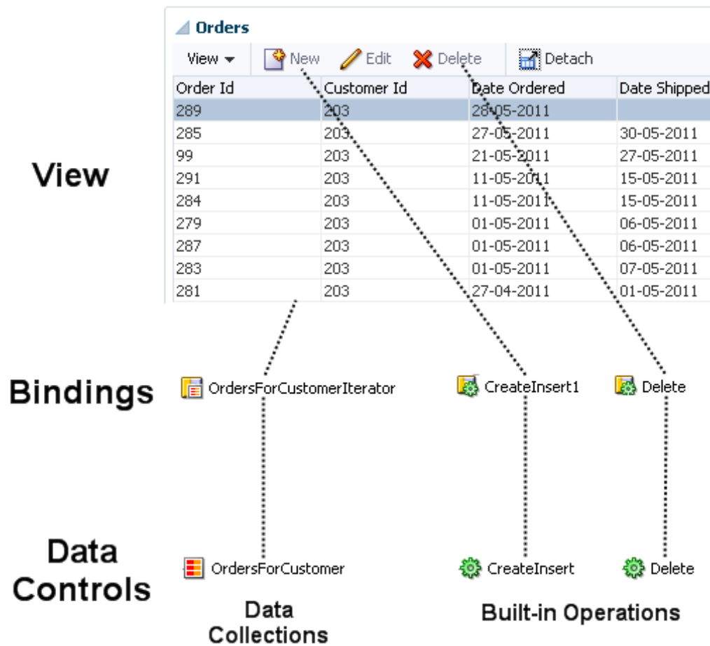
Figure 18-2 Bindings Connect UI Components to Data Controls
