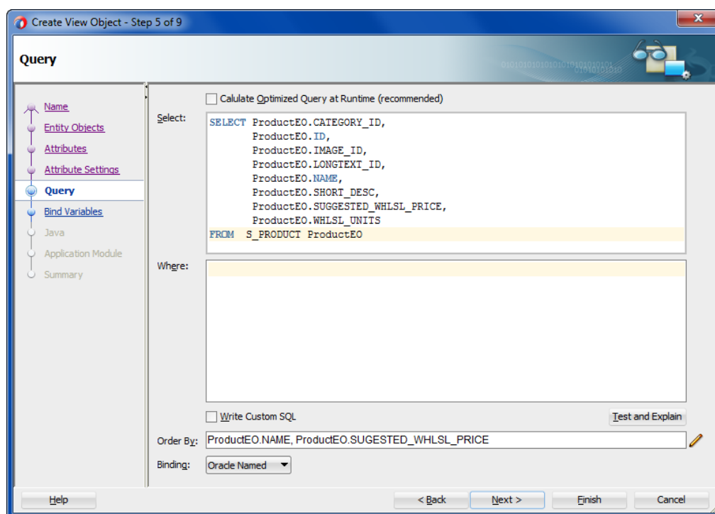
Figure 5-6 Create View Object Wizard, Query Page
