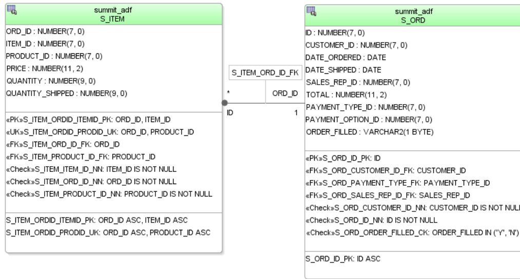
Figure 4-4 S_ITEM and S_ORD Tables Related by Foreign Key
