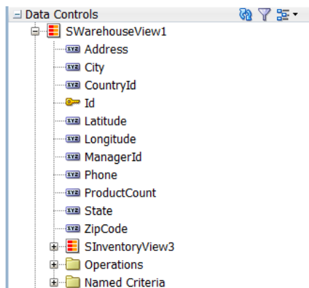
Figure 41-8 Data Collection for Warehouse Location and Product Count
