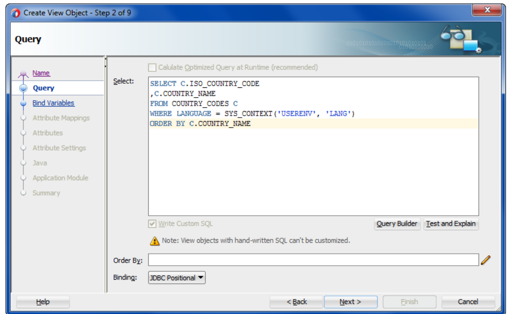
Figure 5-24 Create View Object Wizard, Query Page
