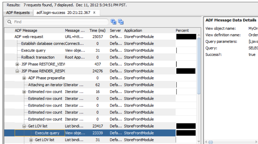
Figure 48-9 Oracle Diagnostic Log Analyzer Displays ADF Event Messages with ADF Data
