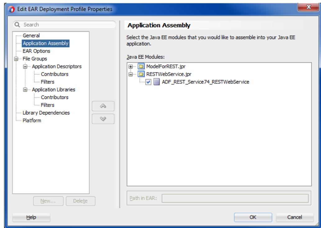
Figure 16-25 Adding a Deployment Dependency on RESTWebService Project
