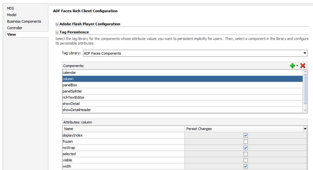
Figure 52-3 Overview Editor for the adf-config.xml File
