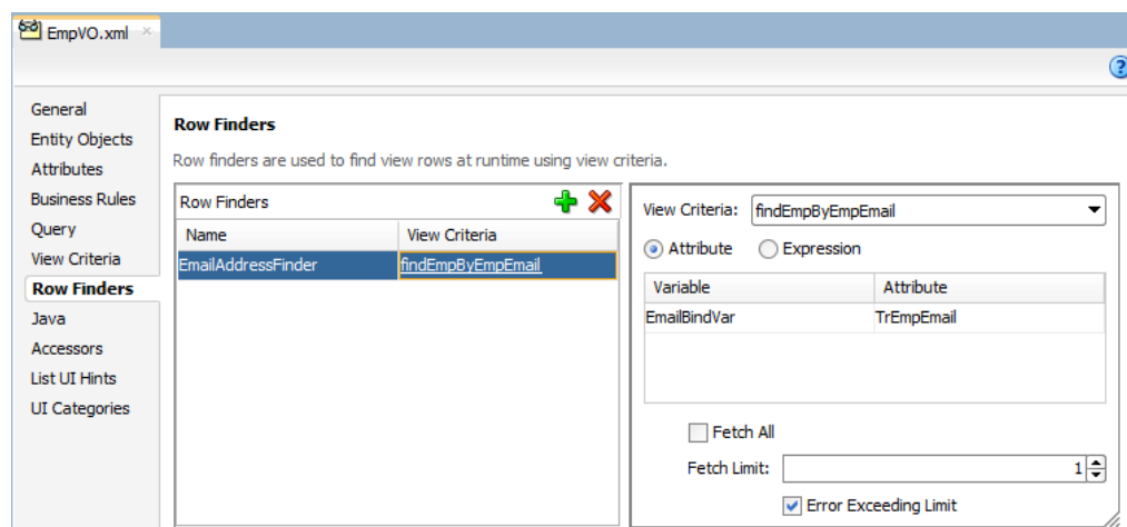
Figure 5-37 View Object Overview Editor with Row Finder
