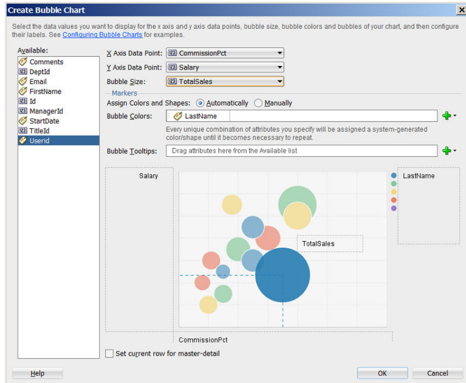
Figure 38-18 Create Bubble Chart Dialog
