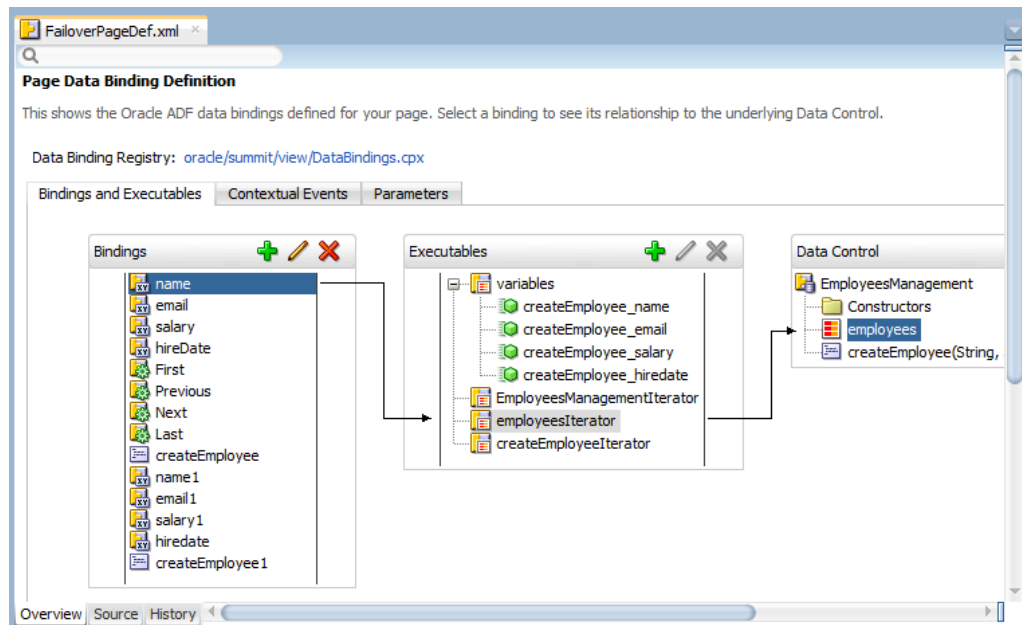
Figure 49-1 Page Data Binding Definition Overview Tab
