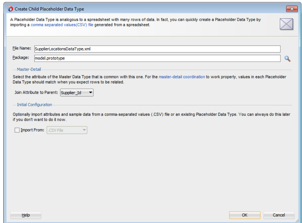
Figure 20-8 Create Child Placeholder Data Type Dialog
