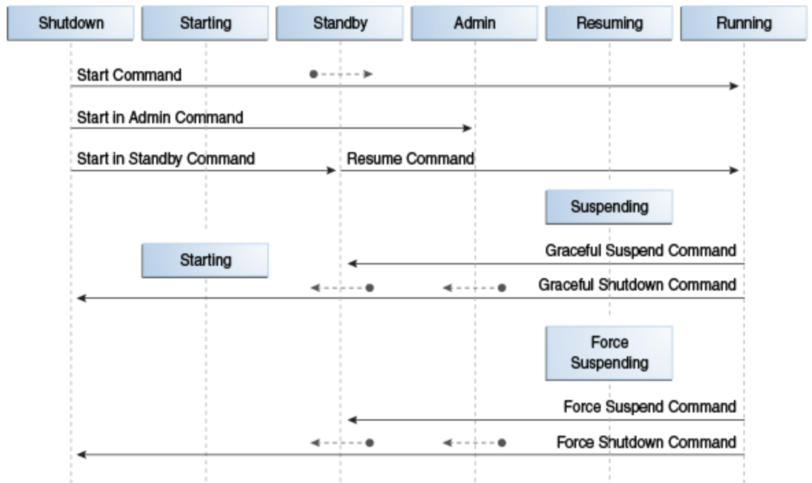
Figure 5-1 State Transitions for Server Life Cycle Commands
