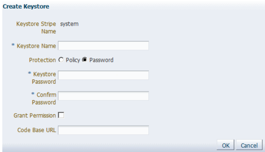
Figure 30-1 Create Keystore
