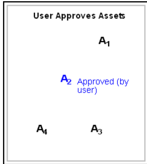
Figure 17-20 User-Approved Asset
