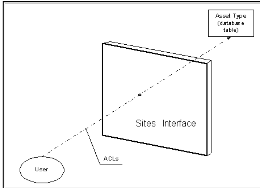
Figure 2-2 User ACLs
