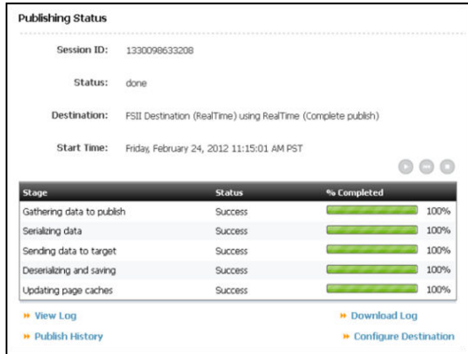
Figure 15-7 Publishing Status
