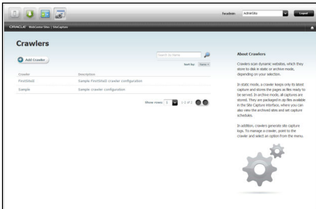
Figure 31-1 Crawlers Page
