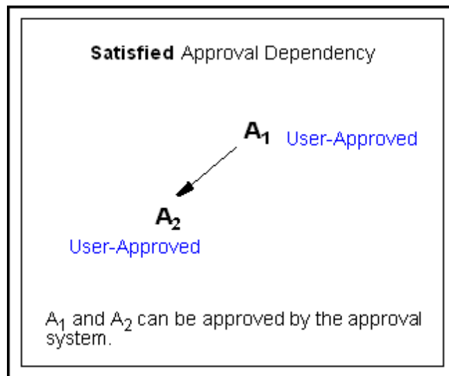
Figure 17-8 Approval Dependencies
