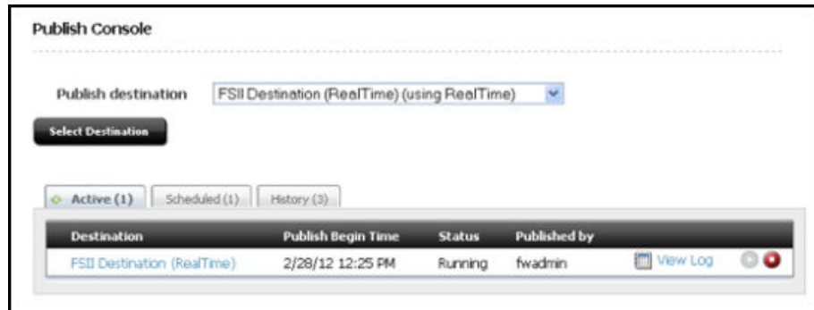
Figure 15-6 Publish Console
