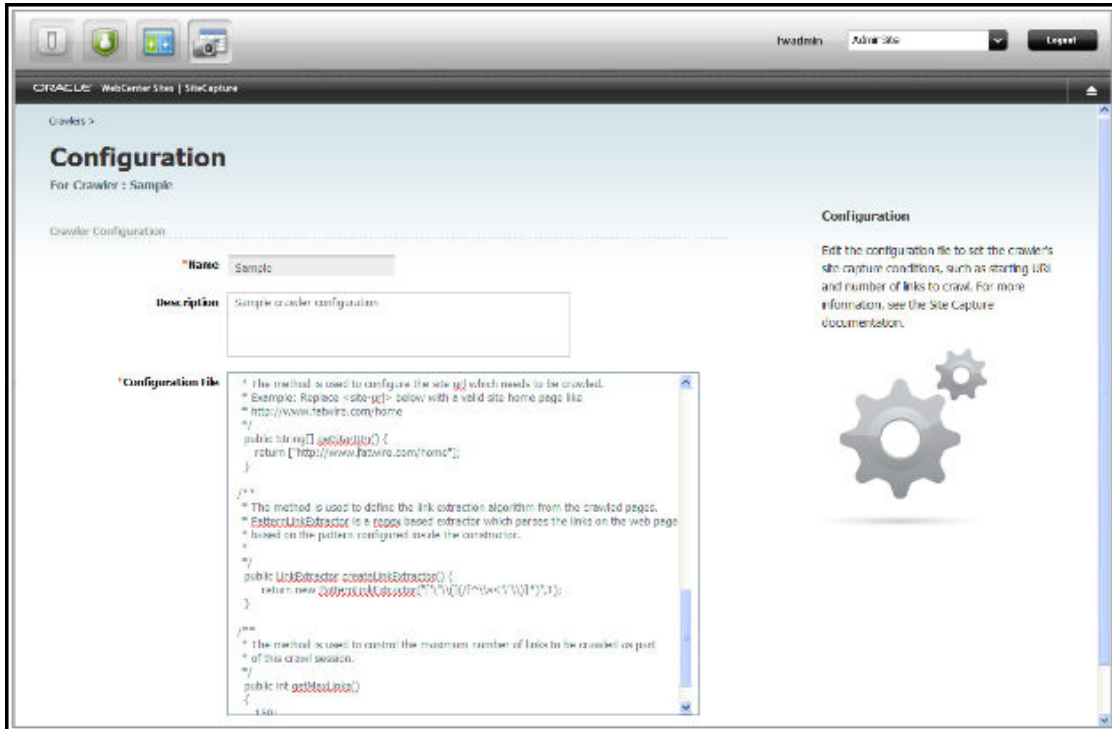
Figure 31-2 Configuration Page
