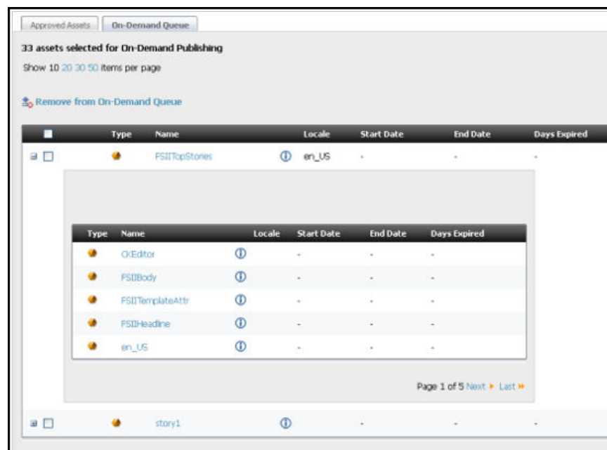
Figure 39-5 On-Demand Tab
