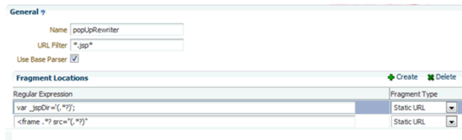
Figure 19-29 popupRewriter
