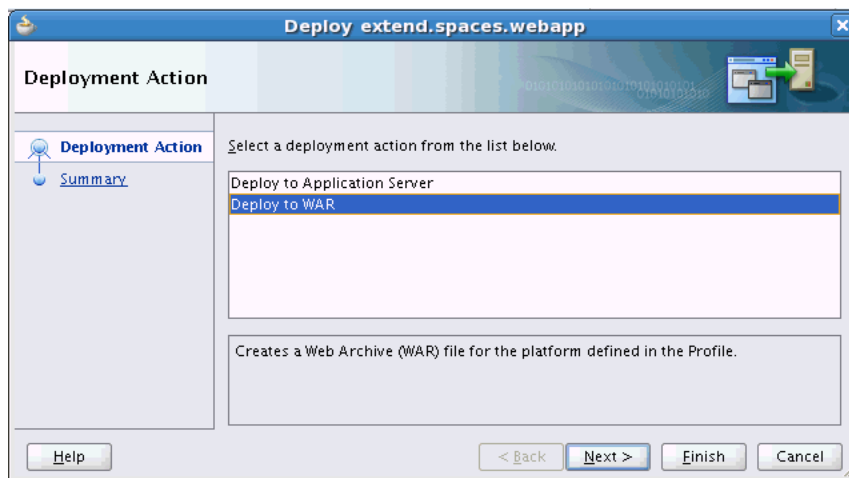
Figure 20-20 Deployment Actions
