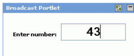
Figure 17-1 Broadcast Portlet
