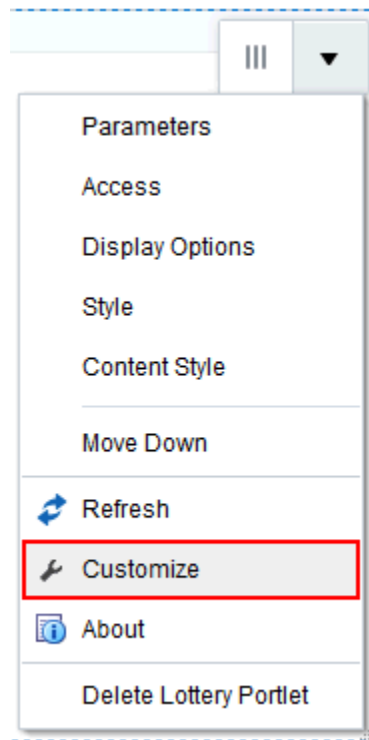
Figure 11-6 Customize Portlet
