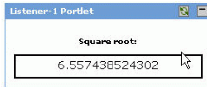
Figure 17-2 Listener -1 Portlet
