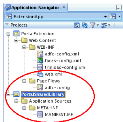
Figure 20-3 PortalSharedLibrary Project
