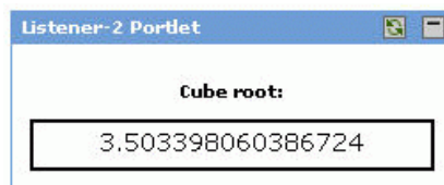
Figure 17-3 Listener -2 Portlet
