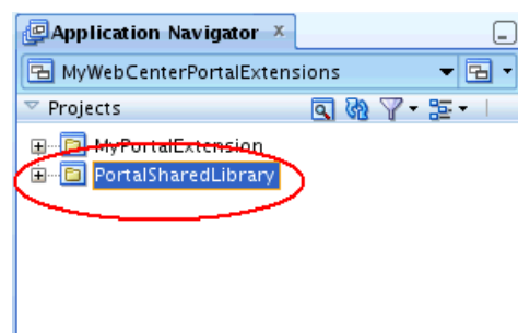
Figure 20-11 PortalSharedLibrary Project
