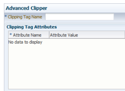
Figure 15-11 Advanced Clipper
