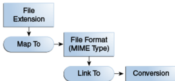
Figure 21-1 Mapping File Formats to a Conversion
