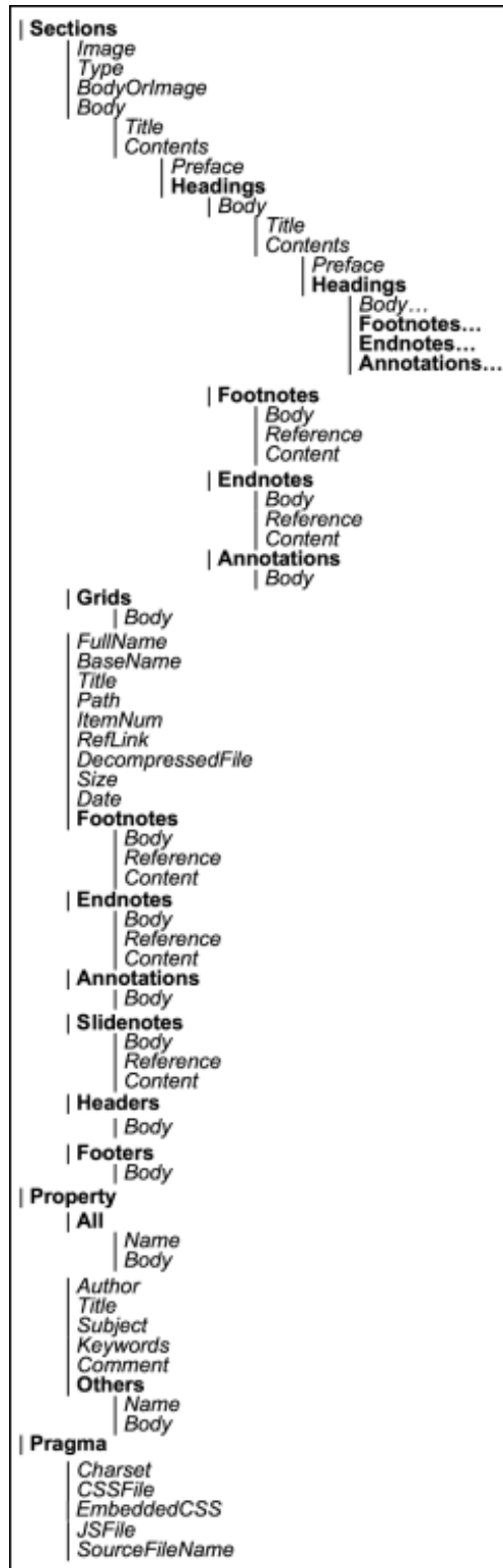
Figure 33-1 Example of an Element Tree
