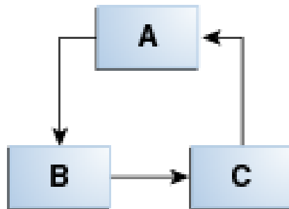
Figure 18-1 Renditions Links
