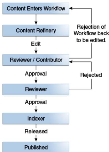
Figure 6-1 Workflow Process
