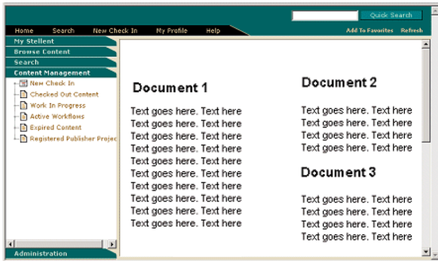
Figure 32-3 Default Layout
