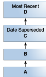
Figure 18-2 Supersedes Links
