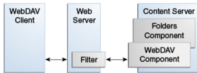
Figure 5-1 WebDAV Process
