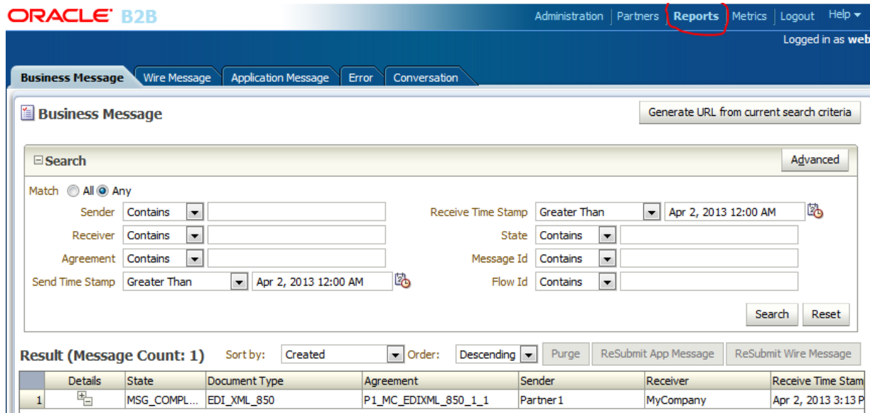
Figure 10-3 Reports Tab
