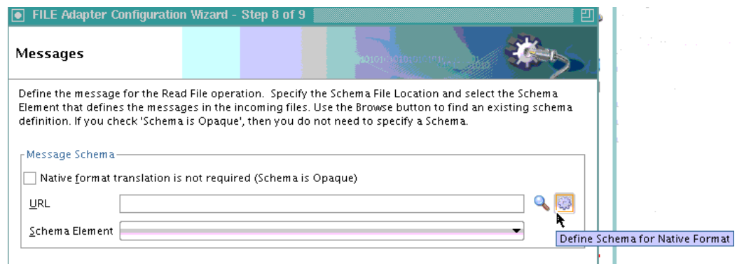
Figure 5-3 Selection of Option to Define a Schema for a Native Format
