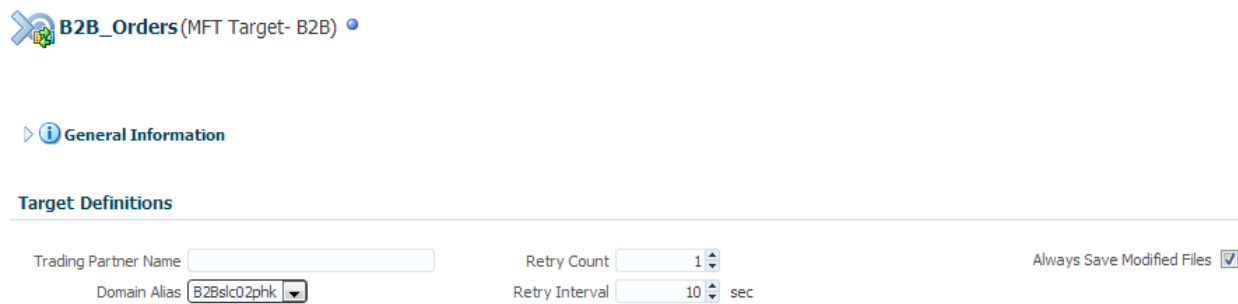
Figure 10-6 B2B_Orders Target
