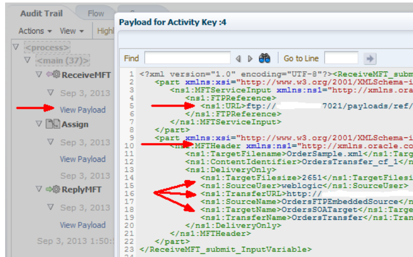
Figure 9-10 Audit Trail
