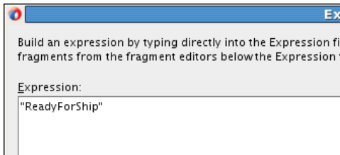
Figure 4-18 ReadyForShip Expression
