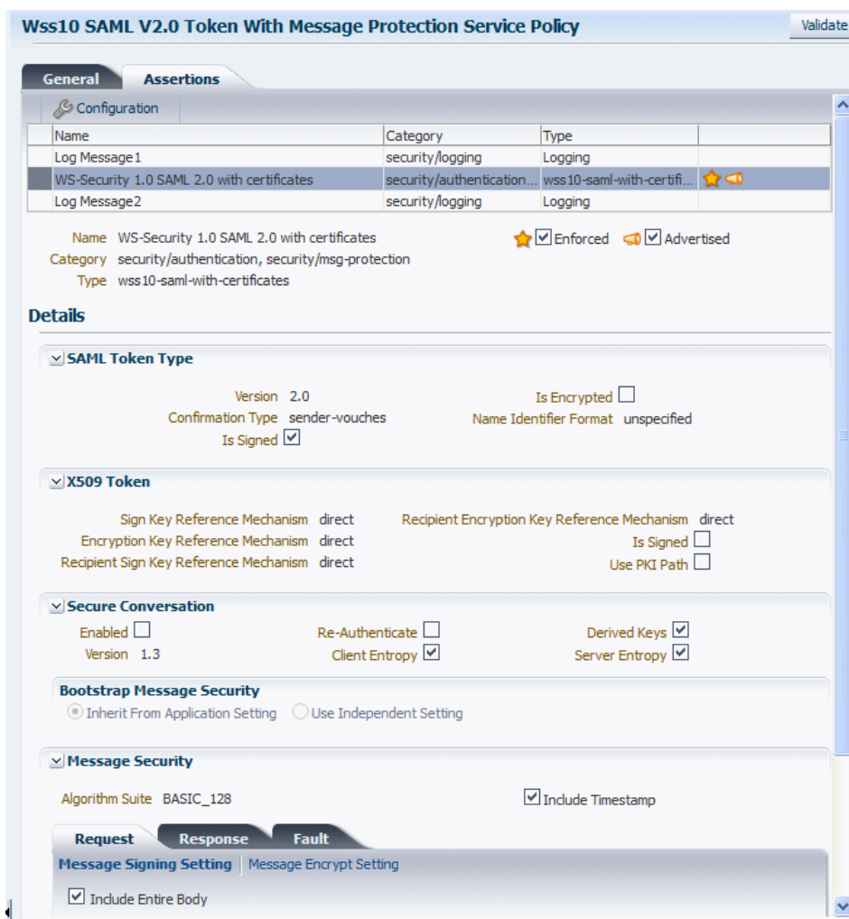
Figure 6-3 Policy Details Page with the Assertion Tab Selected
