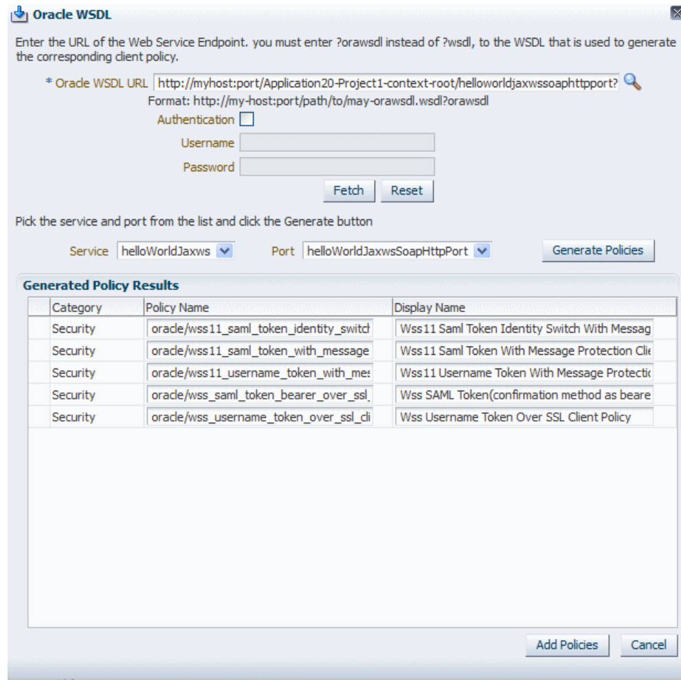
Figure 6-4 Generate Client Policies from WSDL
