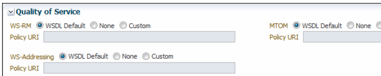
Figure 5-14 Quality of Service Parameters on the Test Web Service Page
