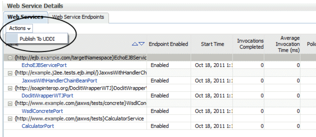
Figure 9-7 Web Services Summary Page with Publish to UDDI Selected
