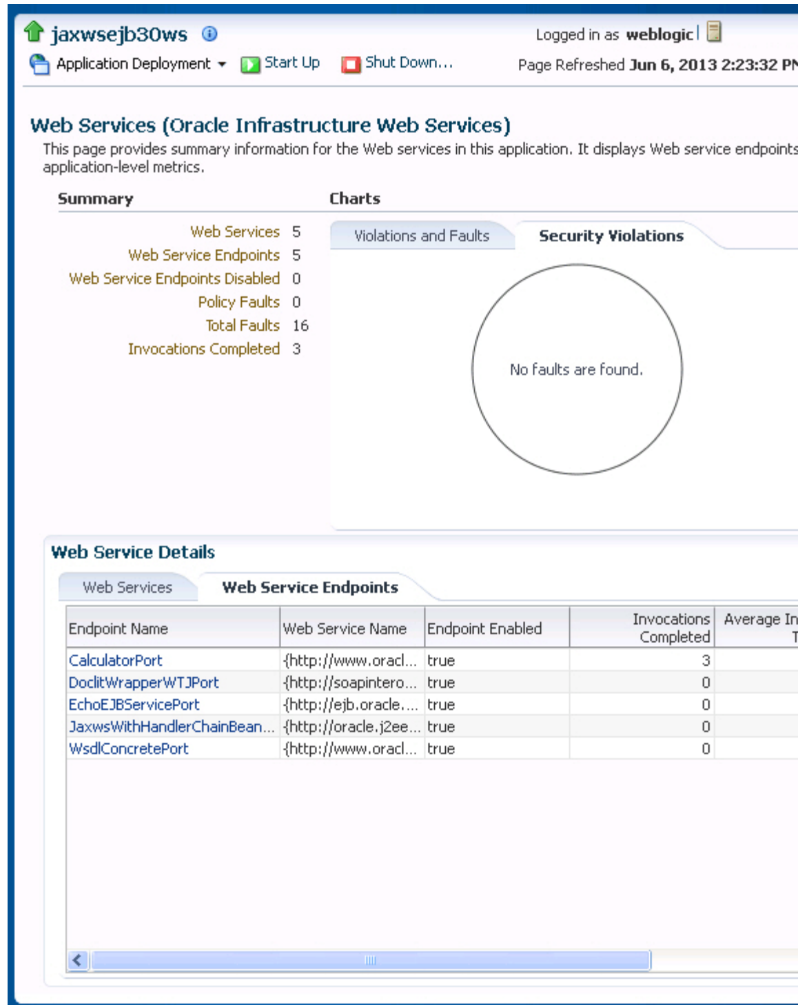
Figure 4-2 Web Services Summary Page for ADF Applications
