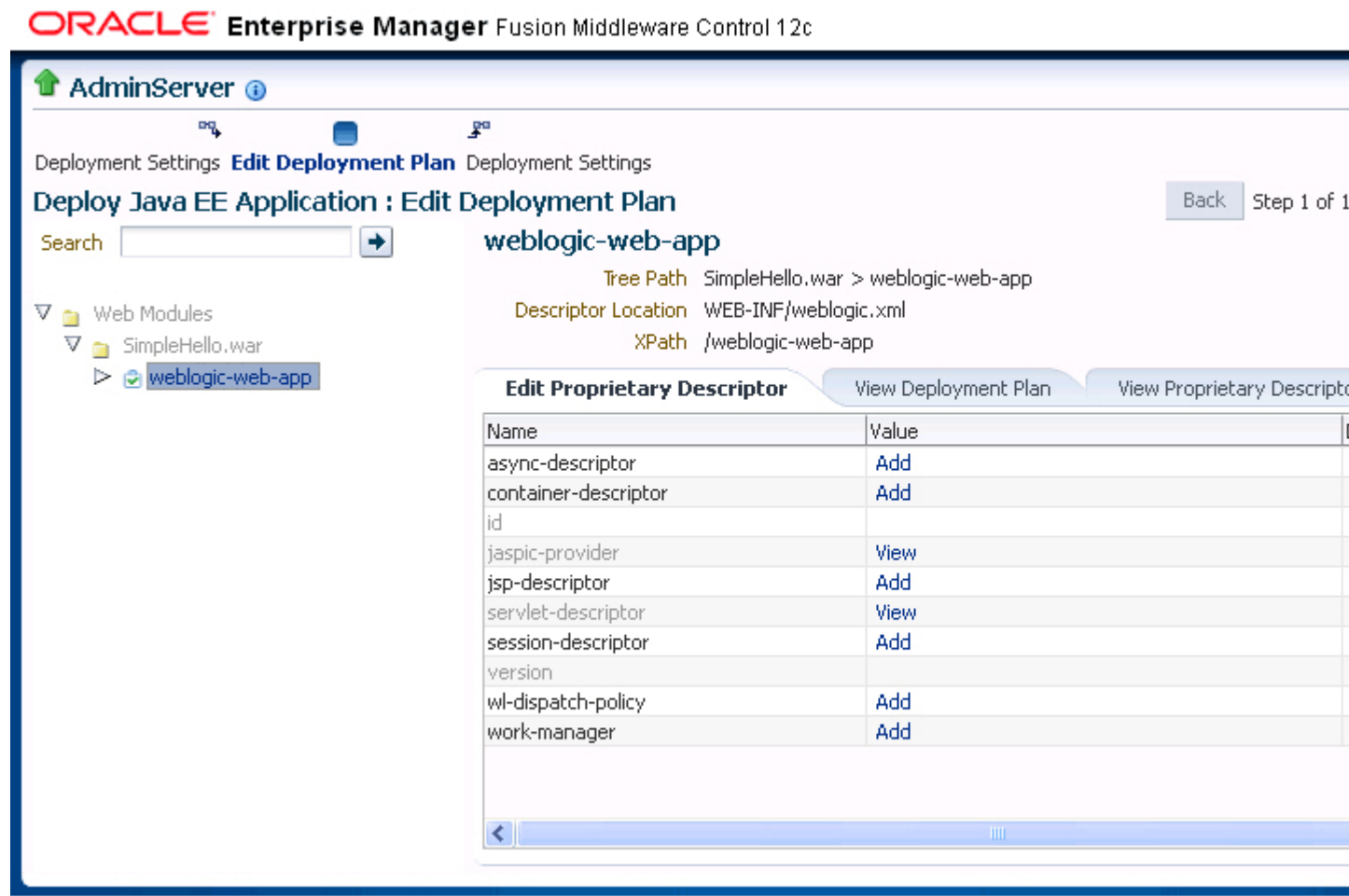
Figure 3-5 Edit Deployment Plan
