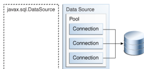
Figure 12-1 Oracle Stream Analytics Data Source
