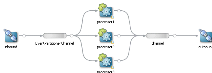
Figure 18-1 EventPartitioner EPN
