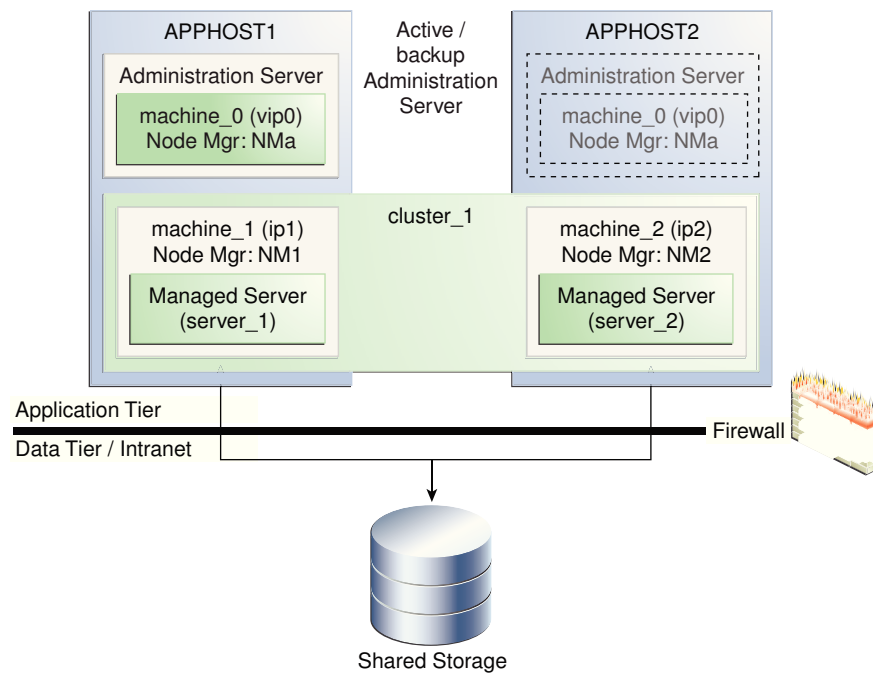
Figure 9-1 Administration Server High Availability Topology
