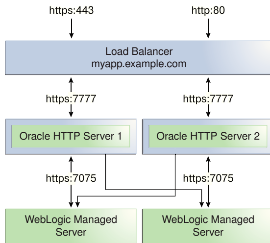
Figure 10-1 Oracle HTTP Server High Availability Architecture
