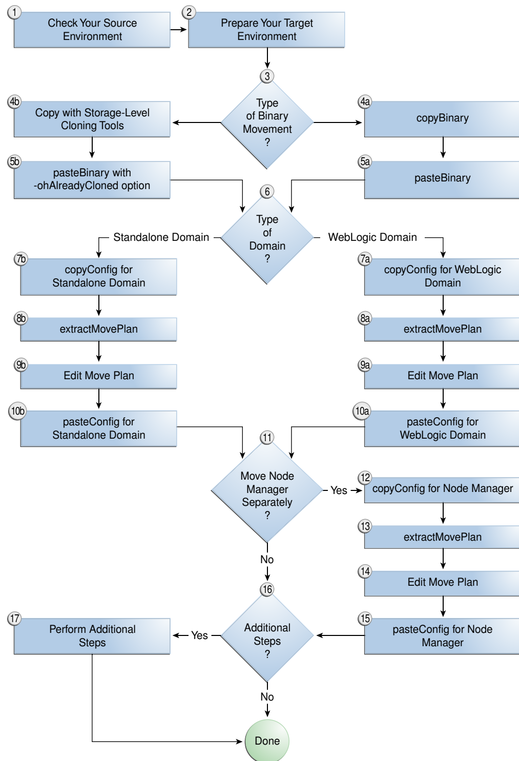
Figure 20-1 Flowchart for Moving Your Environment
