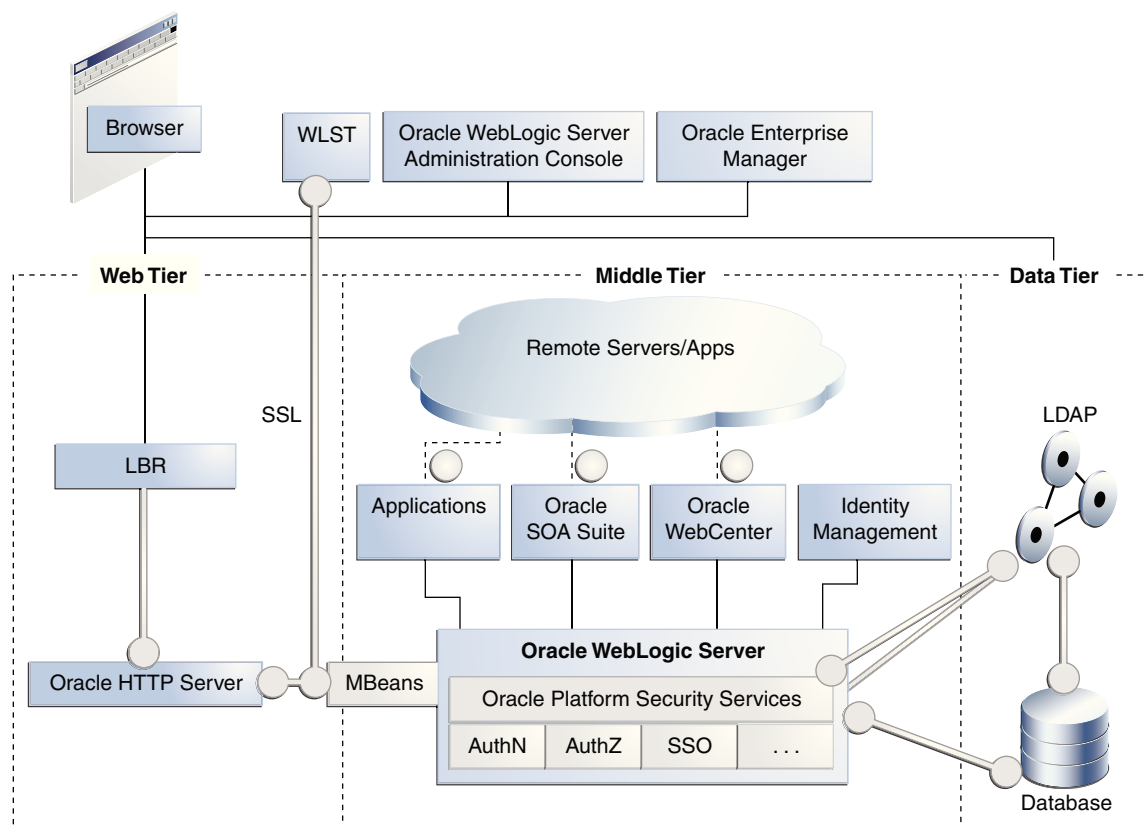
Figure 6-2 SSL in Oracle Fusion Middleware
