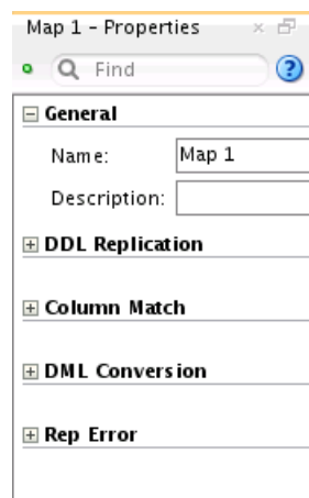
Figure 2-9 Properties Inspector
