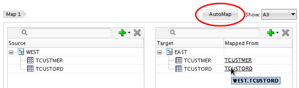
Figure 4-3 Automap
