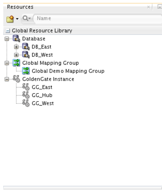
Figure 2-3 Resources Navigator
