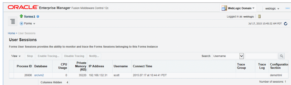
Figure 3-5 User Sessions page
