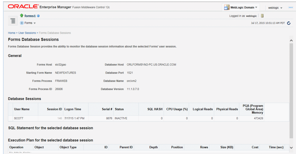
Figure 3-6 Database Sessions Page
