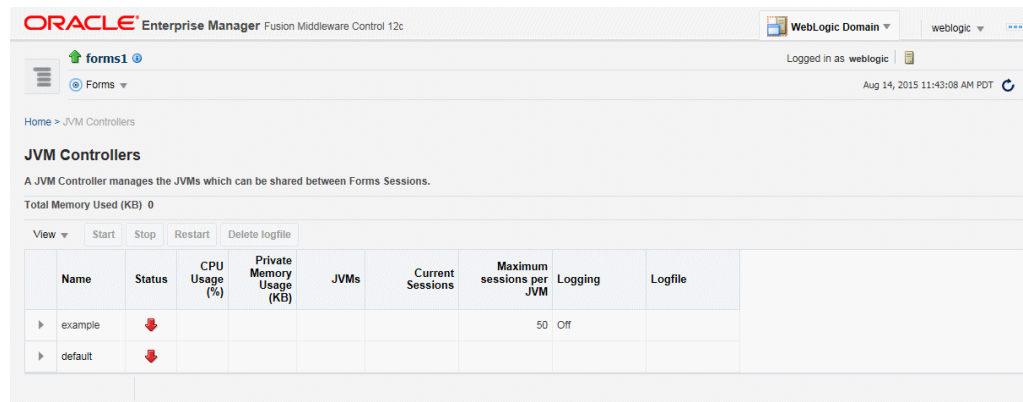
Figure 10-5 JVM Controller Page
