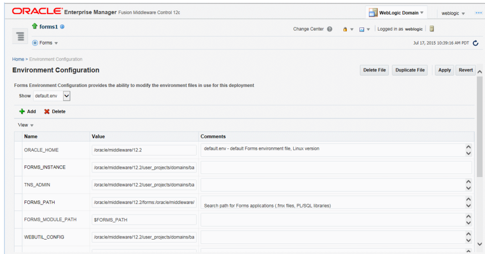
Figure 3-4 Environment Configuration page
