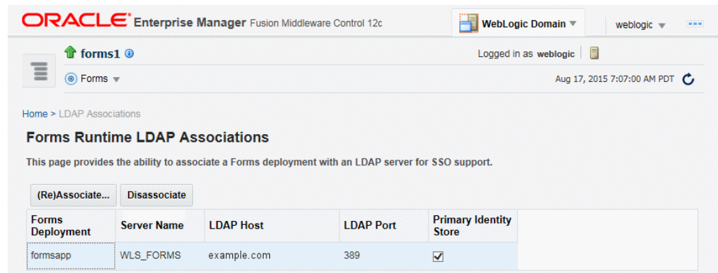
Figure 9-7 Forms Runtime LDAP Associations
