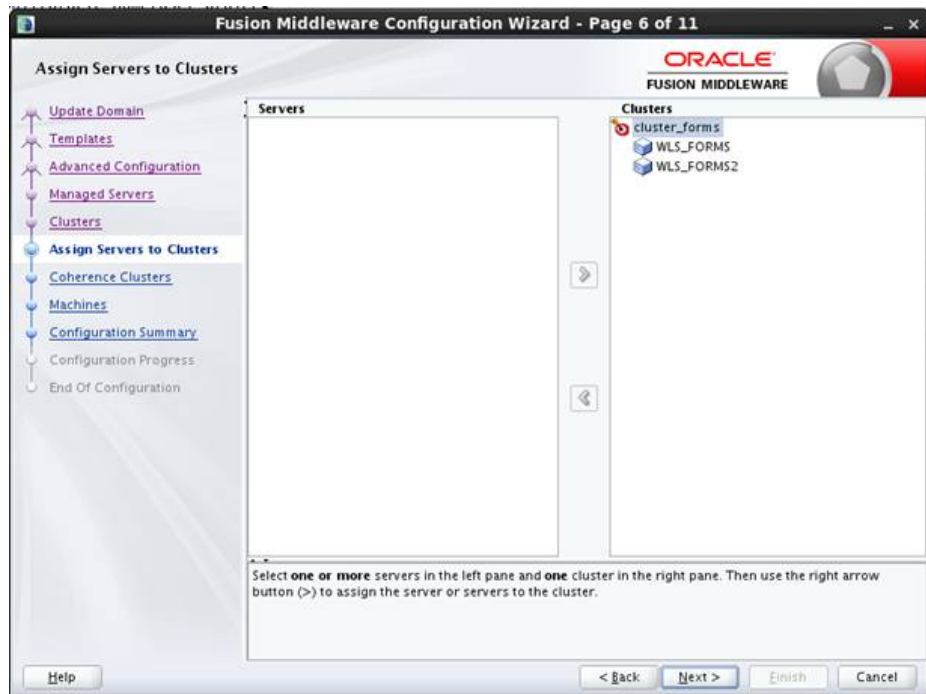
Figure 5-4 Fusion Middleware Configuration Wizard
