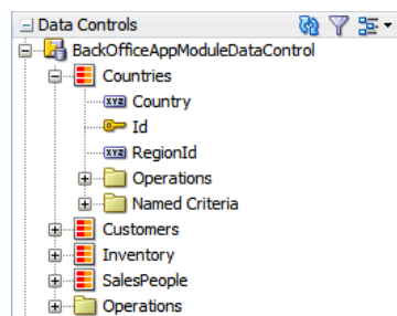
Figure 1-13 BackOfficeAppModuleDataControl
