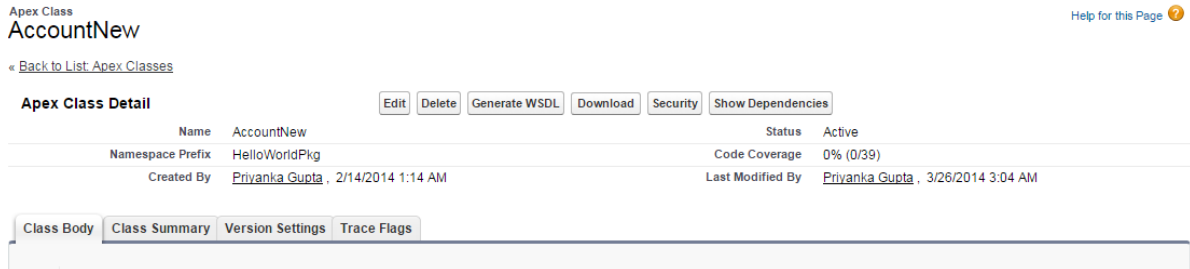
Figure 4- 18 Account New
