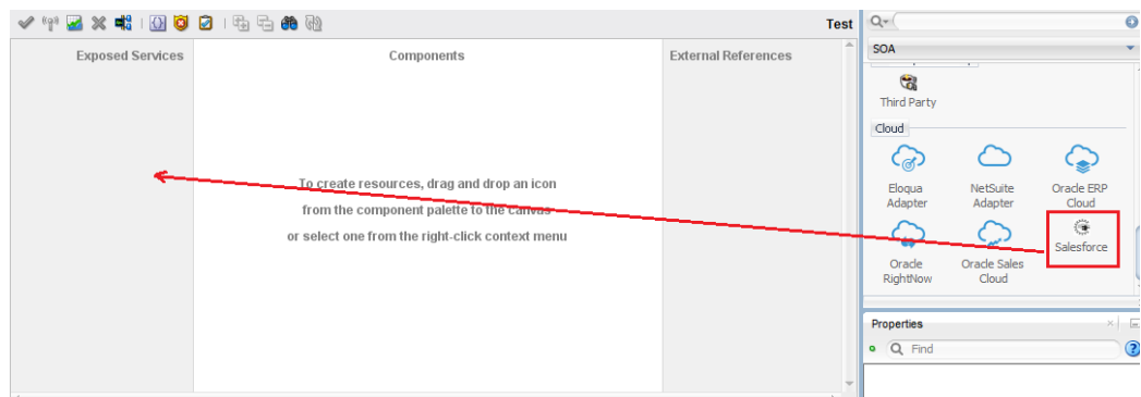
Figure 4-24 Salesforce Adapter
