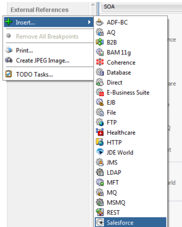
Figure 5- 11 Salesforce Adapter
