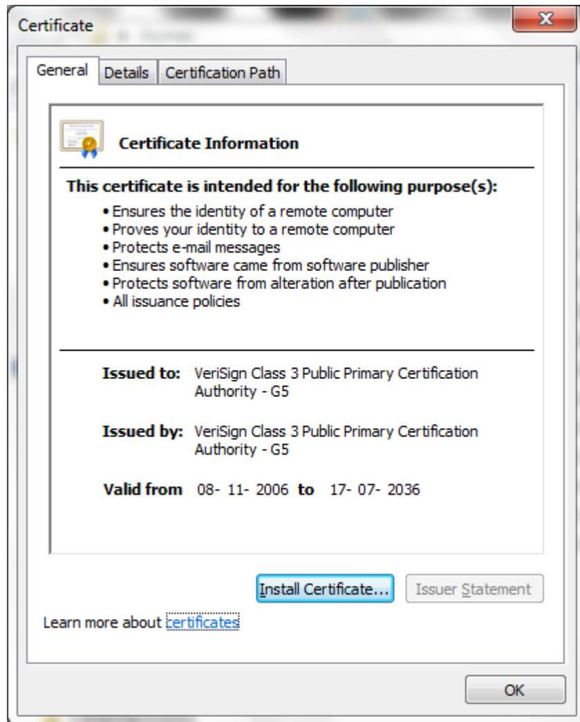
Figure 2-9 Certificate Information
