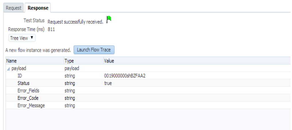
Figure 5-43 Test Status
