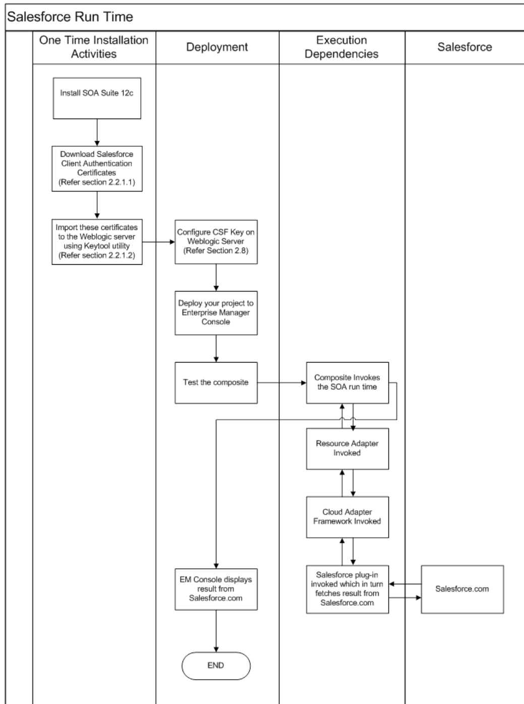
Figure2- 13 Run-Time Lifecycle
