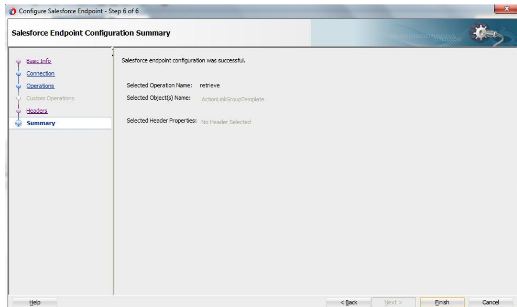
Figure 10 - 21 Finish Page
