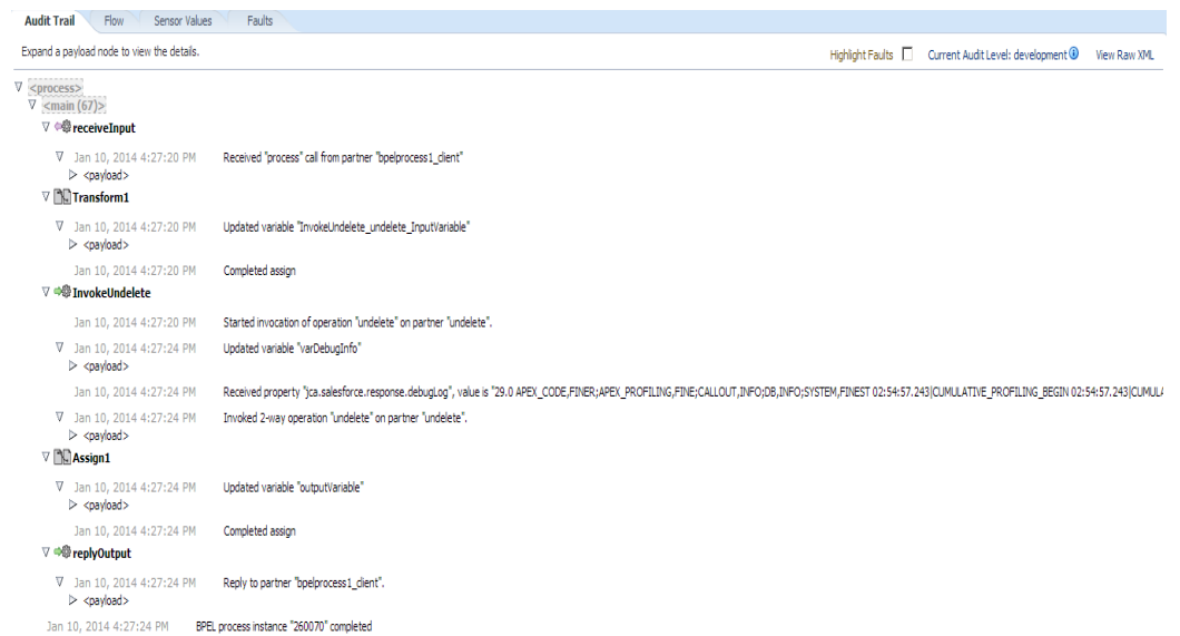
Figure 10 - 121 Audit Trail
