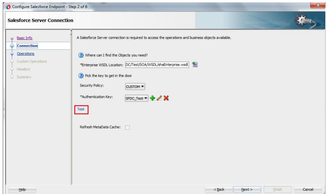
Figure 6-27 Connection Page
