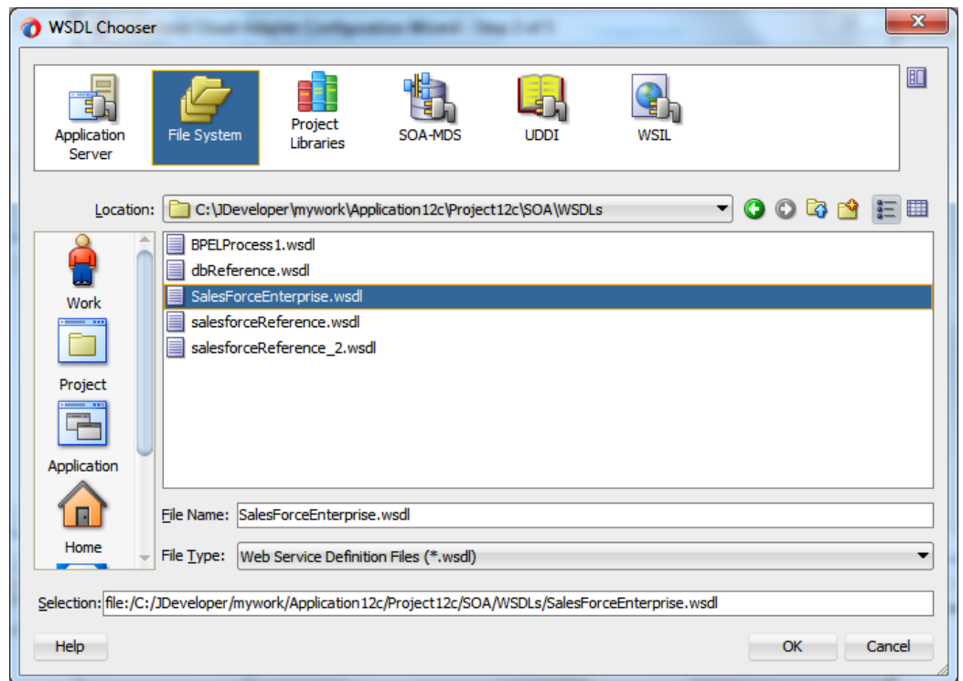
Figure 2-19 WSDL Chooser
