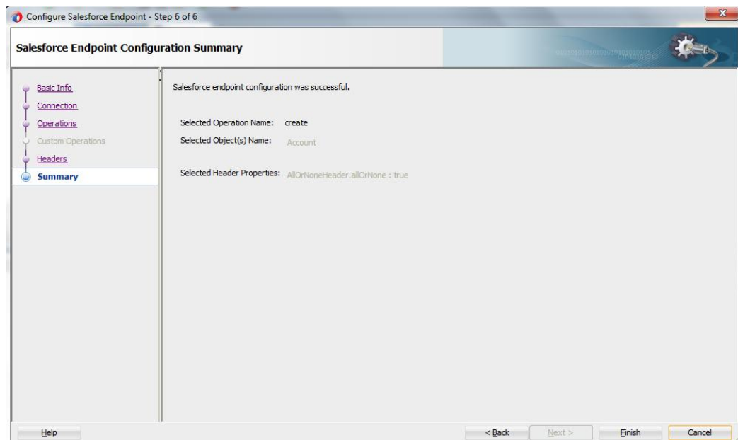
Figure 5- 25 Finish Page
