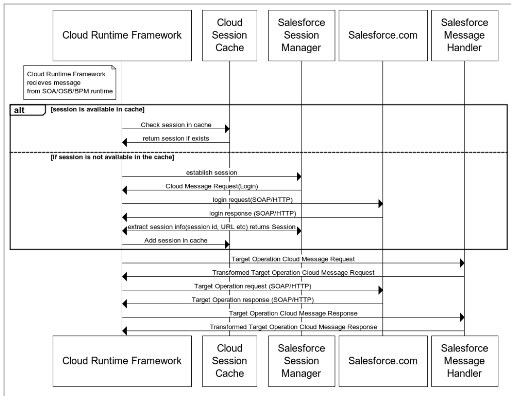
Figure 3- 25 Execution Phase
