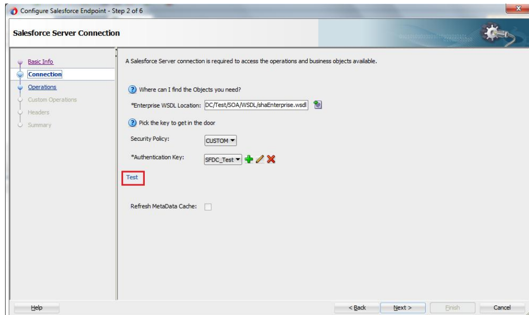
Figure 10 - 89 Test Connection
