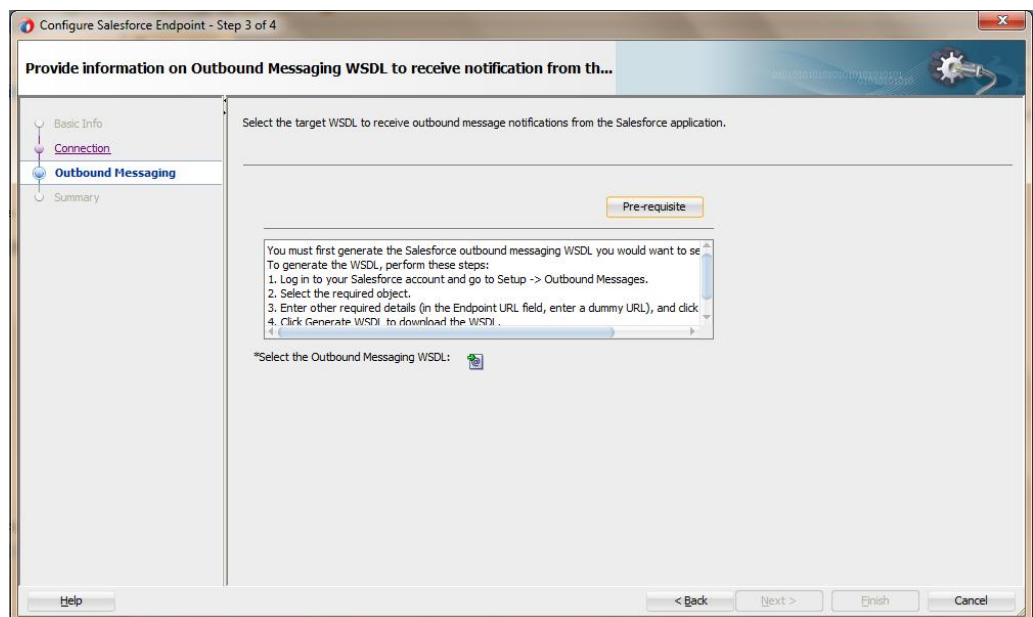
Figure 4-26 Outbound Messaging
