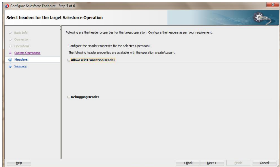
Figure 4- 19 Headers Page
