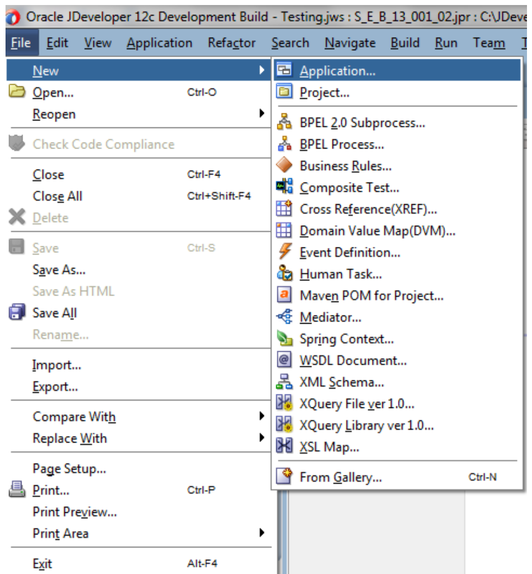
Figure 5-1 Navigation Window
