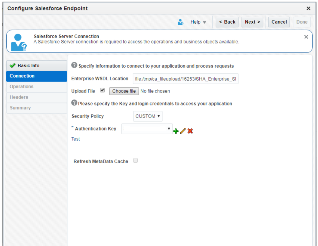
Figure 6-55 Connection Page
