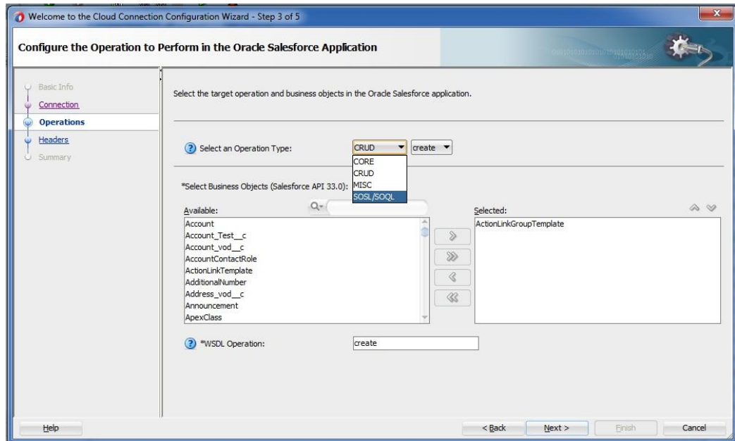
Figure 10 - 16 Select SOQL
