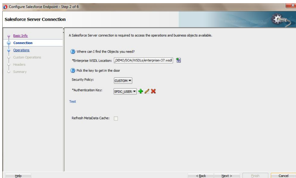
Figure 8- 1 WSDL Location
