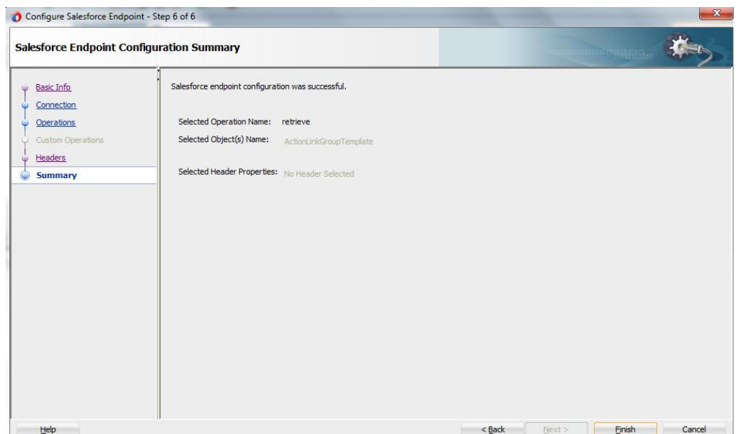
Figure 4- 16 Finish Page
