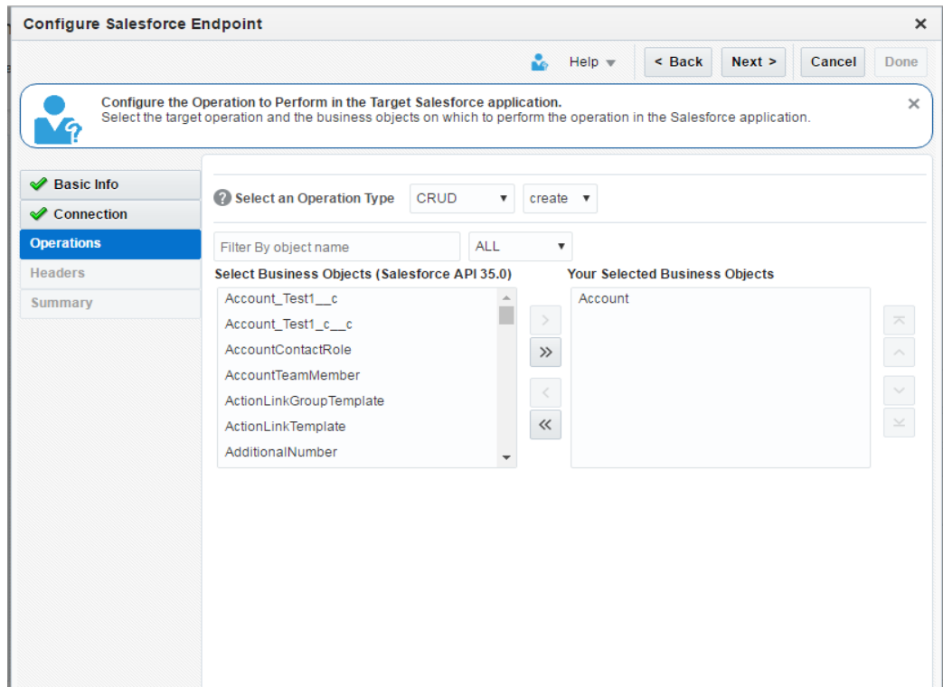
Figure 6- 58 Operations Page
