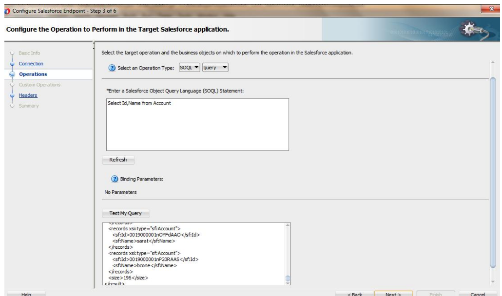
Figure 10 - 19 Query Test
