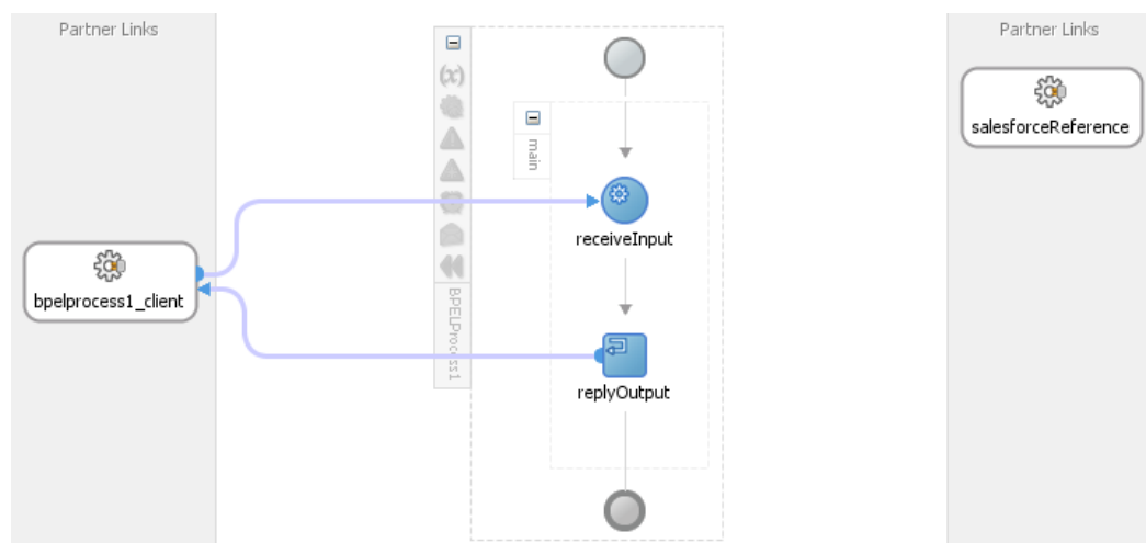
Figure 5-29 Open BPELProcess1
