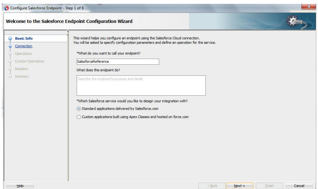
Figure 5- 12 Welcome Page
