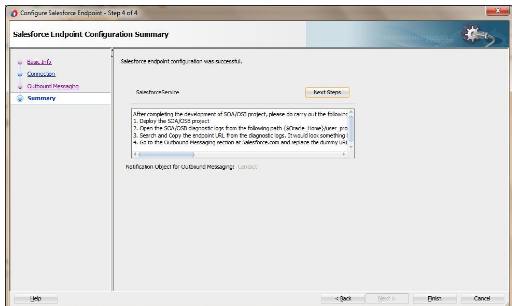
Figure 4- 27 Summary Page
