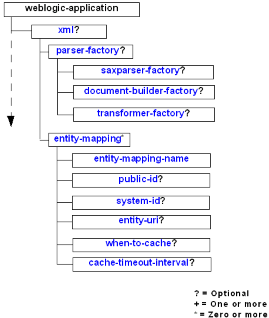
Figure 8-1 Sub-Elements of the &lt;xml&gt; Element in weblogic-application.xml
