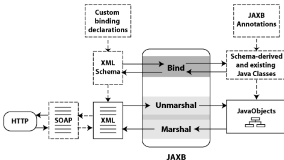
Figure 5-1 Data Binding With JAXB
