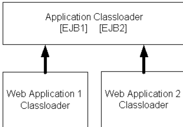
Figure 11-2 Standard Classloader Hierarchy
