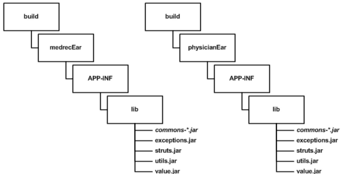
Figure 4-9 Shared JAR Files in MedRec
