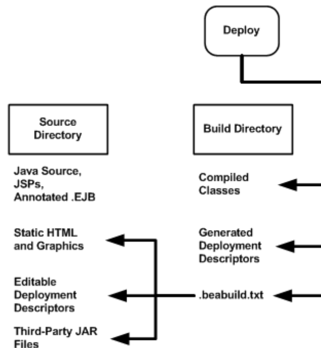
Figure 4-2 Split Directory Deployment
