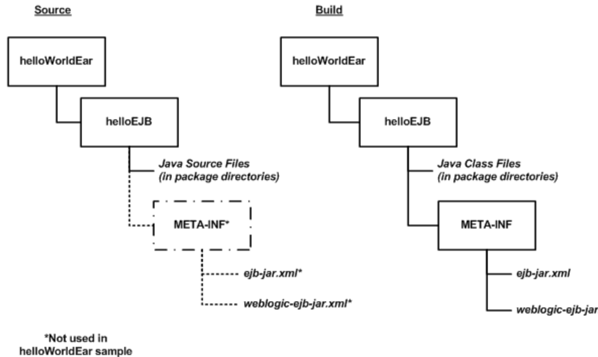
Figure 4-6 EJB Source and Build Directories
