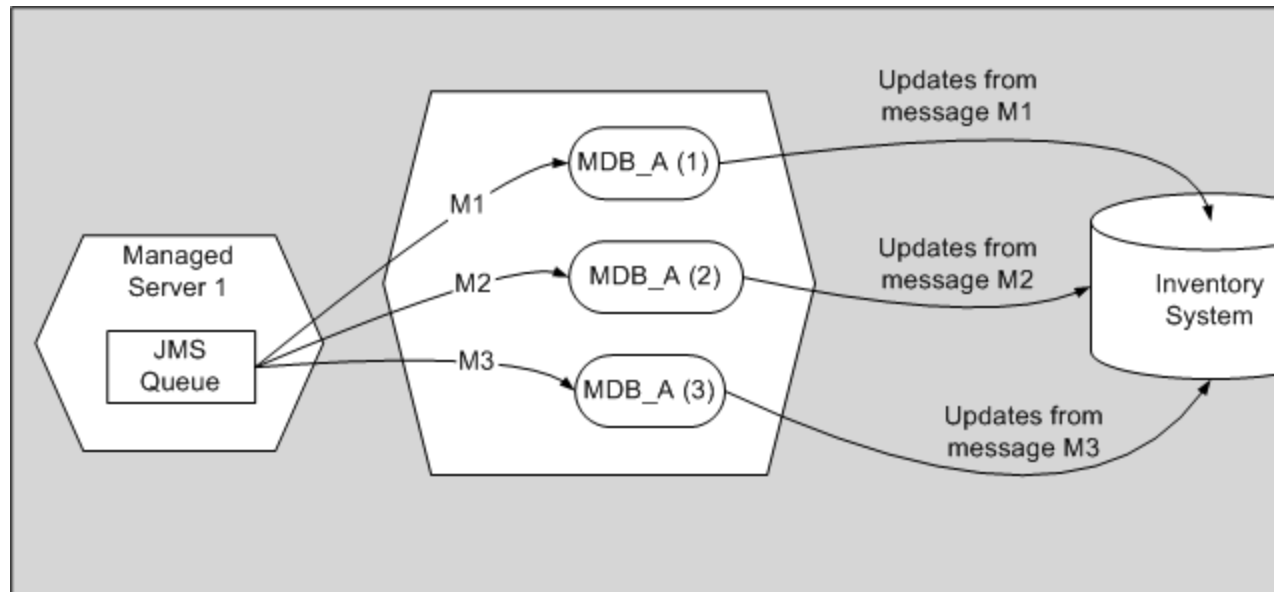
Figure 3-1 Point-to-Point Model
