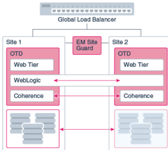
Figure 6-3 Domain Configuration for Active-Active Stretch Cluster Recovery
