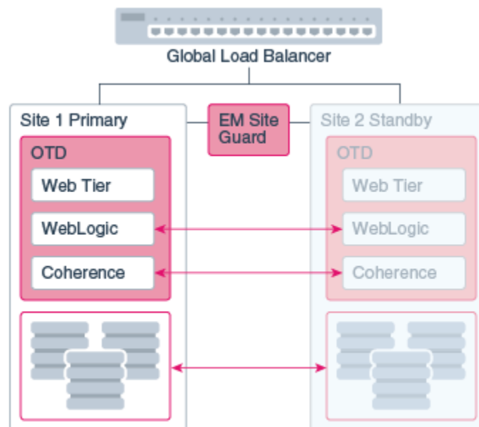
Figure 6-2 Domain Configuration for Active-Passive Recovery
