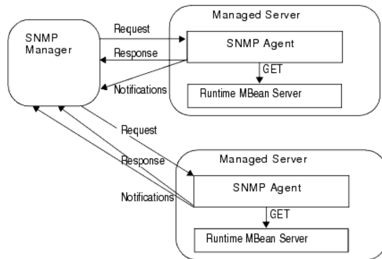
Figure 2-1 De-Centralized Model for SNMP Monitoring and Communication
