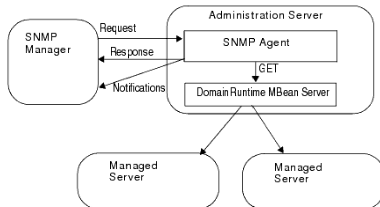
Figure 2-2 Centralized Model for SNMP Monitoring and Communication
