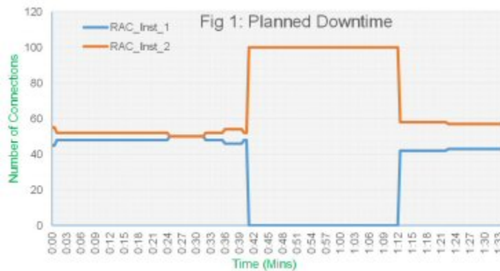
Figure 6-6 Distribution of Connections Across Two Oracle RAC Instances
