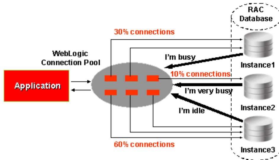
Figure 6-3 Runtime Connection Load Balancing
