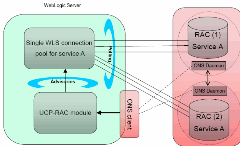
Figure 6-1 Active GridLink Data Source Connectivity
