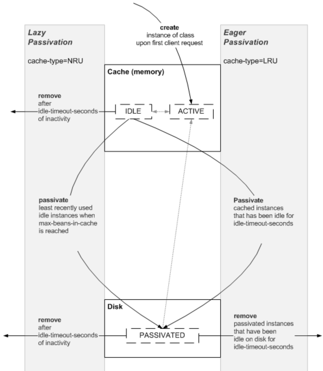
Figure 5-2 Stateful Session EJB Life Cycle
