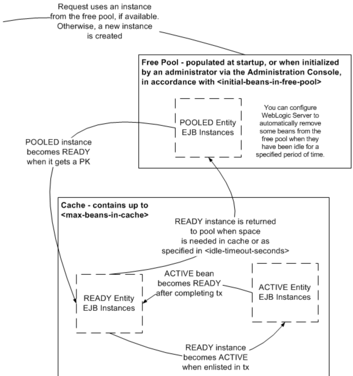
Figure 6-1 Entity Bean Life Cycle
