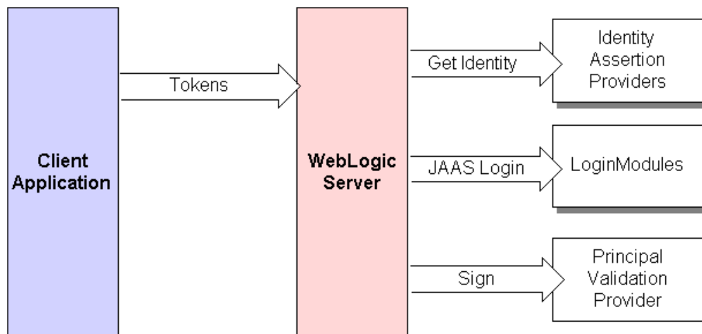
Figure 5-2 Perimeter Authentication
