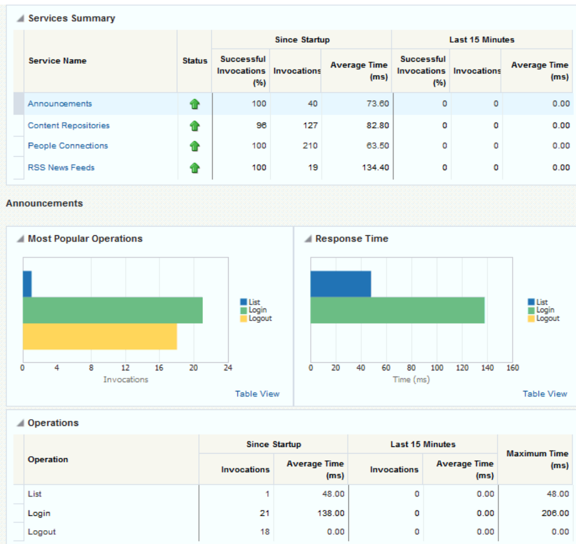
Figure 22-14 Announcements Metrics
