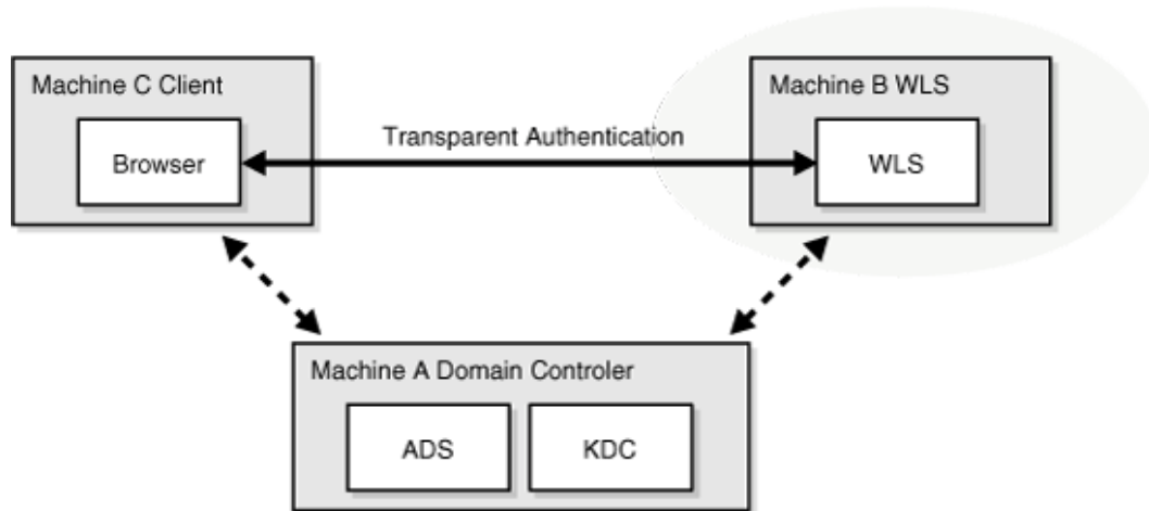
Figure 28-7 SPNEGO-based Authentication
