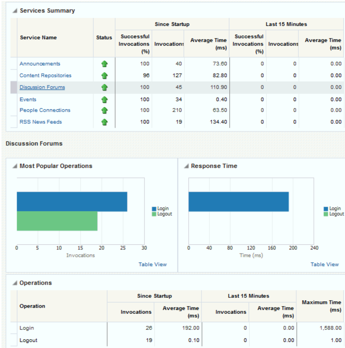
Figure 22-17 Discussion Metrics
