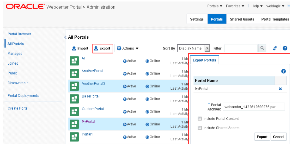
Figure 34-10 Exporting Portals
