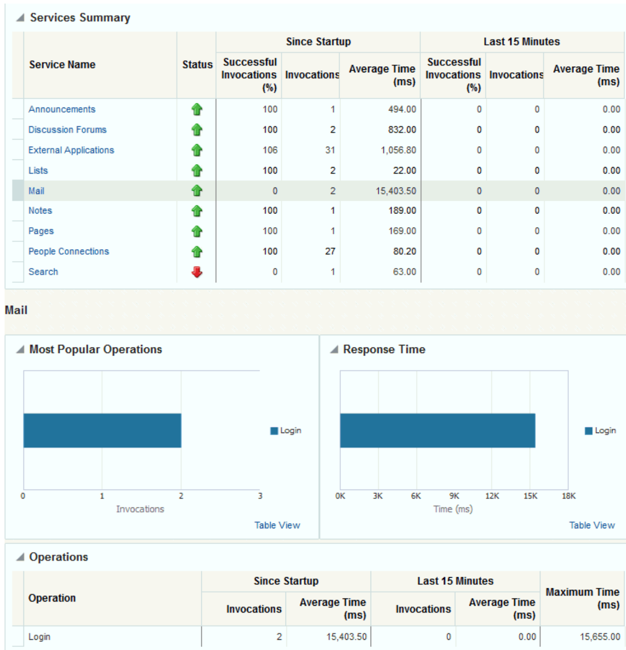
Figure 22-23 Mail Metrics
