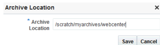
Figure 35-6 Archive Location
