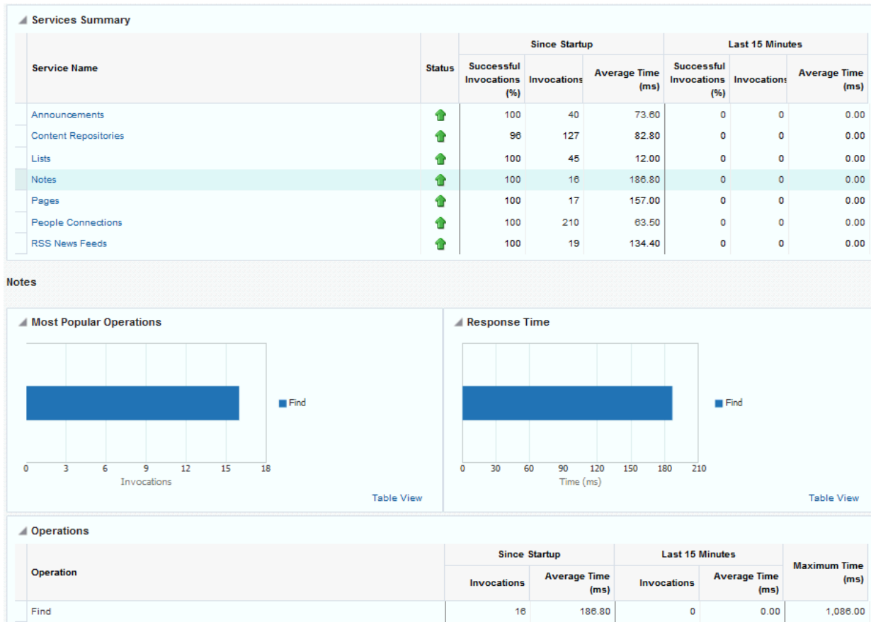
Figure 22-24 Notes Metrics
