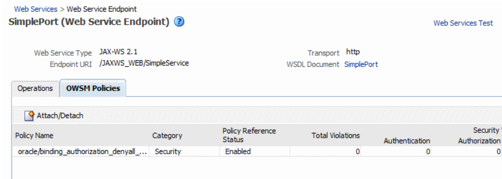
Figure 4-13 Policies Attached to a WebLogic Java EE Web Service Endpoint
