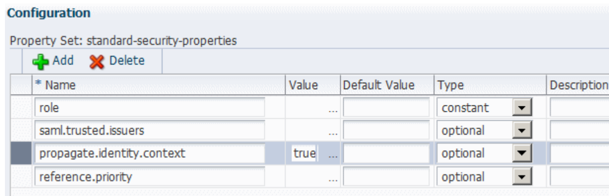
Figure 11-6 Setting the propagate.identity.context Property to True
