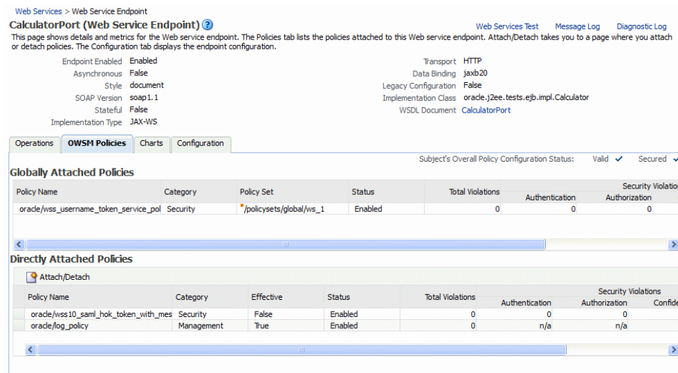
Figure 4-12 Policies Attached to an Oracle Infrastructure Web Service Endpoint
