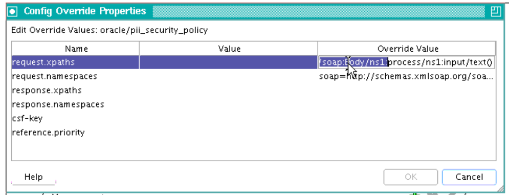
Figure 8-3 Overriding request.xpath s Attribute
