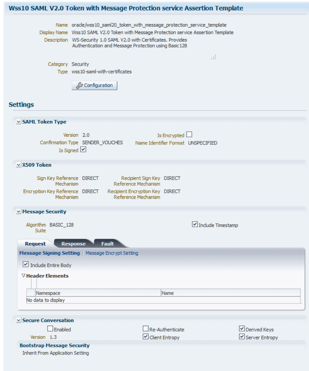
Figure 6-7 Assertion Template Details Page
