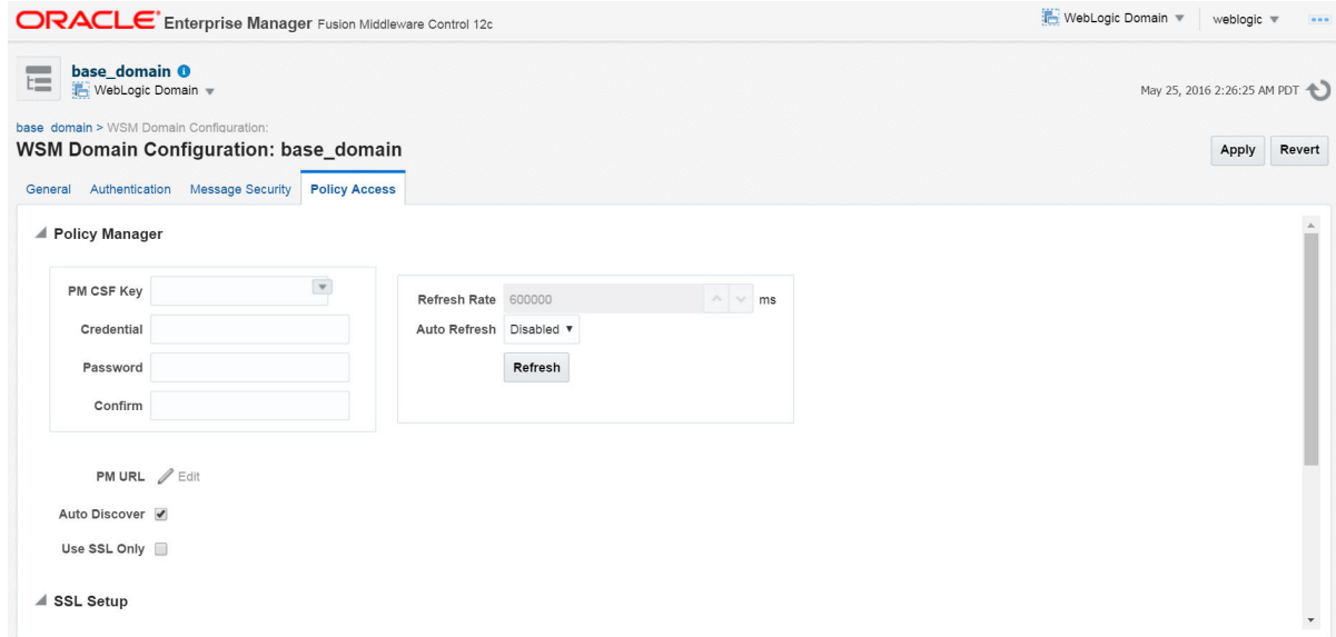
Figure 14-9 Policy Access Tab in WSM Domain Configuration Page Showing the Status of Auto Refresh
