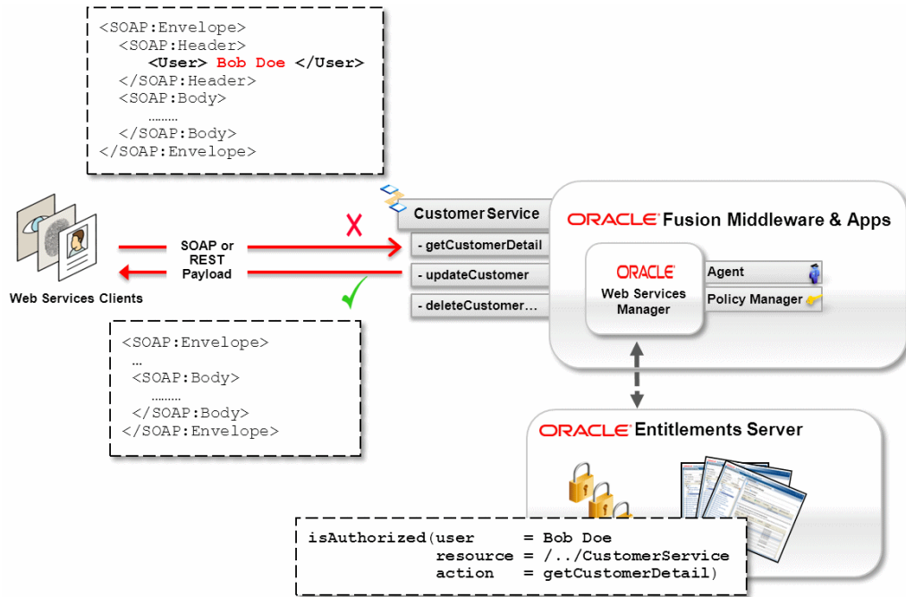
Figure 2-5 Coarse-Grained Authorization
