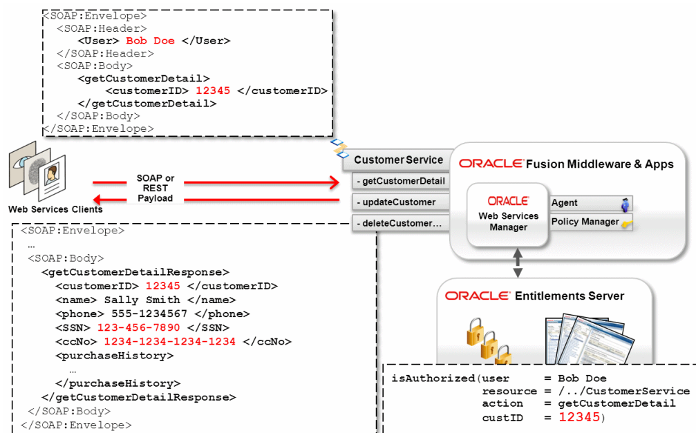
Figure 2-4 Fine-Grained Authorization
