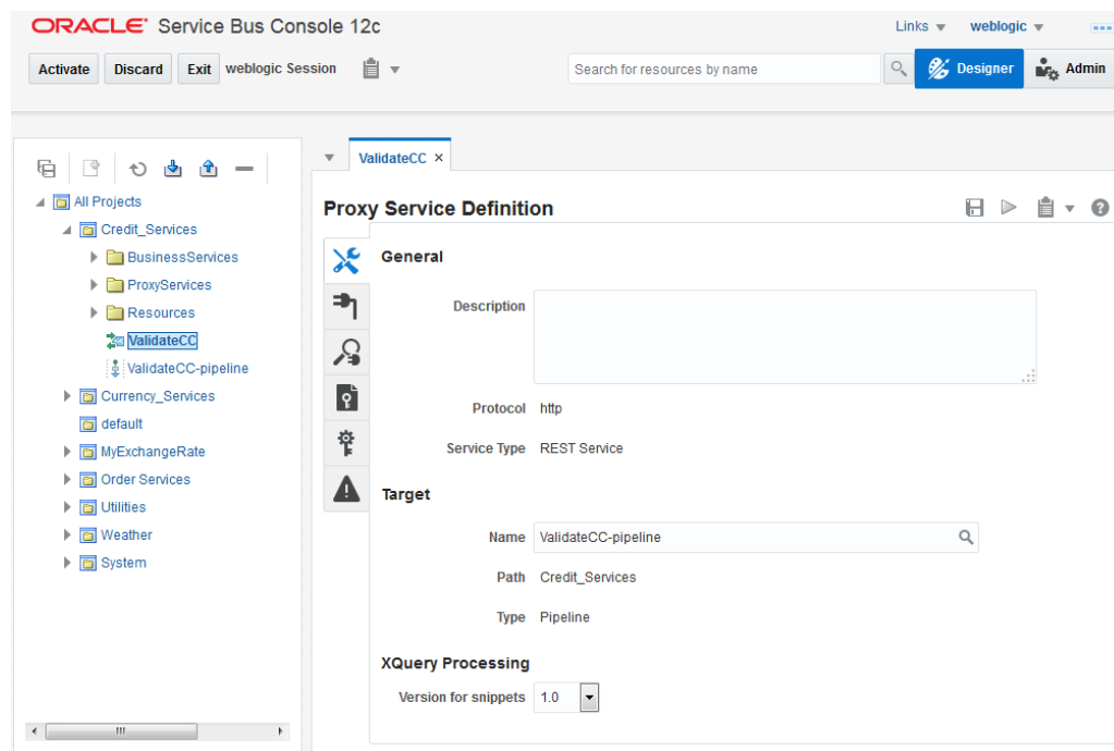
Figure 2-5 Proxy Service Definition Editor
