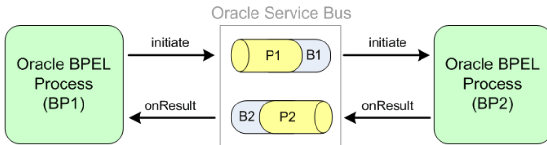
Figure 36-6 SOA Composite Invoking an SOA Composite Through Service Bus
