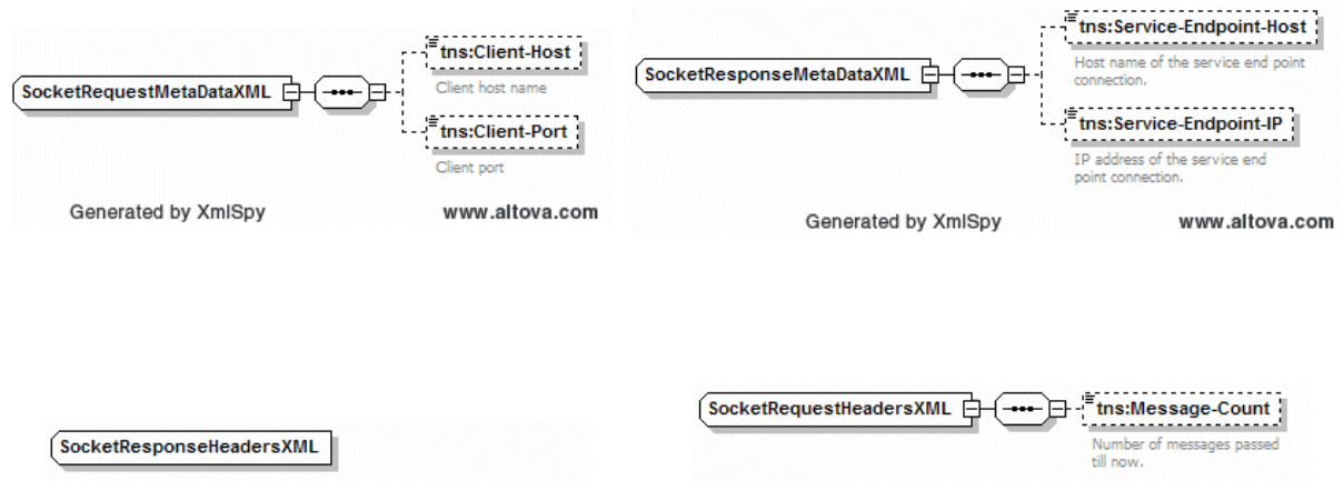
Figure 43-3 Request and Response Header and Metadata Configurations
