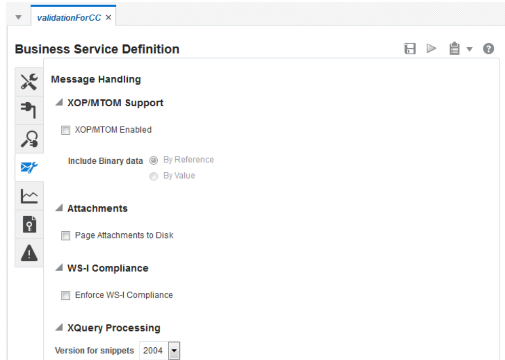
Figure 9-3 Business Service Message Handling Page in the Console
