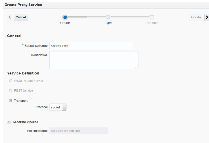
Figure 43-5 Create Proxy Service Wizard
