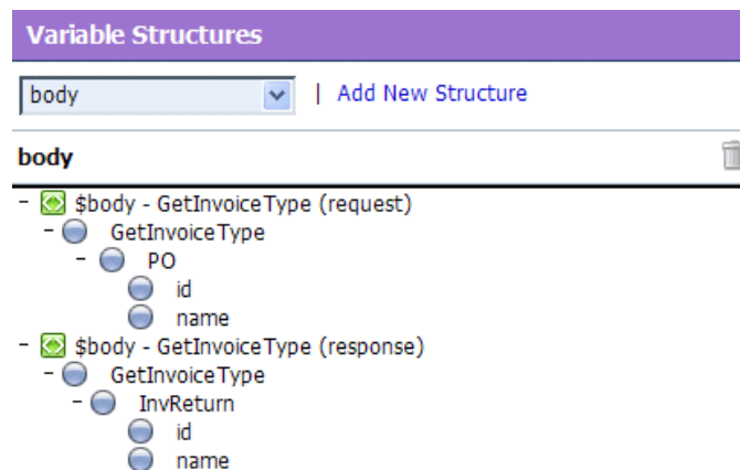
Figure 13-3 Variable Structures— body
