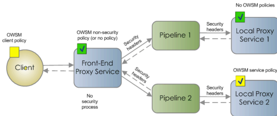
Figure 32-4 Front-end Proxy as Security Pass-through to Local Proxies
