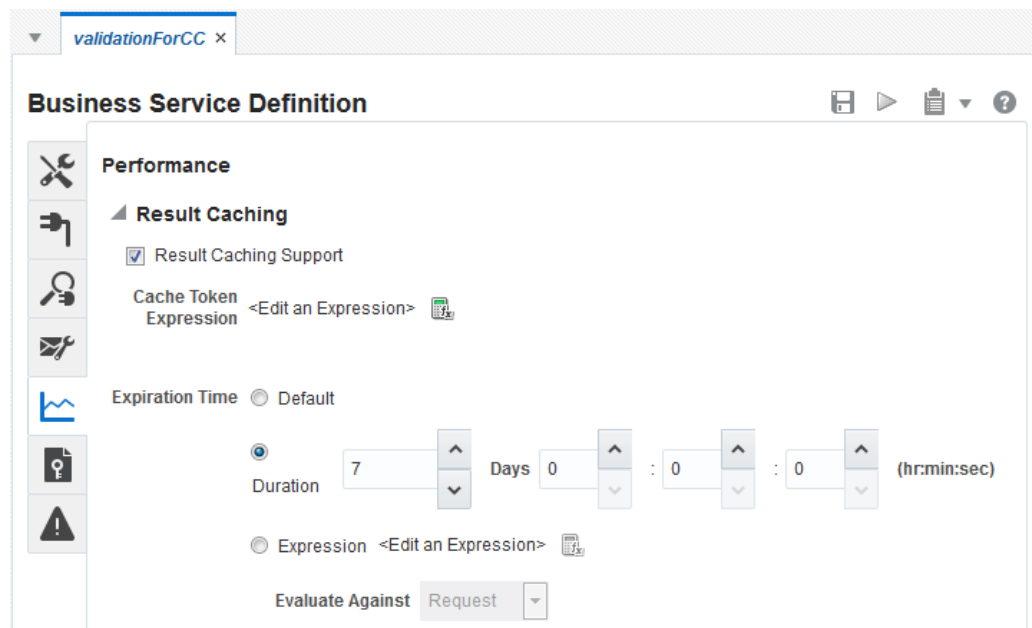
Figure 9-6 Business Service Performance Page in the Console
