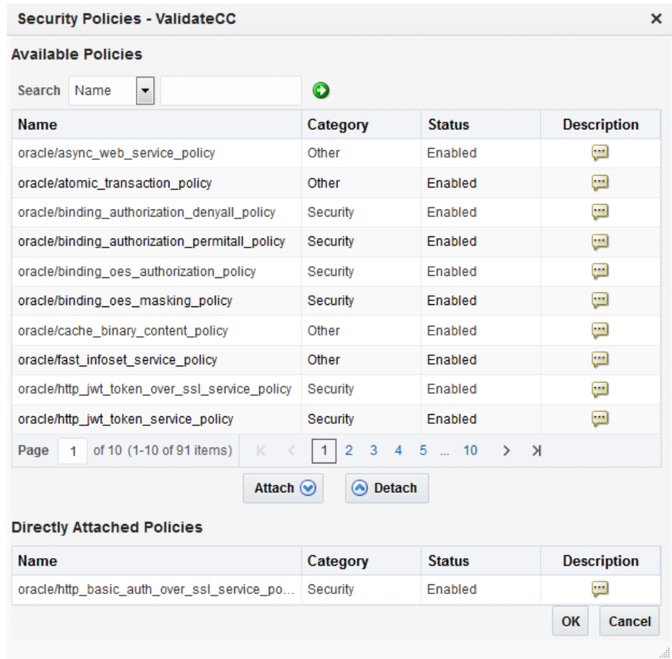
Figure 49-5 Security Policies Dialog in the Oracle Service Bus Console
