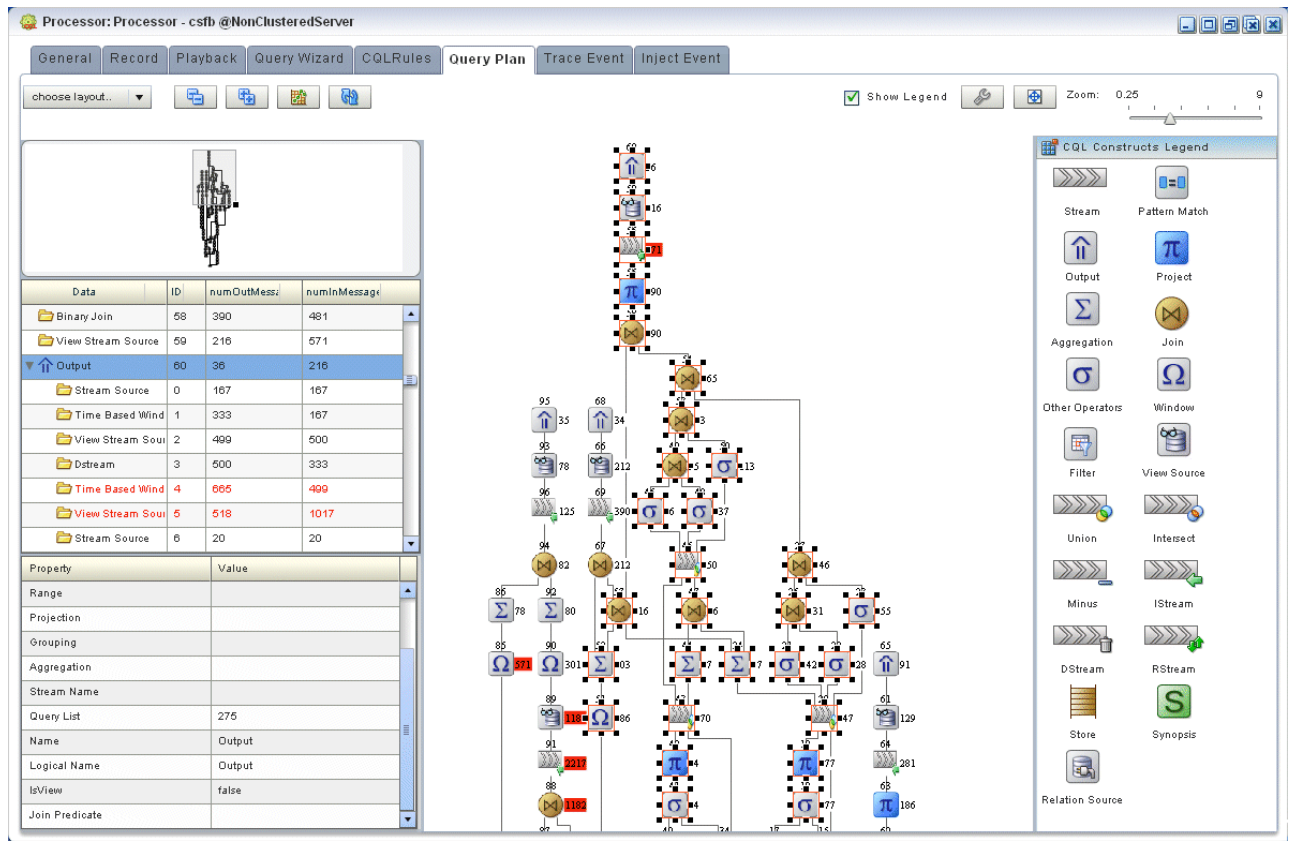
Figure 6-82 Query Plan Showing Dependencies
