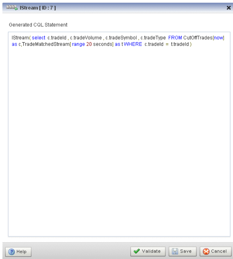
Figure 6-68 Query Wizard IStream Editor Dialog
