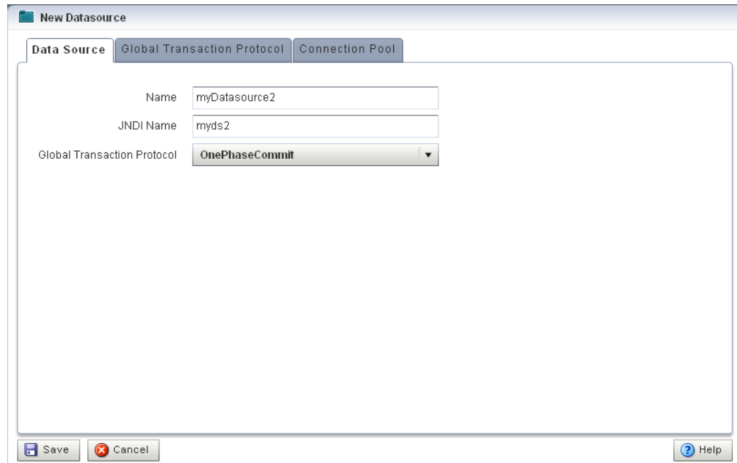
Figure 12-6 New Datasource: Data Source Tab
