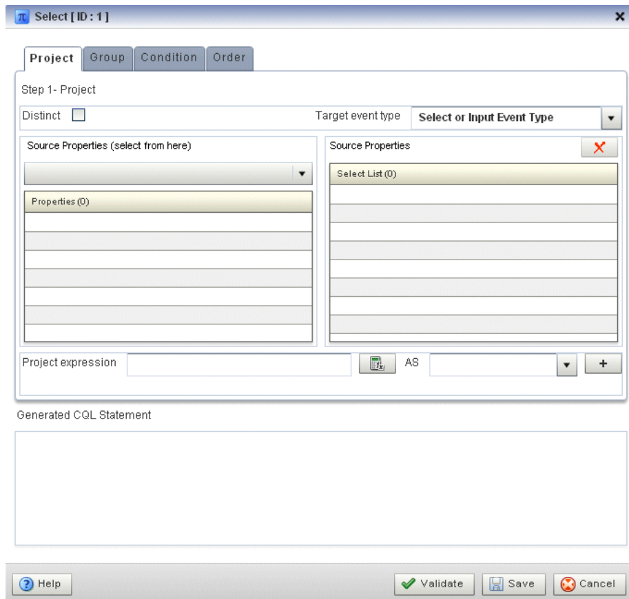
Figure 6-48 Query Wizard Select Editor Dialog: Project Tab
