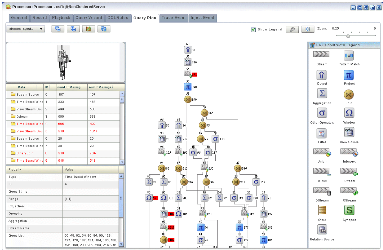
Figure 6-81 Query Plan While Getting Statistics
