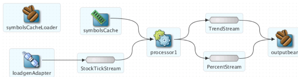
Figure 7-6 The Signal Generation Example Event Processing Network
