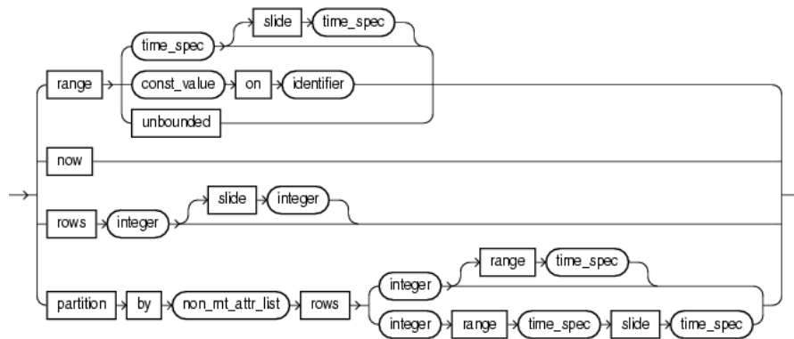
Figure 1-3 window_type
