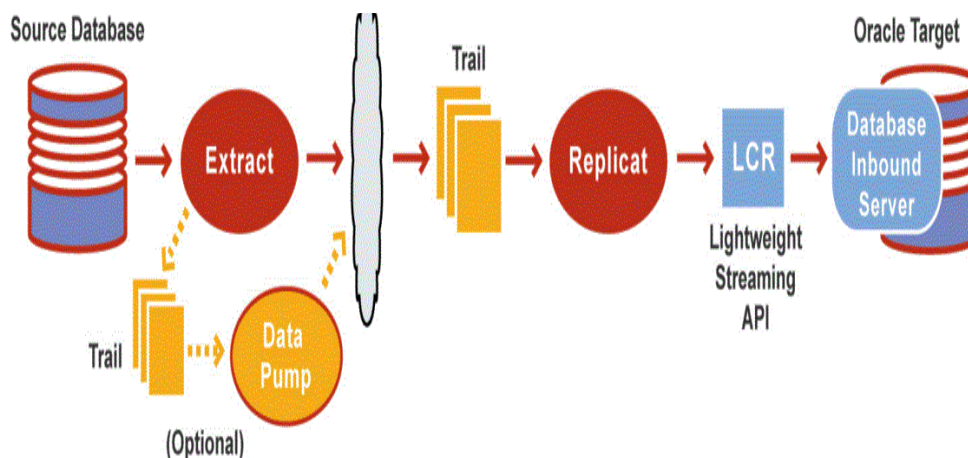
Figure 24–3 Integrated Replicat Configuration
