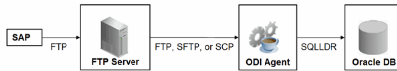
Figure 6–4 Configuration 2: FTP Server is not installed on ODI Agent machine
