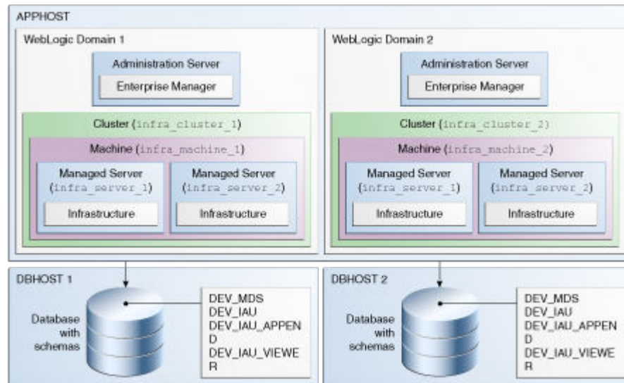
Figure 1-4 Schemas on Multiple Databases for Multiple Domains
