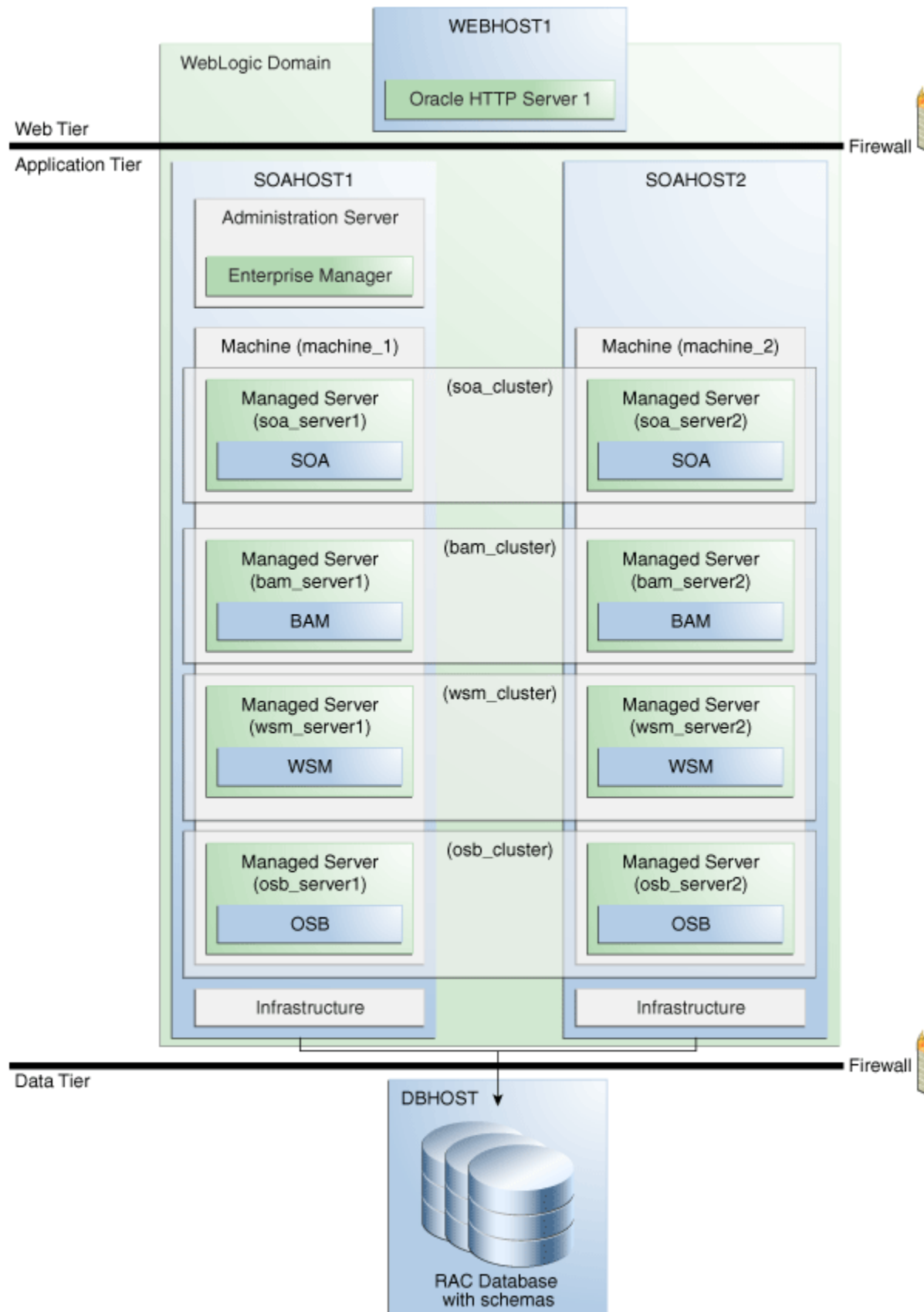
Figure 5-1 Clustered SOA Topology
