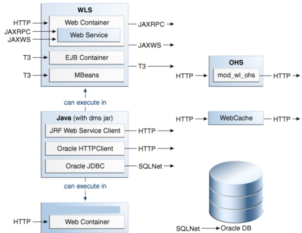
Figure 5-2 DMS Execution Context Communication Protocols
