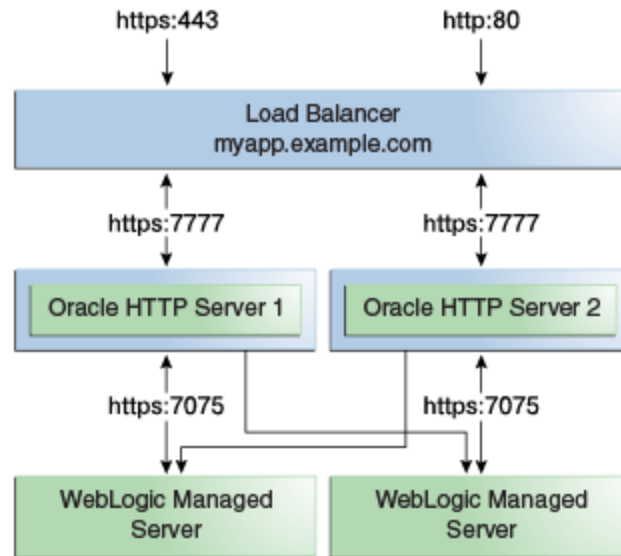
Figure 9-1 Oracle HTTP Server High Availability Architecture
