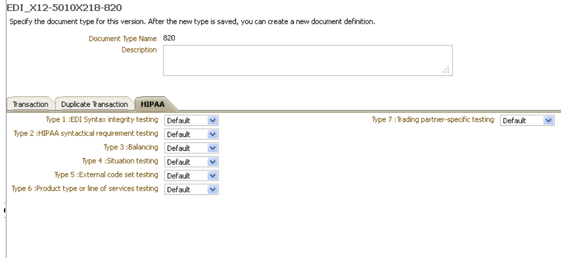
Figure J-1 Configuring SNIP at the Document Level
