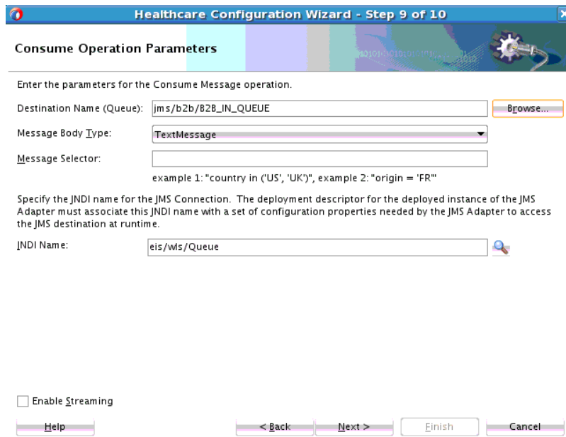
Figure 2-11 Healthcare Configuration Wizard - Consume Operations Page
