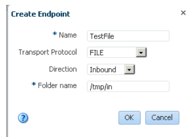
Figure 4-4 Specifying Endpoint Parameters
