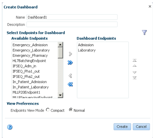
Figure 8-5 Create Dashboard Dialog with Endpoints Selected
