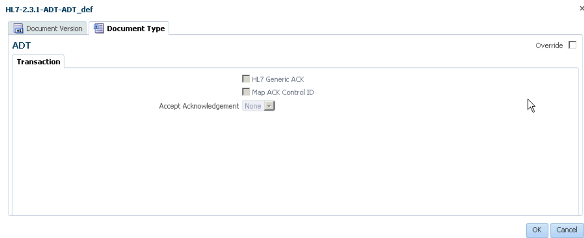
Figure 4-11 Overriding Document Type Parameters
