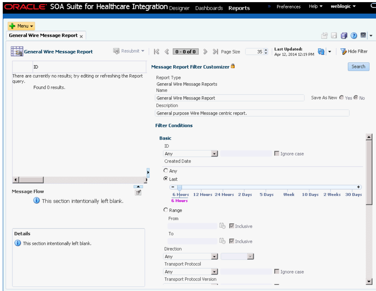
Figure 9-9 Wire Message Report Filter Customizer
