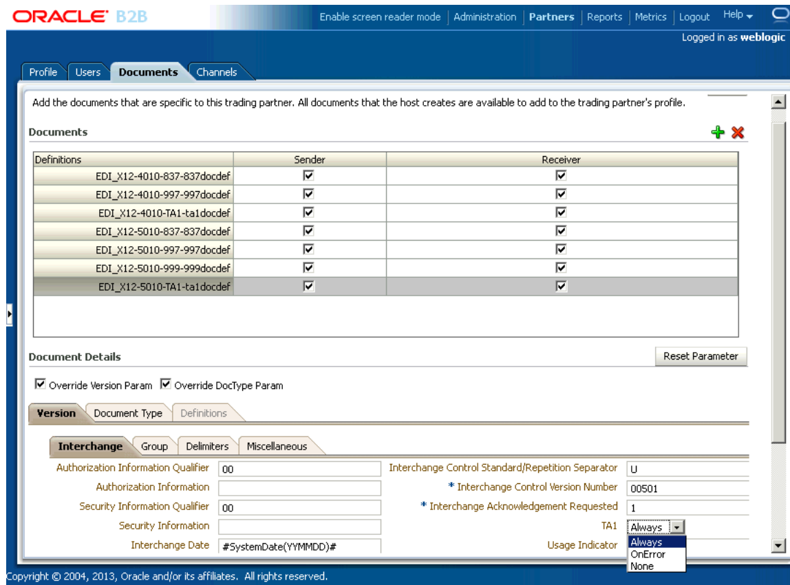
Figure I-5 Configuring TA1 at the Trading Partner Level
