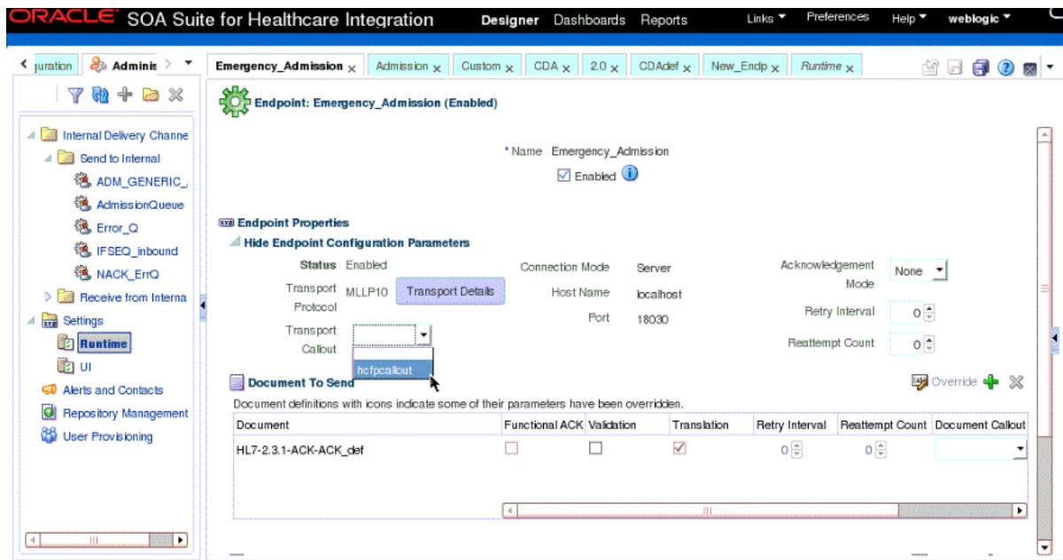
Figure 5-2 Transport Callouts
