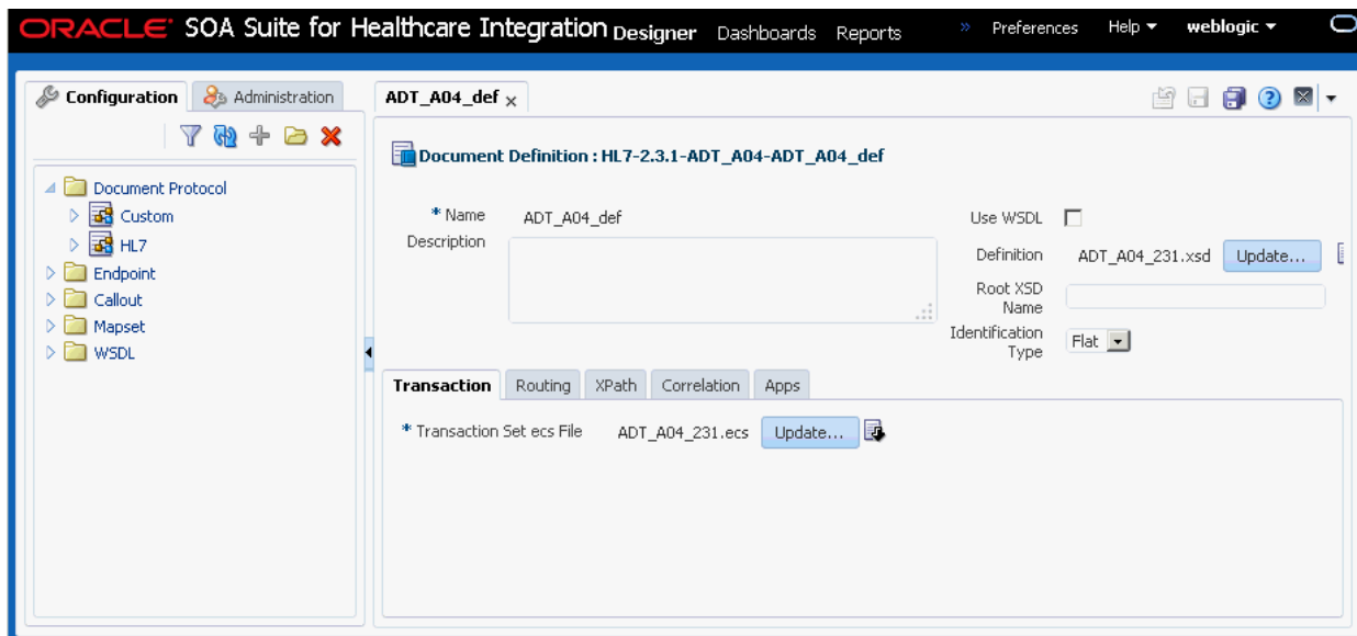
Figure 1-2 Designer Tab
