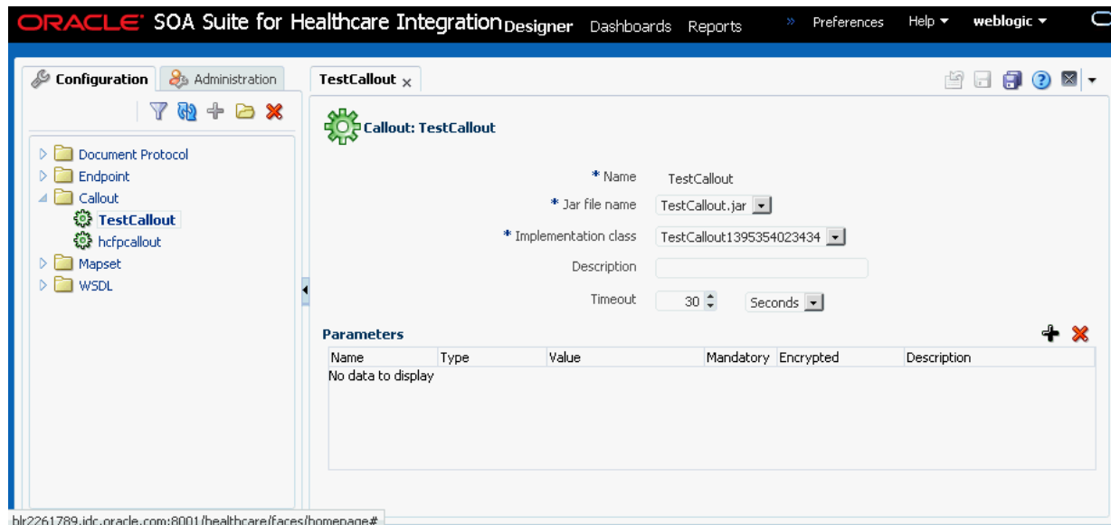
Figure 1-5 Sample Callout
