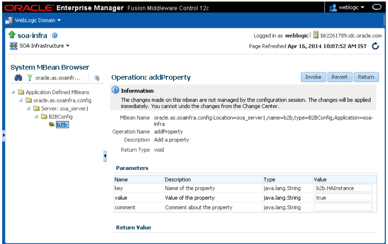
Figure F-3 Adding the b2b.HAInstance Property
