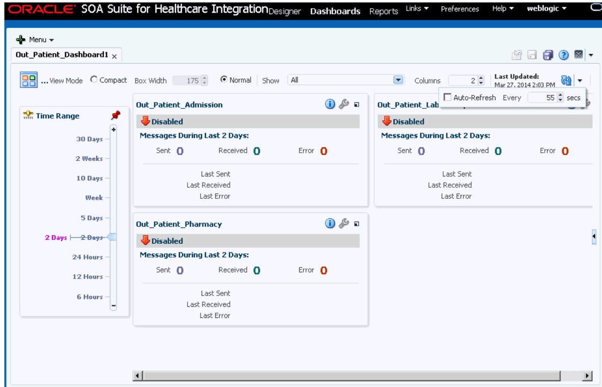
Figure 1-13 Sample Dashboard
