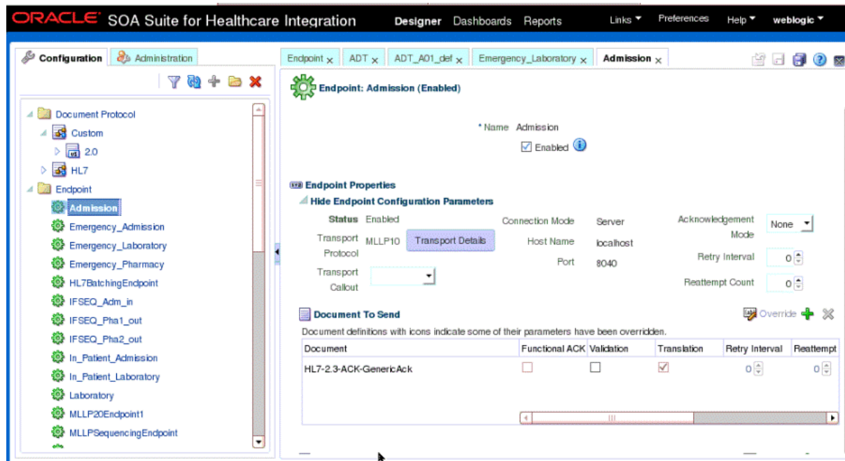
Figure 1-4 Sample Endpoint
