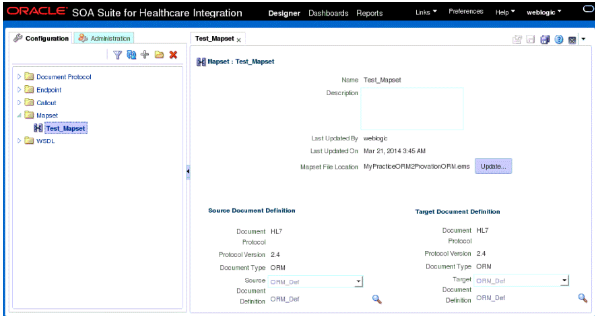
Figure 1-6 Sample Mapset
