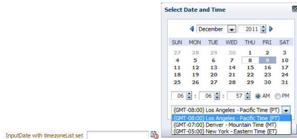
Figure 11-21 Custom Time Zone List in inputDate Component
