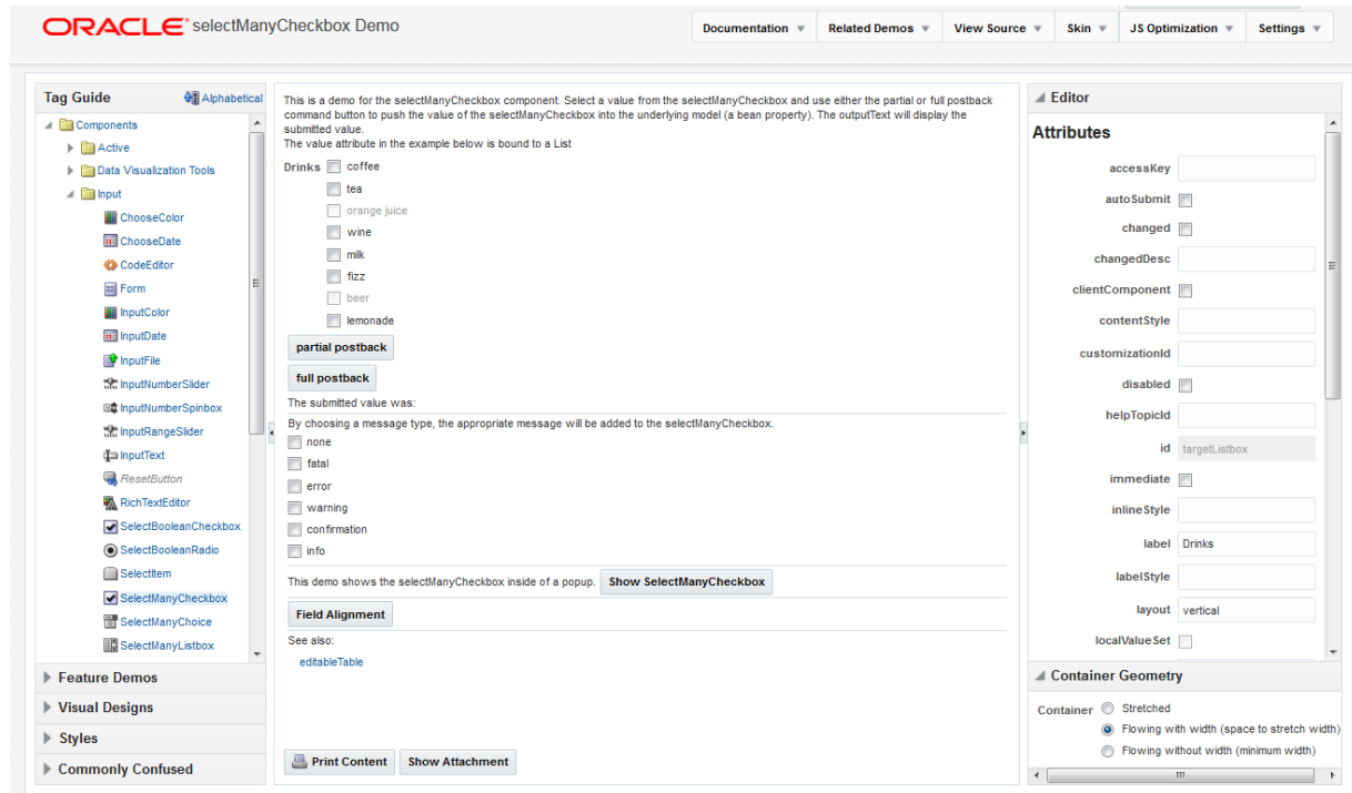
Figure 2-1 Tag Demonstration
