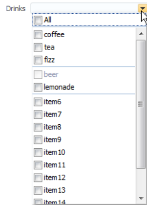
Figure 11-33 selectManyChoice Component
