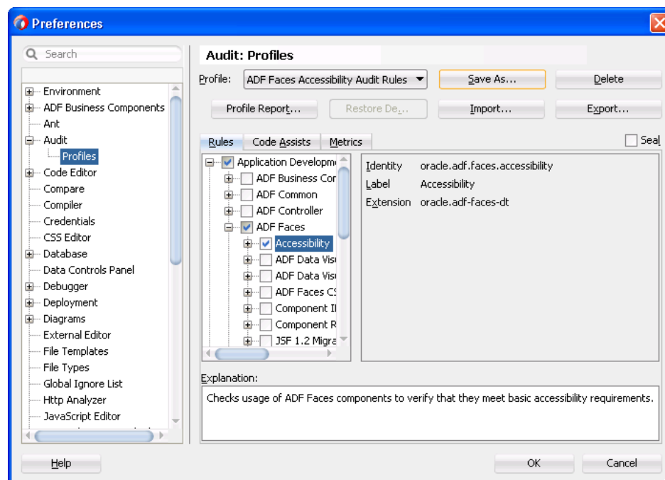
Figure 37-5 Audit Profile Settings for ADF Faces Accessibility
