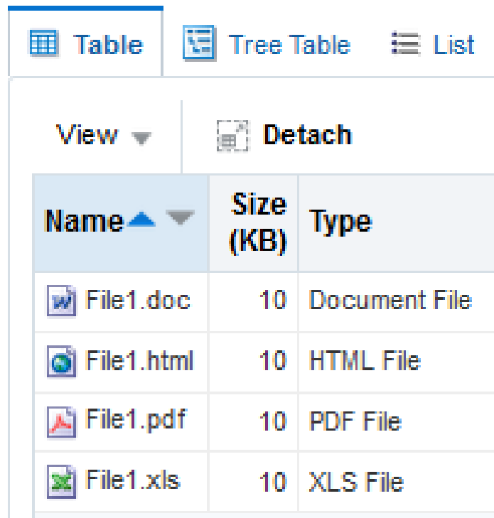
Figure 9-55 panelTabbed Panes
