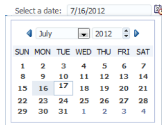
Figure 11-18 inputDate Component
