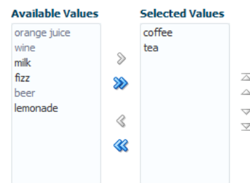
Figure 11-35 selectOrderShuttle Component
