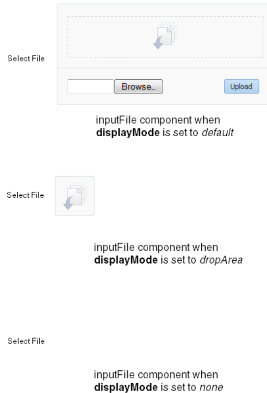
Figure 11-53 displayMode Attribute Values for inputFile Component
