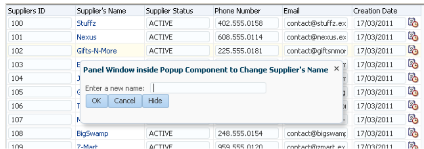
Figure 16-7 Popup Component Invoked by a Server-Side Method
