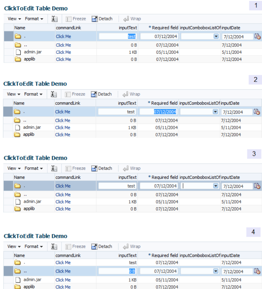
Figure C-2 Tab and Enter Keys Traversal Sequence in a Table
