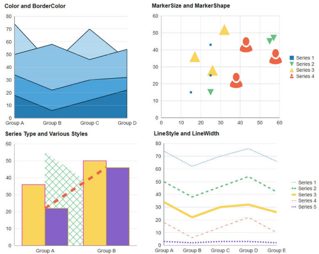
Figure 23-25 Chart Series Customization
