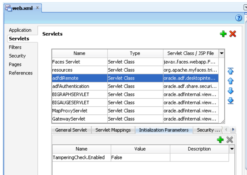
Figure 17-8 Disabling the Metadata Tamper Check In JDeveloper
