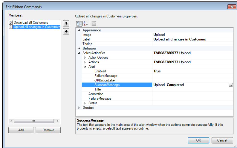
Figure 9-13 Alert Message Properties in an Action Set
