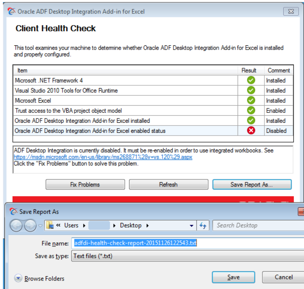
Figure H-3 Client Health Check Tool
