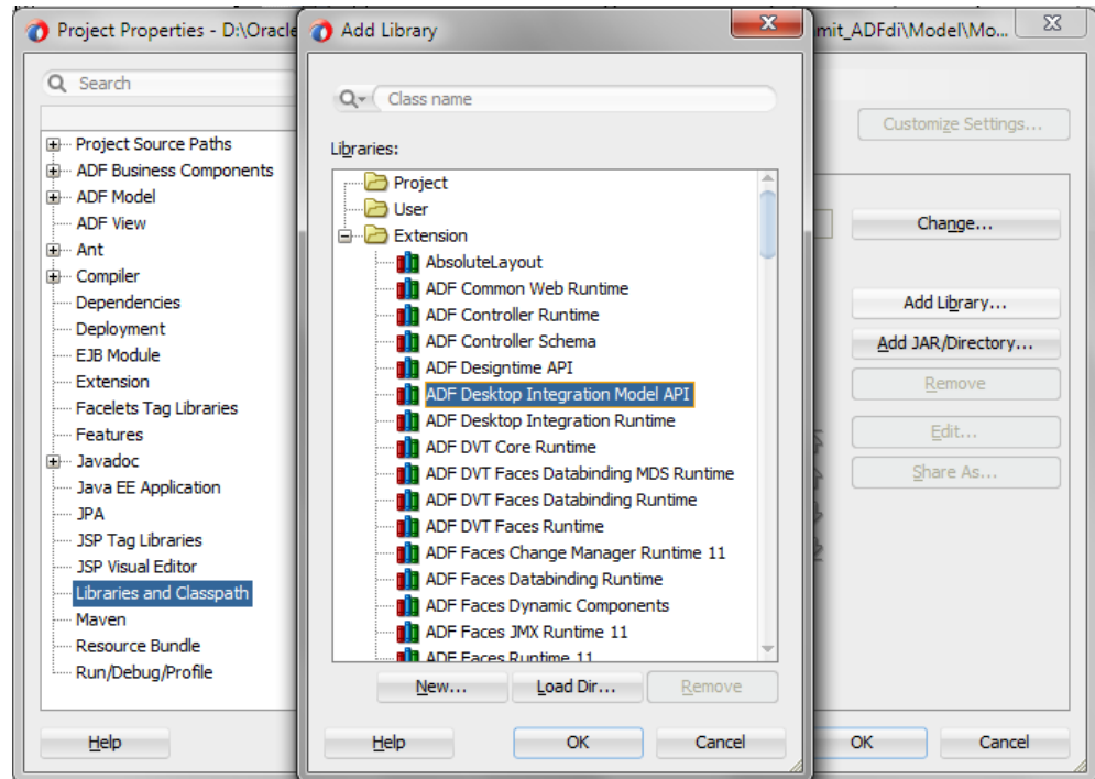
Figure G-1 Add Library Dialog
