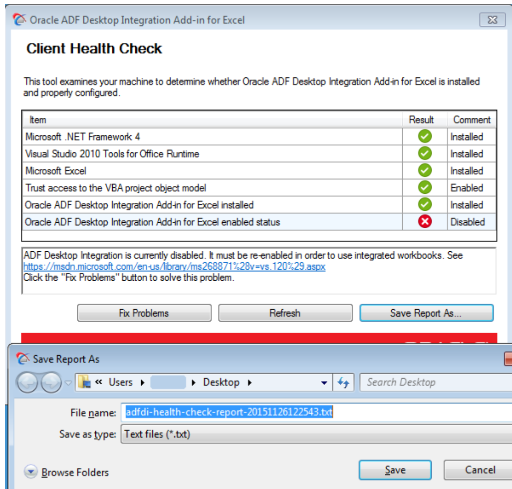
Figure 17-3 Client Health Check Tool
