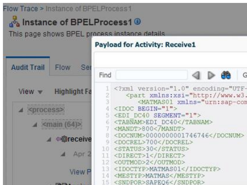
Figure 8-246 Audit Trail
