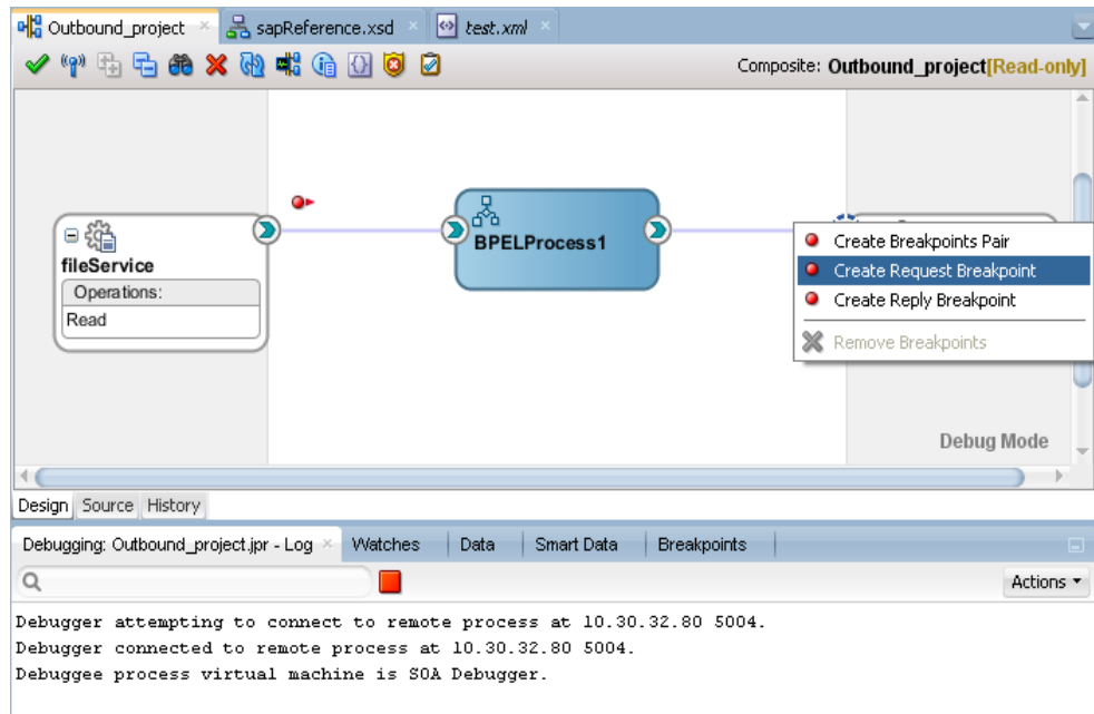
Figure 5-78 Breakpoint Options
