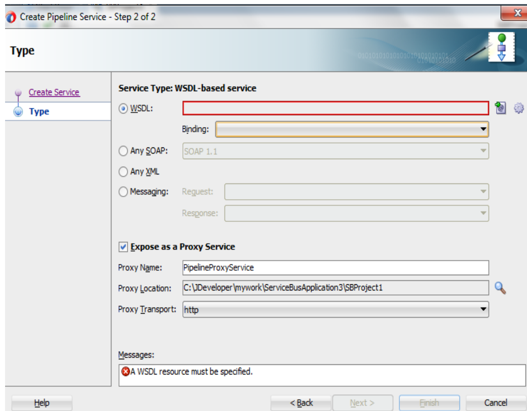
Figure 8-178 Type Page
