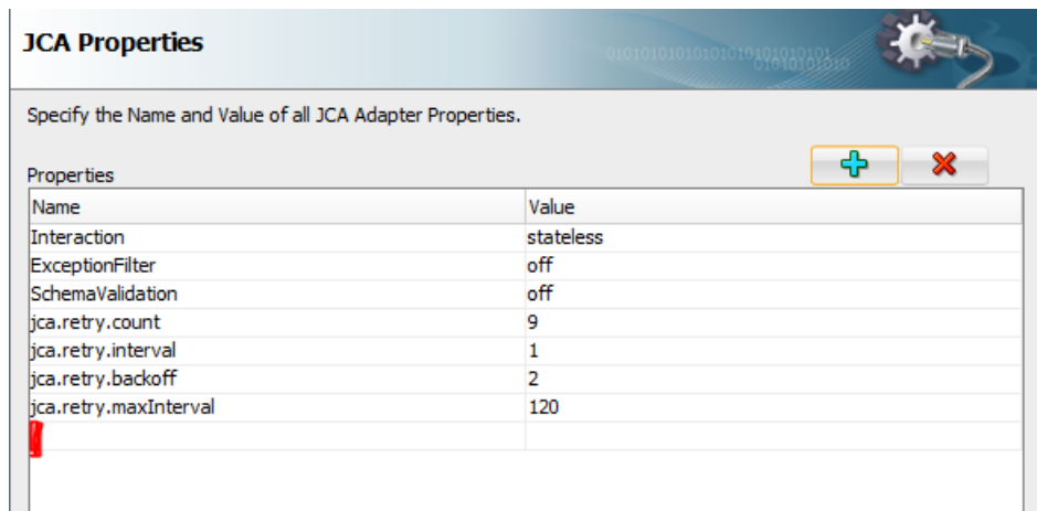
Figure 5-87 JCA Property
