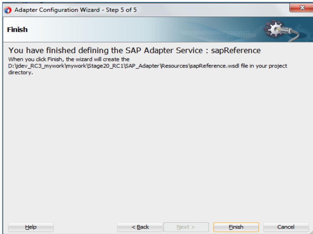
Figure 6-34 Finish Page
