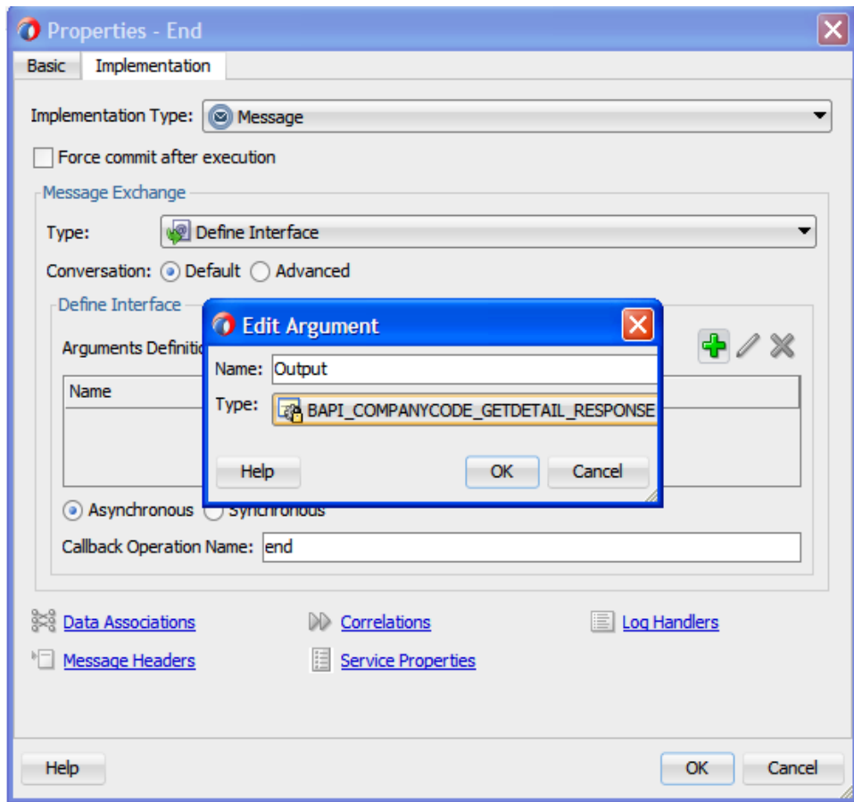
Figure 8-141 Implementation Tab
