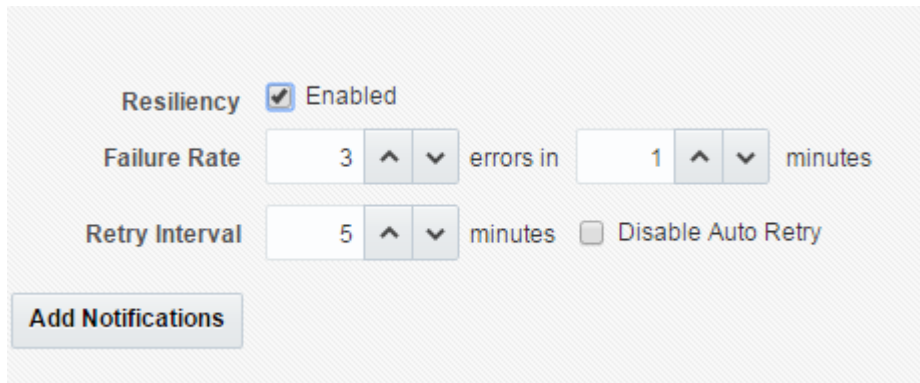
Figure 5-115 Resiliency Configuration
