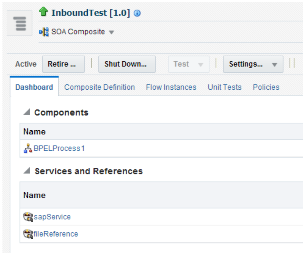
Figure 8-245 Instances Tab
