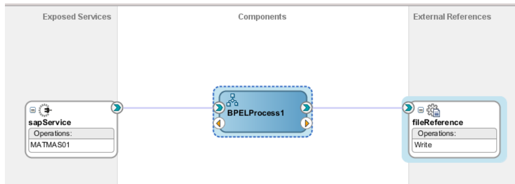
Figure 5-90 JCA Property
