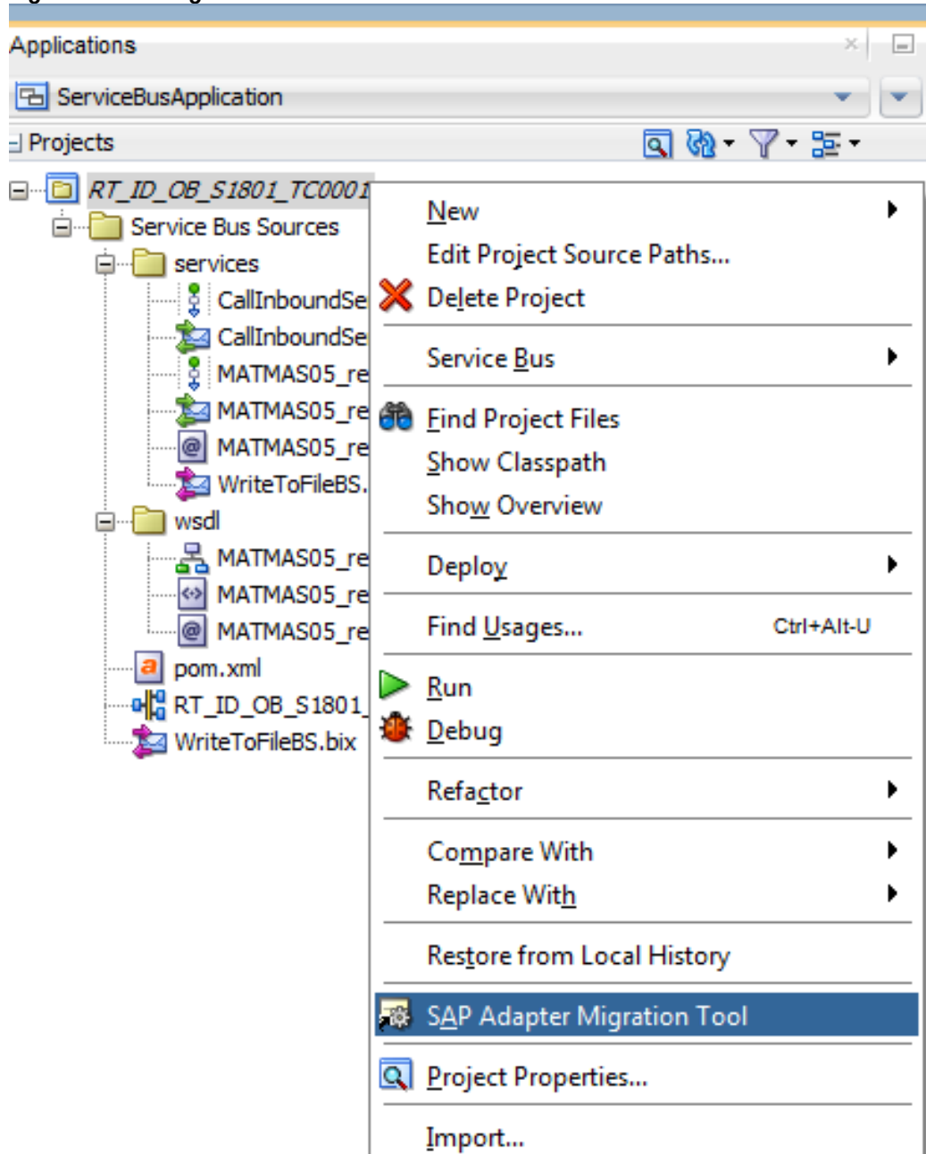
Figure 12-13 Migration Tool
