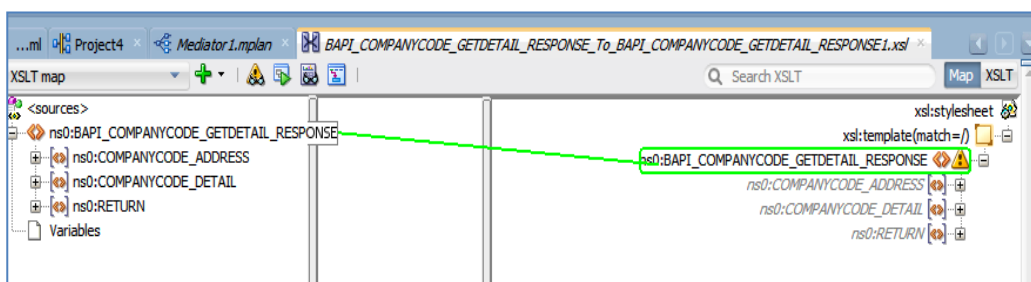
Figure 8-85 Mapping Page
