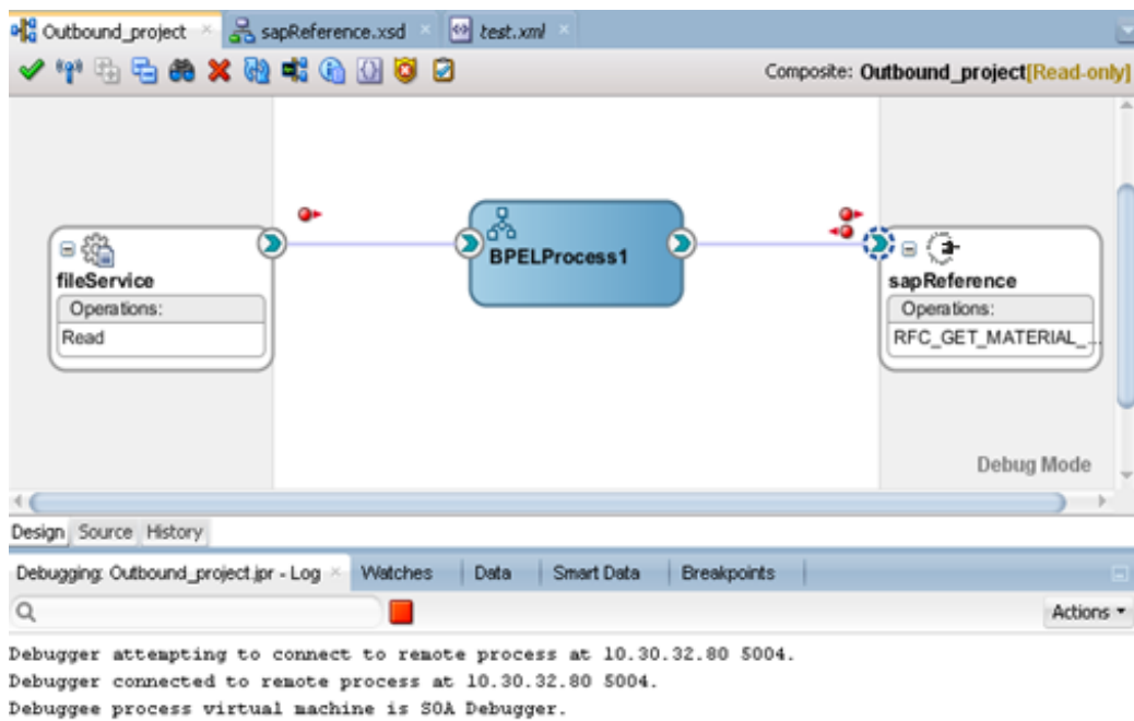
Figure 5-79 Breakpoint Options
