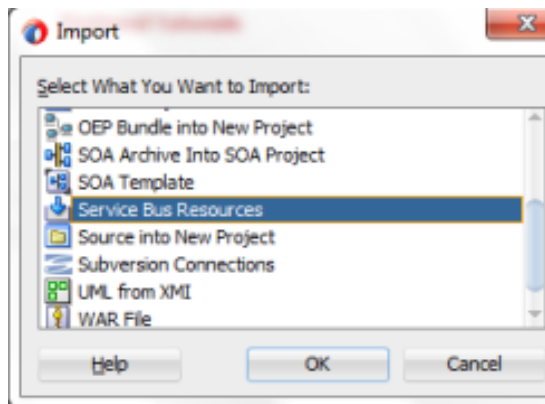
Figure 12-9 Import Window
