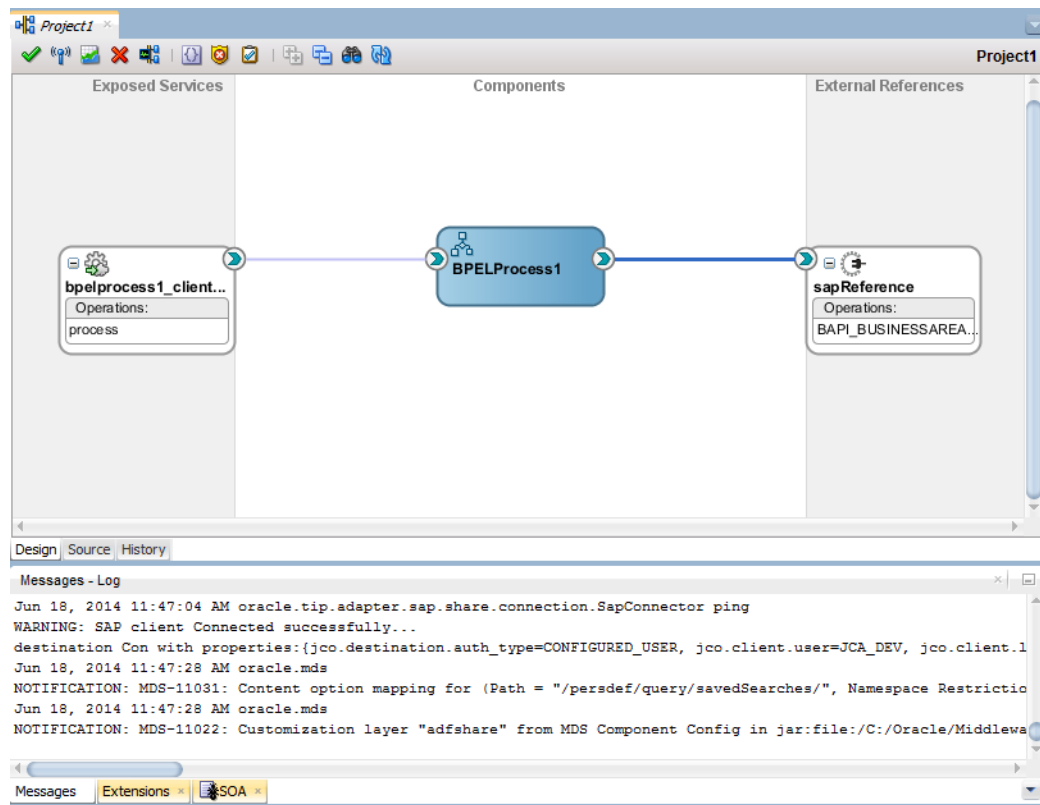
Figure 2-10 Outbound Composite
