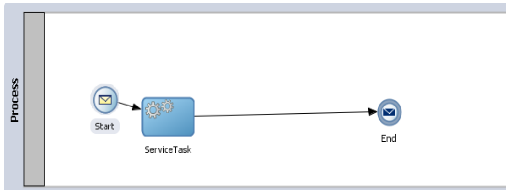
Figure 8-127 Service Task
