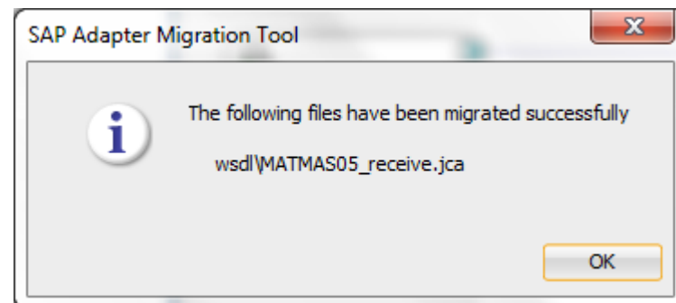
Figure 12-16 Confirmaion Window
