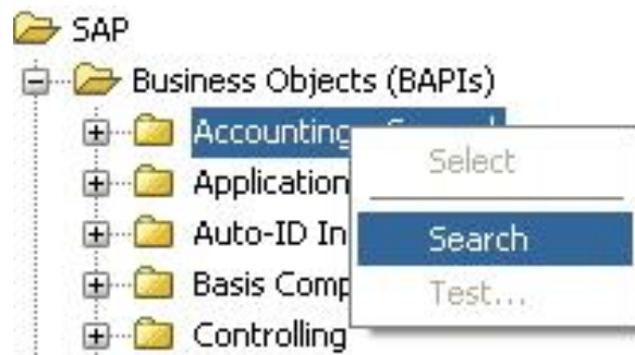
Figure 6-24 Search Option
