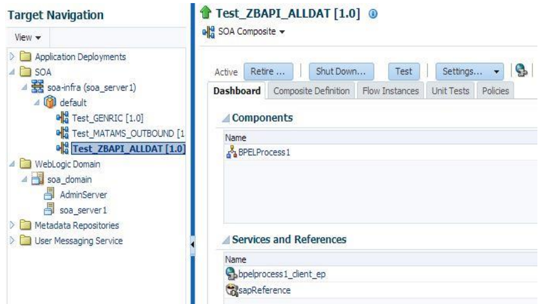
Figure 5-56 Target Navigation
