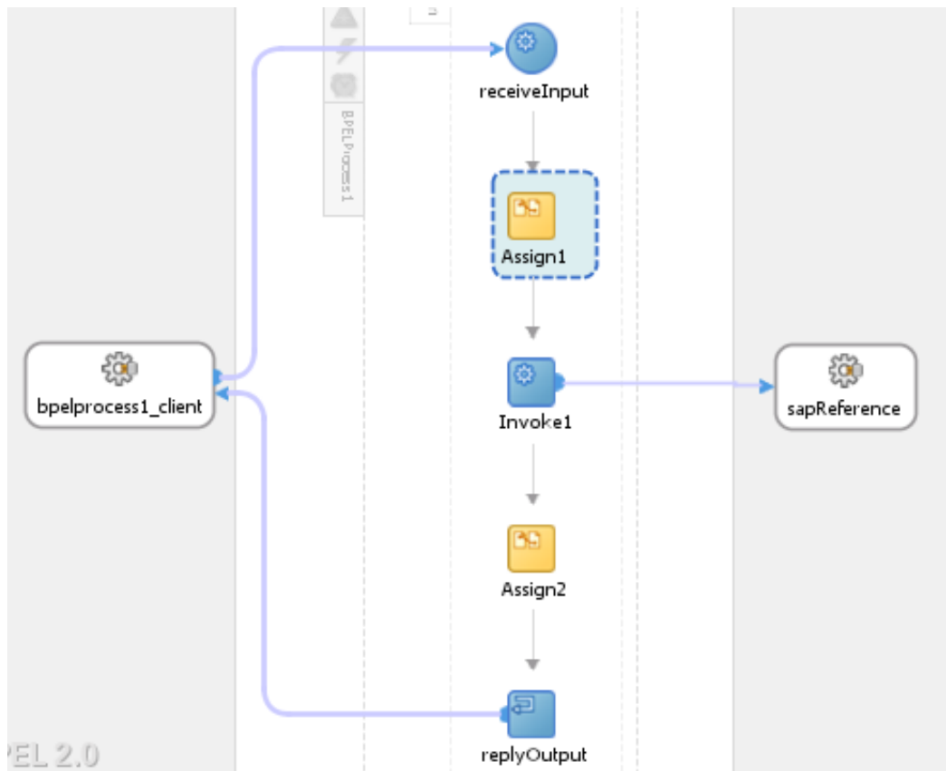
Figure 8-46 Composite.xml
