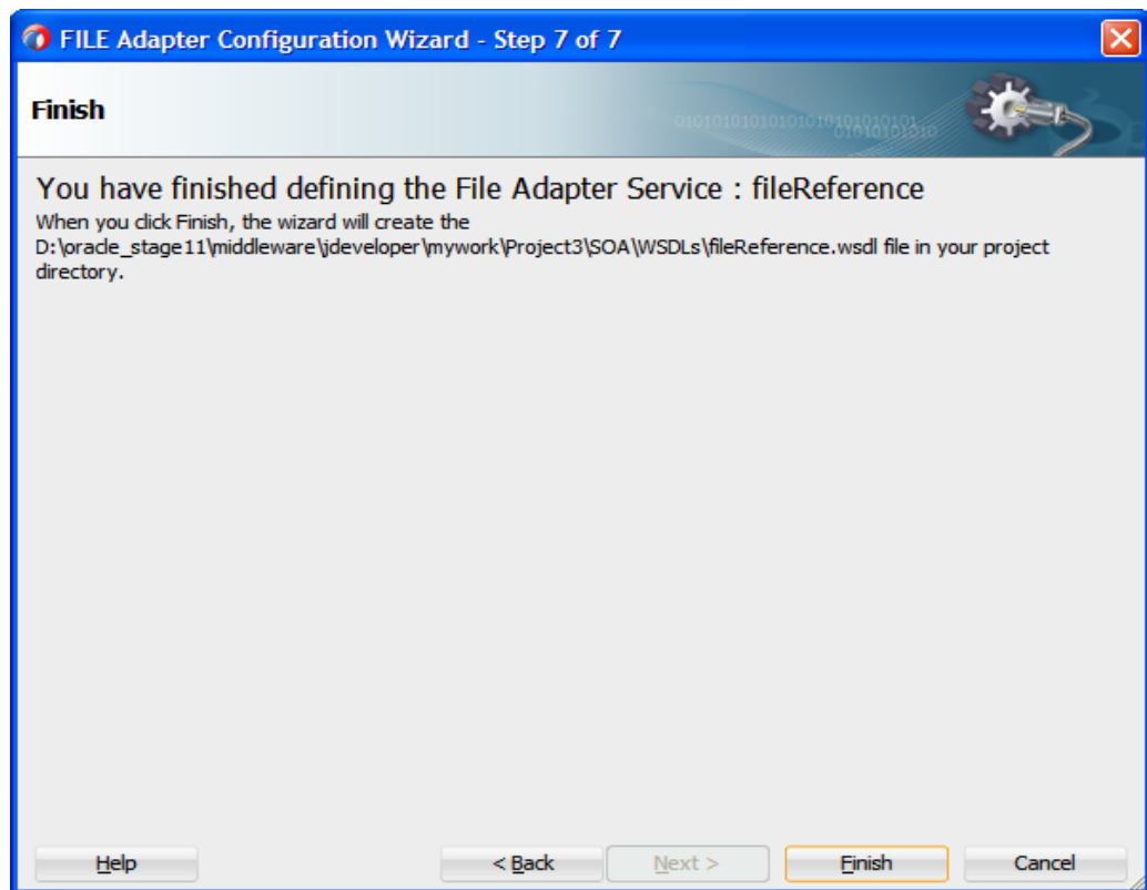
Figure 8-98 Finish Page
