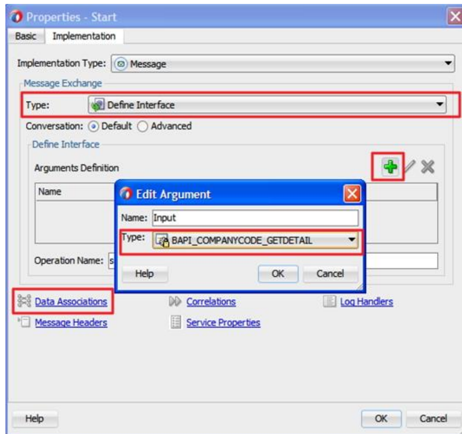
Figure 8-128 Properties-Start Dialog
