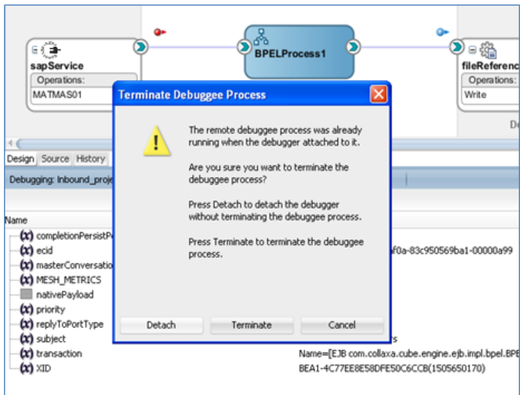
Figure 5-74 Detach Debugger
