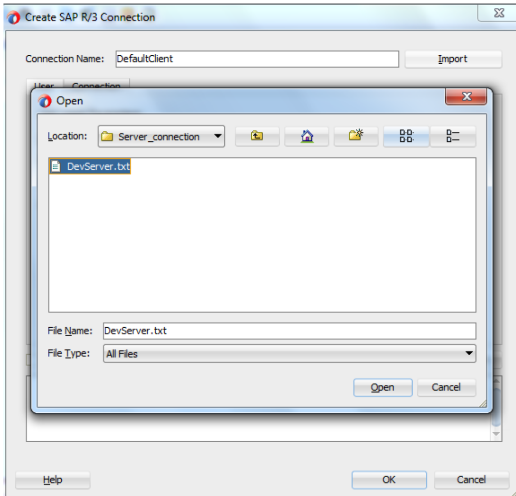
Figure 6-8 Import Button
