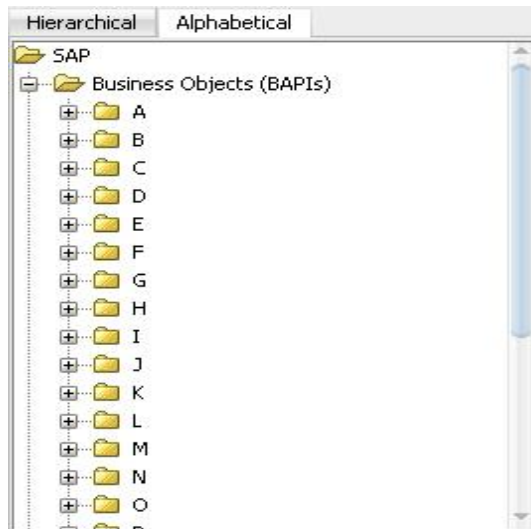
Figure 6-22 Alphabetical Tab
