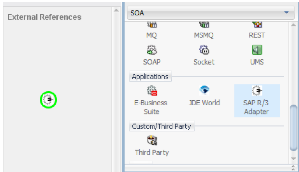
Figure 2-9 Adapter Component
