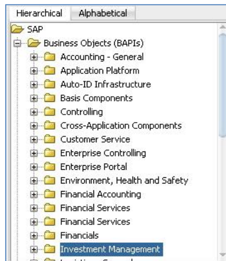
Figure 8-198 Hierarchical Tab
