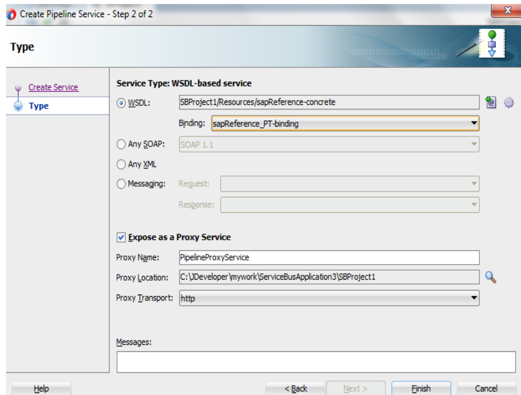
Figure 8-180 Type Page
