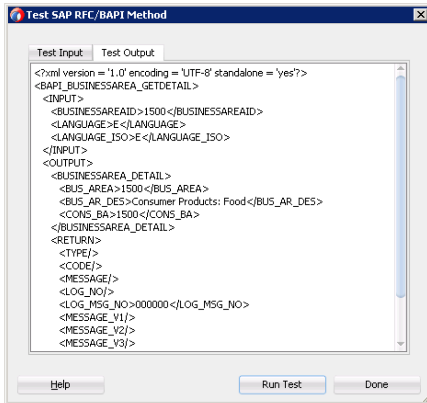
Figure 5-24 Test Output
