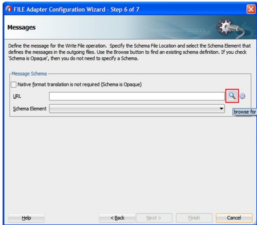
Figure 8-95 Messages Page
