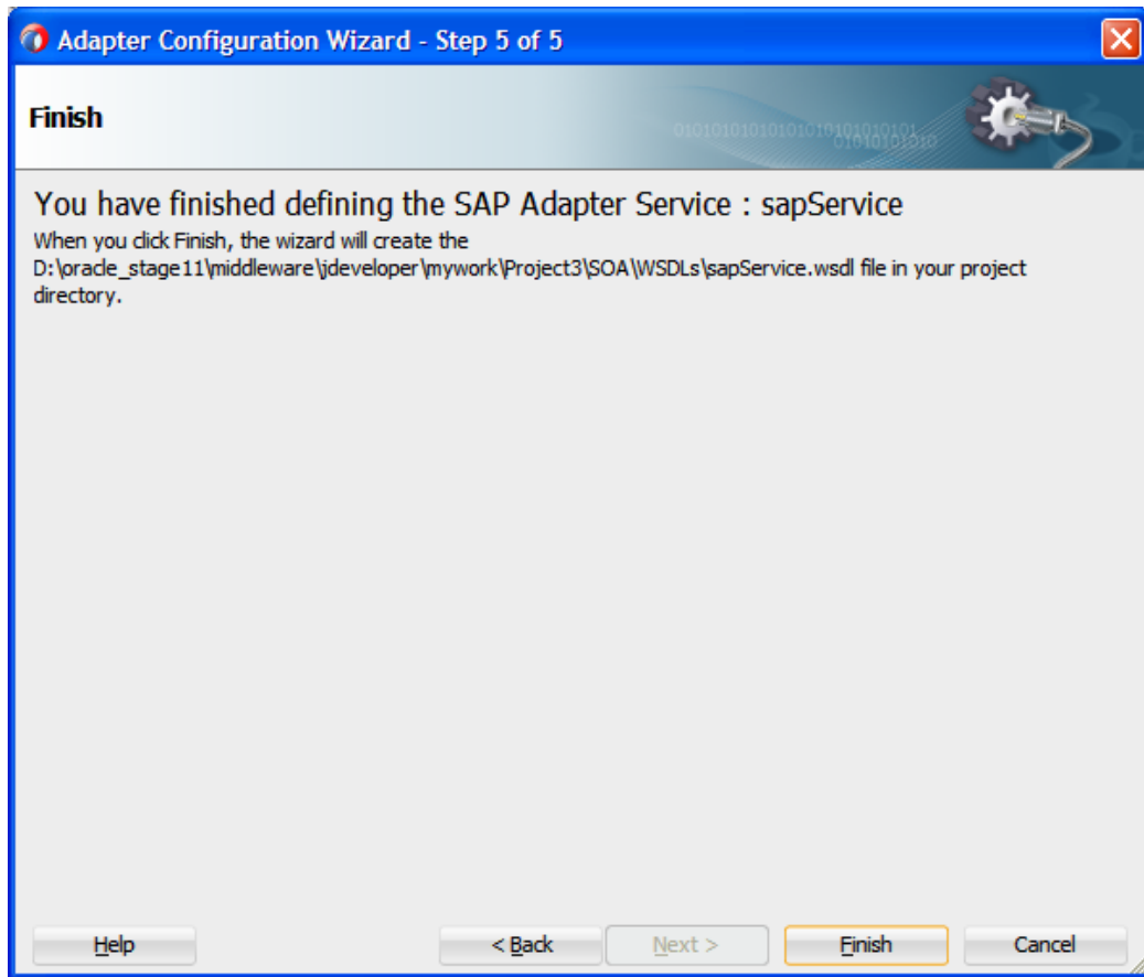
Figure 8-62 Finish Page
