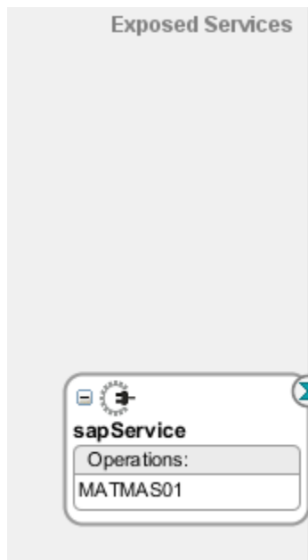
Figure 8-63 Adapter Component
