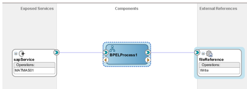
Figure 5-112 Design of Composite
