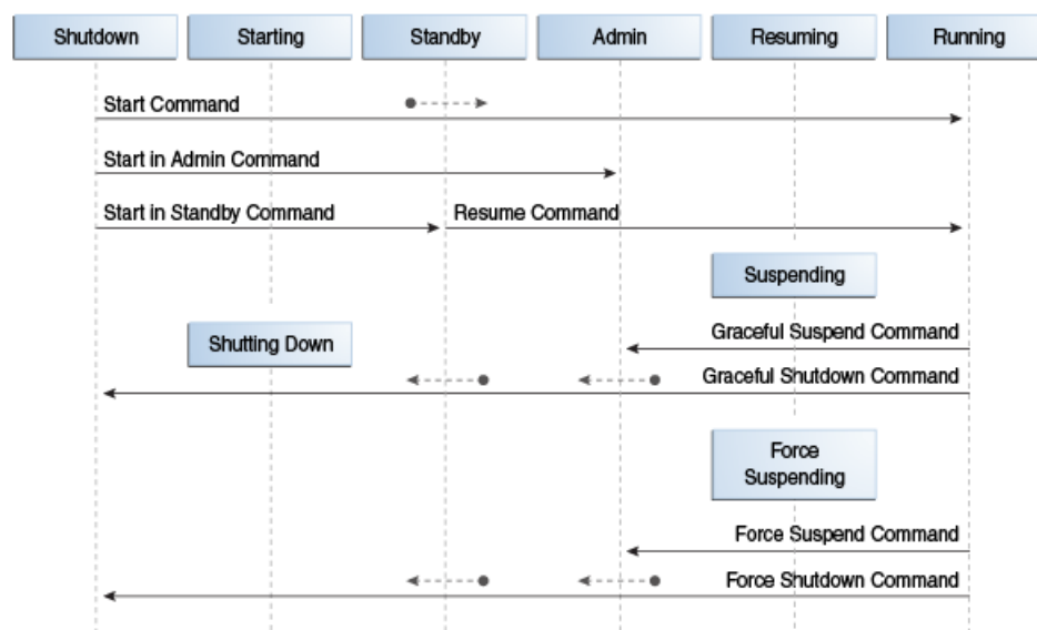
Figure 5–1 State Transitions for Server Life Cycle Commands
