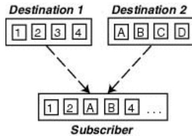
Figure 9–2 Multicasting Sequence Gap
