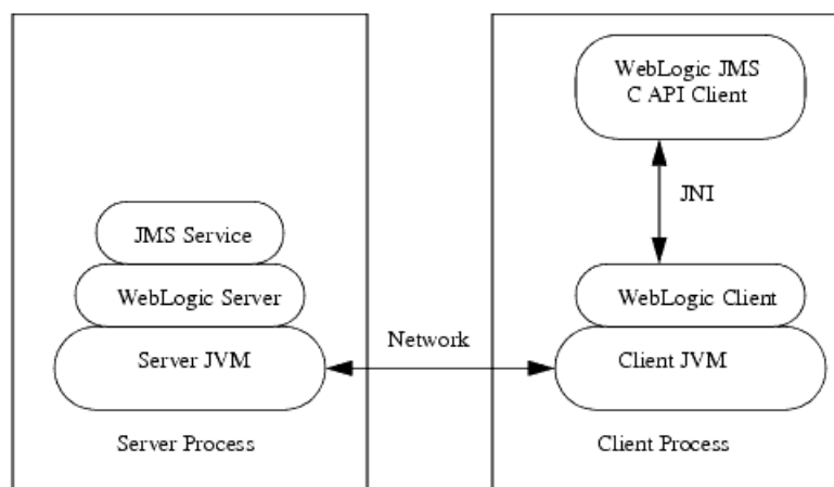
Figure 16-1 WebLogic JMS C API Client Application Environment
