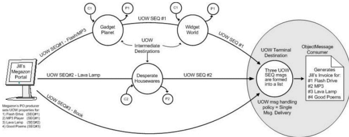
Figure 12–1 Workflow for Jill's Order Using Unit-of-Work
