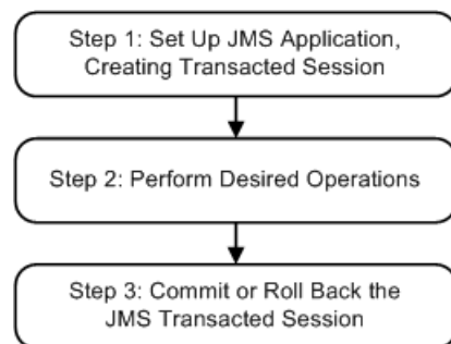
Figure 13–1 Setting Up and Using a JMS Transacted Session
