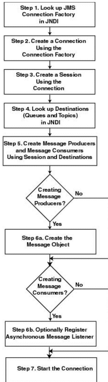
Figure 6–2 Setting Up a JMS Application using Classic API
