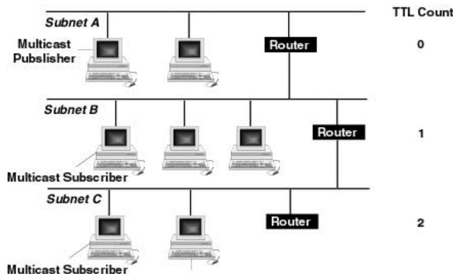
Figure 9–3 Multicast TTL Example
