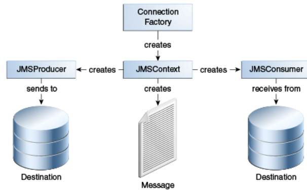
Figure 5–1 Simplified API Programming Model
