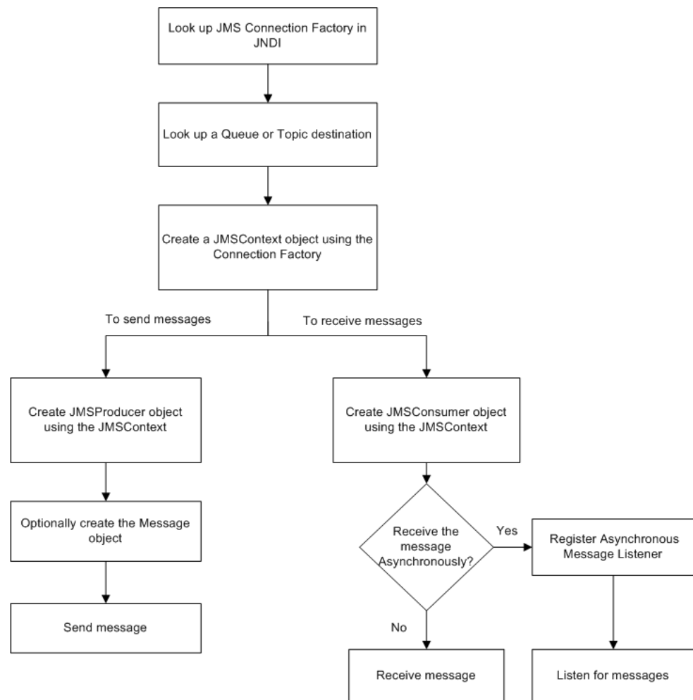
Figure 6–1 Setting up a JMS Application Using the Simplified API
