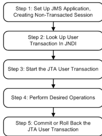
Figure 13–2 Setting Up and Using a JTA User Transaction
