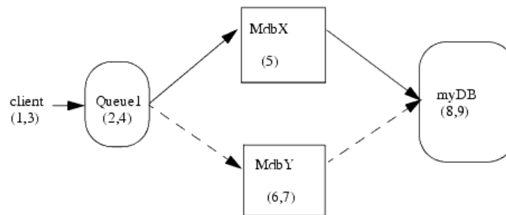
Figure 11–2 Workflow for Joe's Order Using Unit-of-Order
