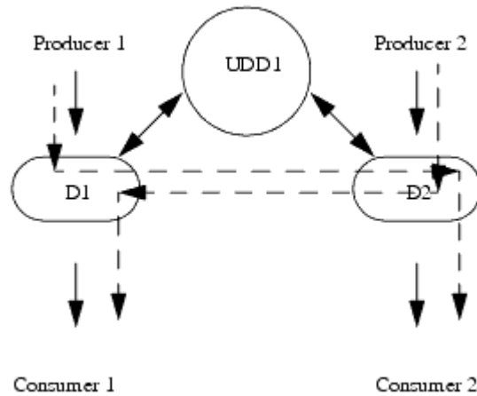
Figure 10–2 Using Distributed Topics
