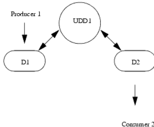
Figure 10–3 Stuck Messages
