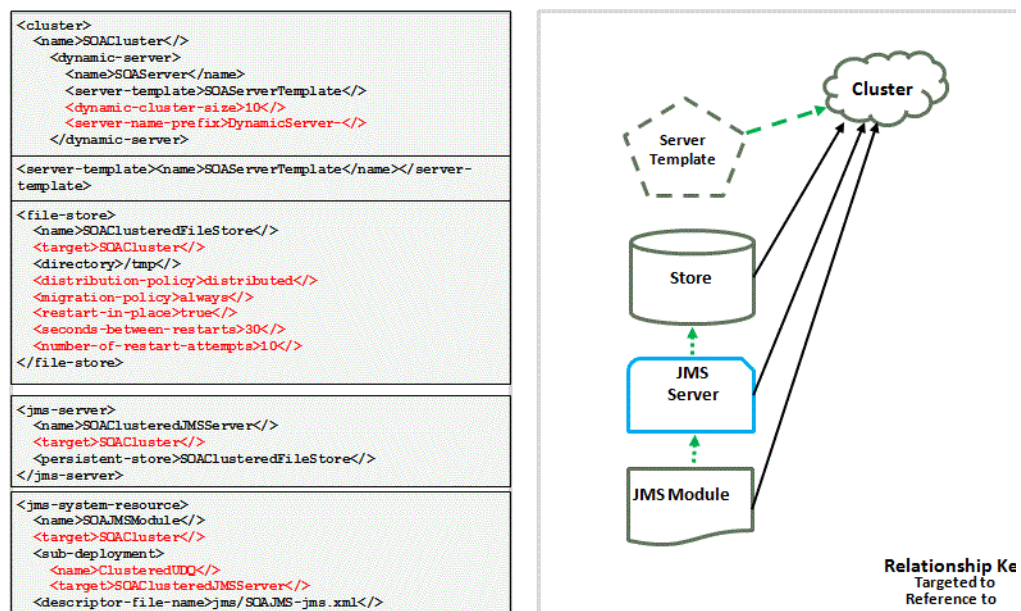
Figure 5–1 Dynamic Clustered JMS
